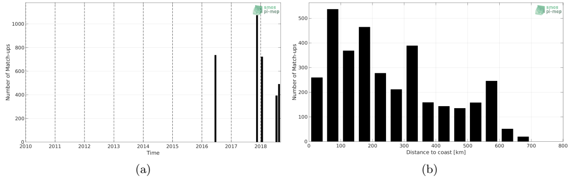
Figure 1: Number of match-ups between TSG-LEGOS-DM and SMOS-L3-CATDS-CPDC-V317-10DAYS-25KM SSS as a function of time (a) and as function of the distance to coast (b) over the Congo river plume Pi-MEP region and for the full satellite product period.
