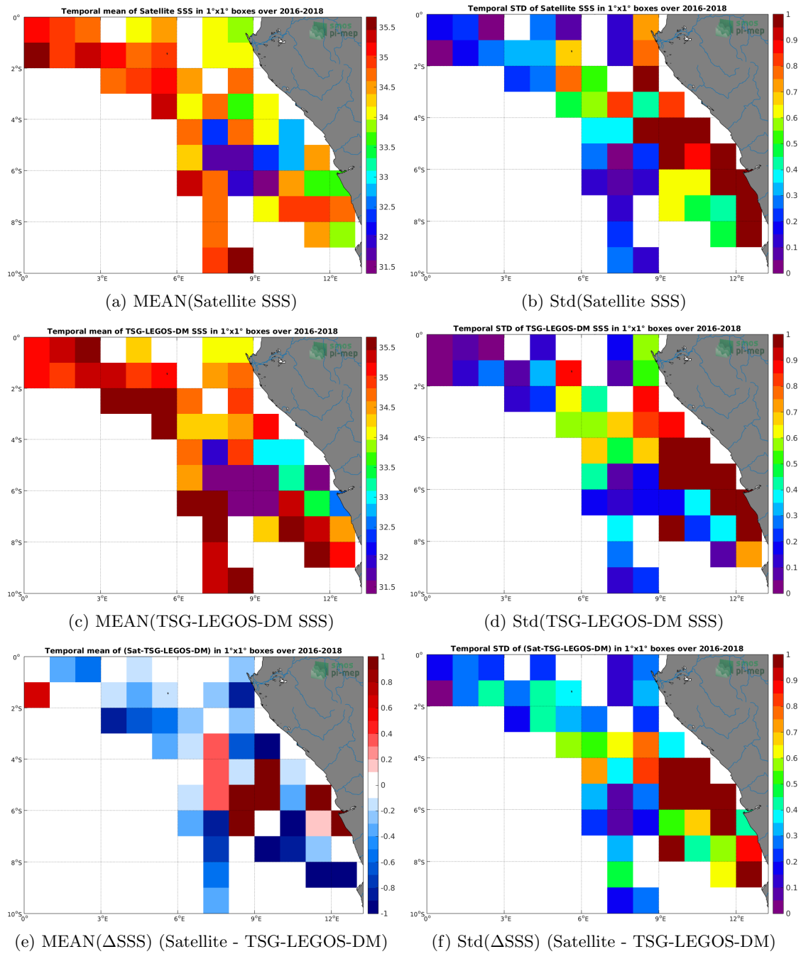
Figure 6: Temporal mean (left) and Std (right) of SSS from SMOS-L3-CATDS-CPDC-V317-10DAYS-25KM (top), TSG-LEGOS-DM (middle), and of \Delta SSS (Satellite - TSG-LEGOS-DM). Only match-up pairs are used to generate these maps.
