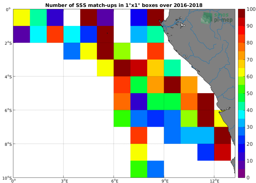
Figure 4: Number of SSS match-ups between TSG-LEGOS-DM SSS and the SMOS-L3-CATDS-CPDC-V317-10DAYS-25KM SSS product for the Congo river plume Pi-MEP region over 1^\circ \times 1^\circ boxes and for the full satellite product period.
