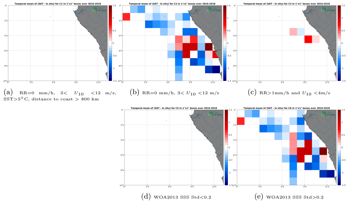
Figure 12: Temporal mean gridded over spatial boxes of size 1^\circ \times 1^\circ of \Delta SSS (SMOS-L3-CATDS-CPDC-V317-10DAYS-25KM - TSG-LEGOS-DM) for 5 different subdatasets corresponding to:RR=0 mm/h, 3 < U_{10} < 12 m/s, SST >5^\circ C, distance to coast > 800 km (a), RR=0 mm/h, 3 < U_{10} < 12 m/s (b), RR >1 mm/h and U_{10} < 4 m/s (c), WOA2013 SSS Std <0.2 (d), WOA2013 SSS Std >0.2 (e).
