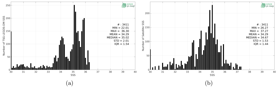
Figure 2: Histograms of SSS from TSG-LEGOS-DM (a) and SMOS-L3-CATDS-CPDC-V317-10DAYS-25KM (b) considering all match-up pairs per bins of 0.1 over the Congo river plume Pi-MEP region and for the full satellite product period.
