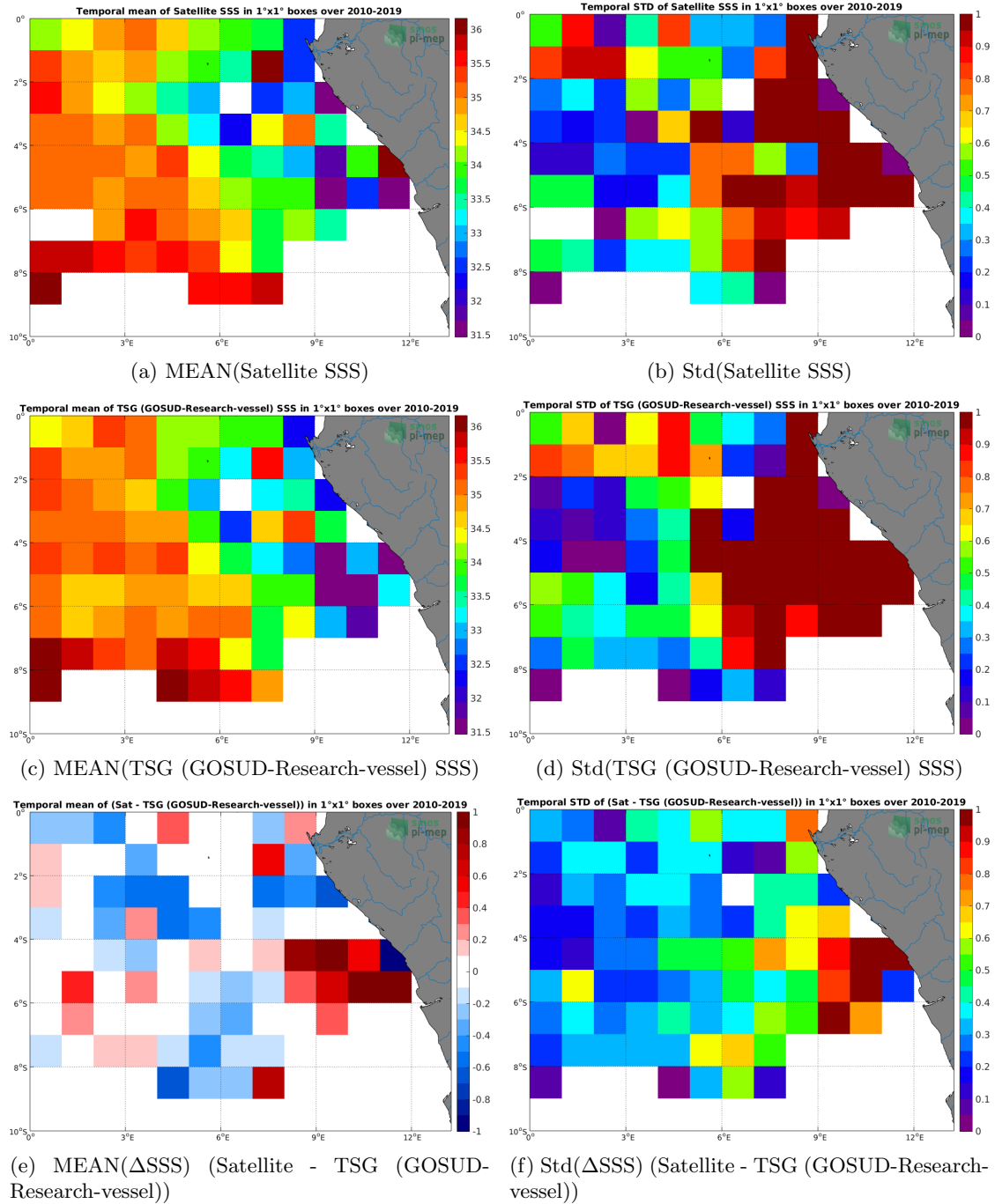
Figure 6: Temporal mean (left) and Std (right) of SSS from SMOS SSS L3 v317 - 10 Days - 25 km (CATDS-CPDC) (top), TSG (GOSUD-Research-vessel) (middle), and of \Delta SSS (Satellite - TSG (GOSUD-Research-vessel)). Only match-up pairs are used to generate these maps.
