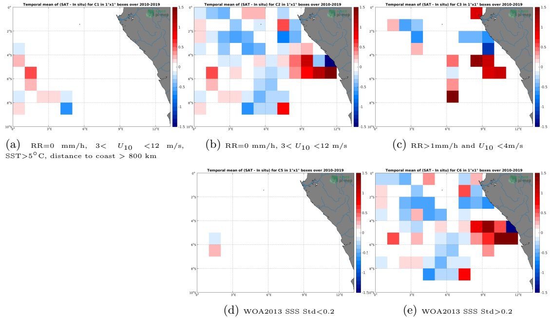
Figure 12: Temporal mean gridded over spatial boxes of size 1^\circ \times 1^\circ of \Delta SSS (SMOS SSS L3 v317 - 10 Days - 25 km (CATDS-CPDC) - TSG (GOSUD-Research-vessel)) for 5 different subdatasets corresponding to: RR=0 mm/h, 3 < U_{10} < 12 m/s, SST > 5^\circ\text{C} , distance to coast > 800 km (a), RR=0 mm/h, 3 < U_{10} < 12 m/s (b), RR > 1 mm/h and U_{10} < 4 m/s (c), WOA2013 SSS Std < 0.2 (d), WOA2013 SSS Std > 0.2 (e).
