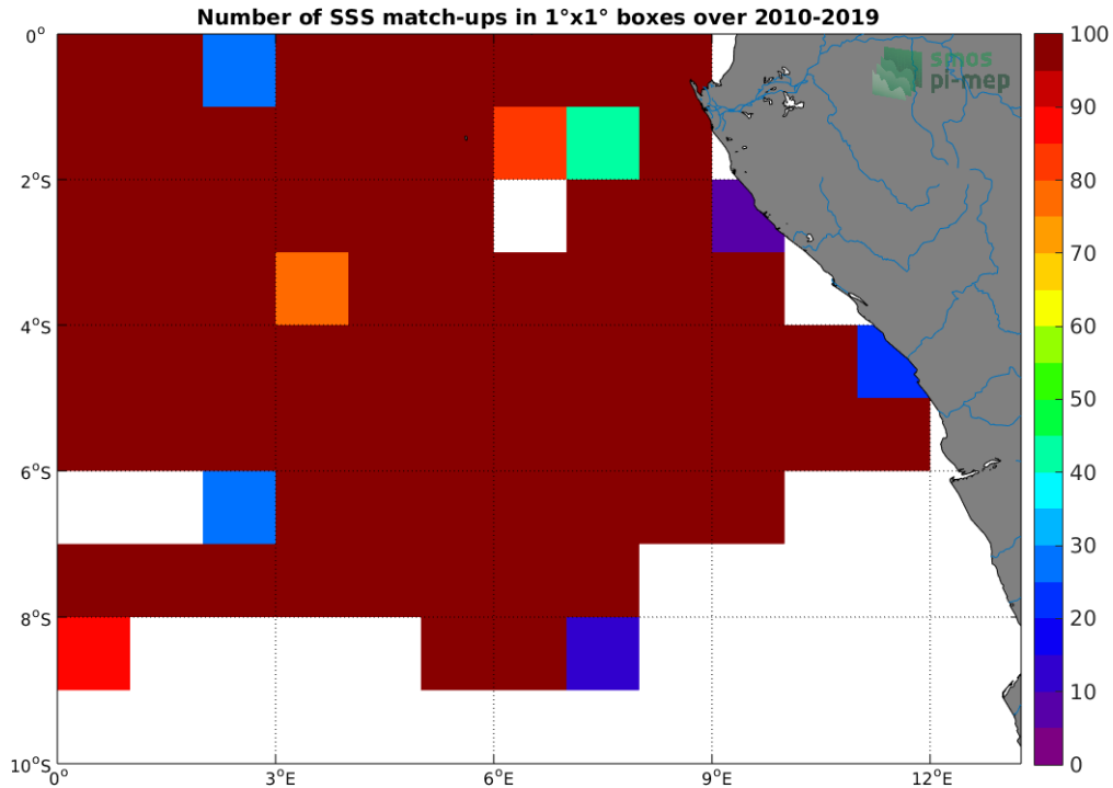
Figure 4: Number of SSS match-ups between TSG (GOSUD-Research-vessel) SSS and the SMOS SSS L3 v317 - 10 Days - 25 km (CATDS-CPDC) SSS product for the Congo river plume Pi-MEP region over 1°x1° boxes and for the full satellite product period.
