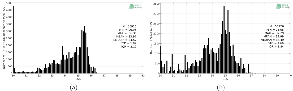
Figure 2: Histograms of SSS from TSG (GOSUD-Research-vessel) (a) and SMOS SSS L3 v317 - 10 Days - 25 km (CATDS-CPDC) (b) considering all match-up pairs per bins of 0.1 over the Congo river plume Pi-MEP region and for the full satellite product period.
