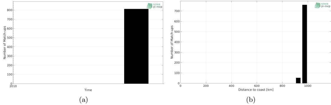
Figure 1: Number of match-ups between TSG-SAMOS and SMOS-L3-CATDS-CPDC-V3-MONTHLY-25KM SSS as a function of time (a) and as function of the distance to coast (b) over the Congo river plume Pi-MEP region and for the full satellite product period.
