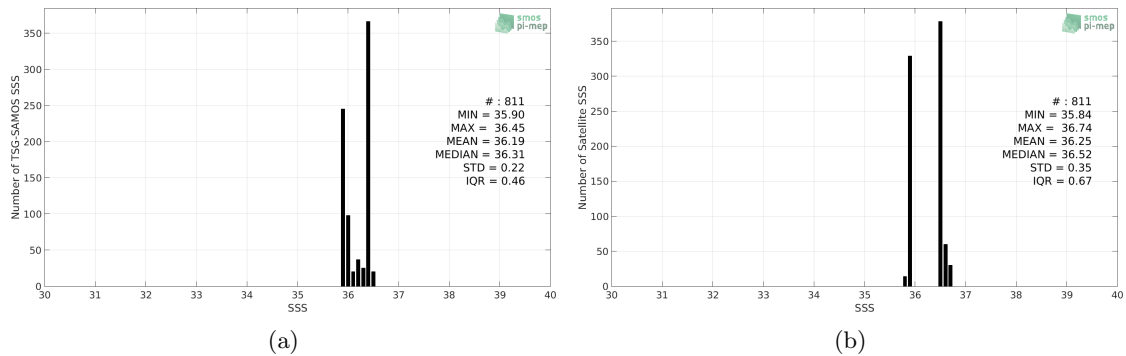
Figure 2: Histograms of SSS from TSG-SAMOS (a) and SMOS-L3-CATDS-CPDC-V3-MONTHLY-25KM (b) considering all match-up pairs per bins of 0.1 over the Congo river plume Pi-MEP region and for the full satellite product period.
