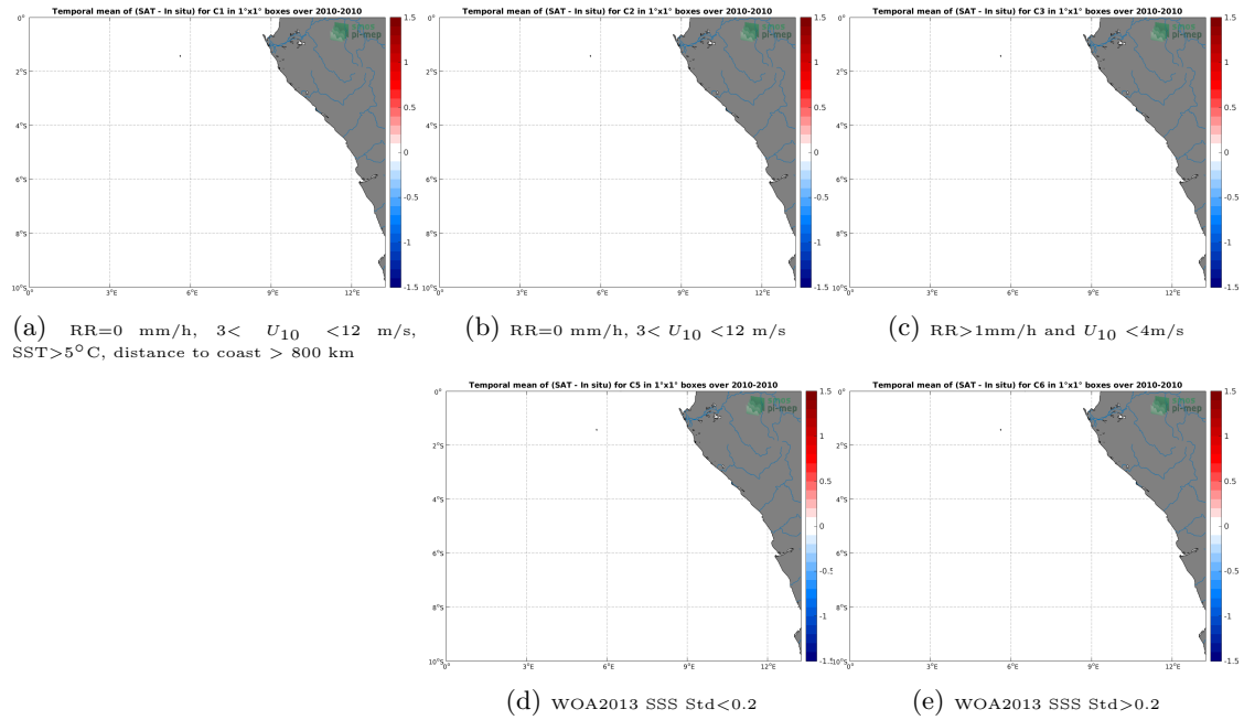
Figure 12: Temporal mean gridded over spatial boxes of size 1^\circ \times 1^\circ of \Delta SSS (SMOS-L3-CATDS-CPDC-V3-MONTHLY-25KM - TSG-SAMOS) for 5 different subdatasets corresponding to:RR=0 mm/h, 3 < U_{10} < 12 m/s, SST >5^\circ\text{C} , distance to coast > 800 km (a), RR=0 mm/h, 3 < U_{10} < 12 m/s (b), RR >1 mm/h and U_{10} < 4 m/s (c), WOA2013 SSS Std <0.2 (d), WOA2013 SSS Std >0.2 (e).
