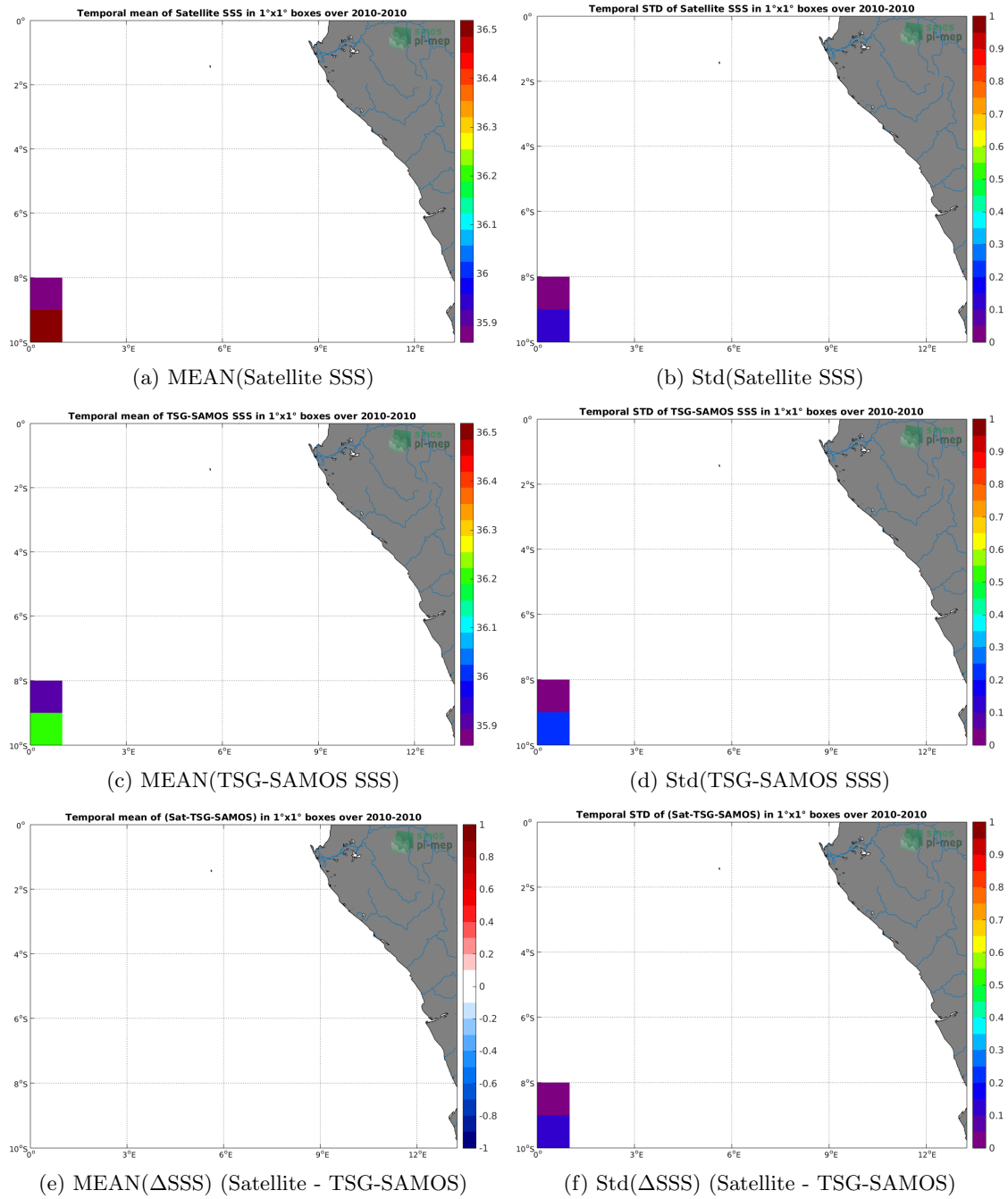
Figure 6: Temporal mean (left) and Std (right) of SSS from SMOS-L3-CATDS-CPDC-V3-MONTHLY-25KM (top), TSG-SAMOS (middle), and of \Delta SSS (Satellite - TSG-SAMOS). Only match-up pairs are used to generate these maps.
