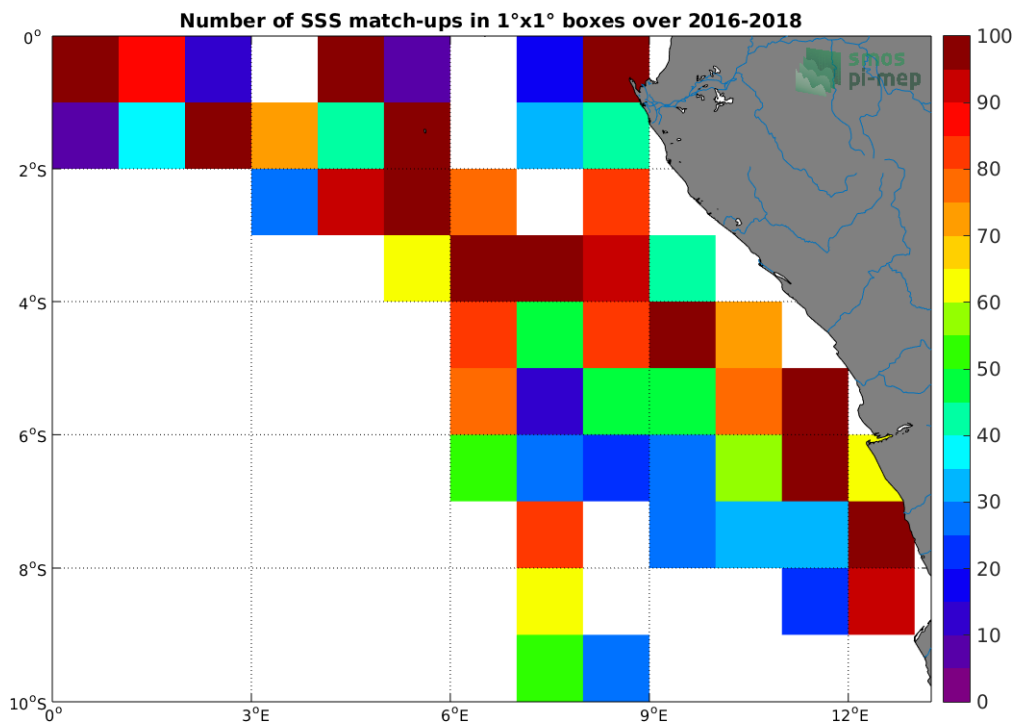
Figure 4: Number of SSS match-ups between TSG-LEGOS-DM SSS and the SMOS-L3-CATDS-CPDC-V3-MONTHLY-25KM SSS product for the Congo river plume Pi-MEP region over 1^\circ \times 1^\circ boxes and for the full satellite product period.
