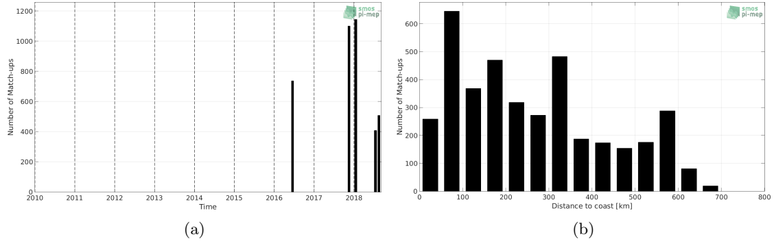
Figure 1: Number of match-ups between TSG-LEGOS-DM and SMOS-L3-CATDS-CPDC-V3-MONTHLY-25KM SSS as a function of time (a) and as function of the distance to coast (b) over the Congo river plume Pi-MEP region and for the full satellite product period.
