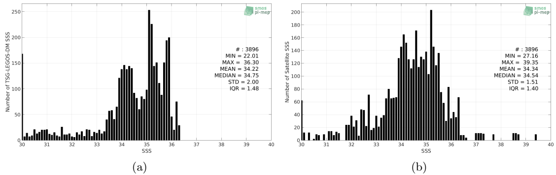
Figure 2: Histograms of SSS from TSG-LEGOS-DM (a) and SMOS-L3-CATDS-CPDC-V3-MONTHLY-25KM (b) considering all match-up pairs per bins of 0.1 over the Congo river plume Pi-MEP region and for the full satellite product period.
