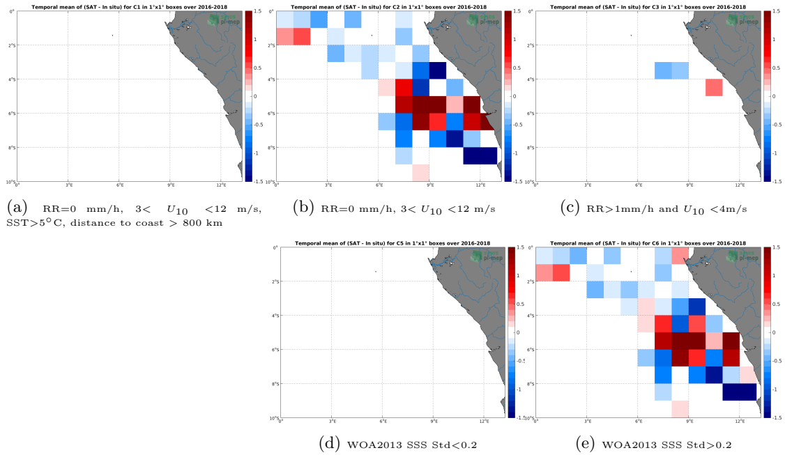
Figure 12: Temporal mean gridded over spatial boxes of size 1^\circ \times 1^\circ of \Delta SSS (SMOS-L3-CATDS-CPDC-V3-MONTHLY-25KM - TSG-LEGOS-DM) for 5 different subdatasets corresponding to:RR=0 mm/h, 3 < U_{10} < 12 m/s, SST > 5^\circ\text{C} , distance to coast > 800 km (a), RR=0 mm/h, 3 < U_{10} < 12 m/s (b), RR > 1 mm/h and U_{10} < 4 m/s (c), WOA2013 SSS Std < 0.2 (d), WOA2013 SSS Std > 0.2 (e).
