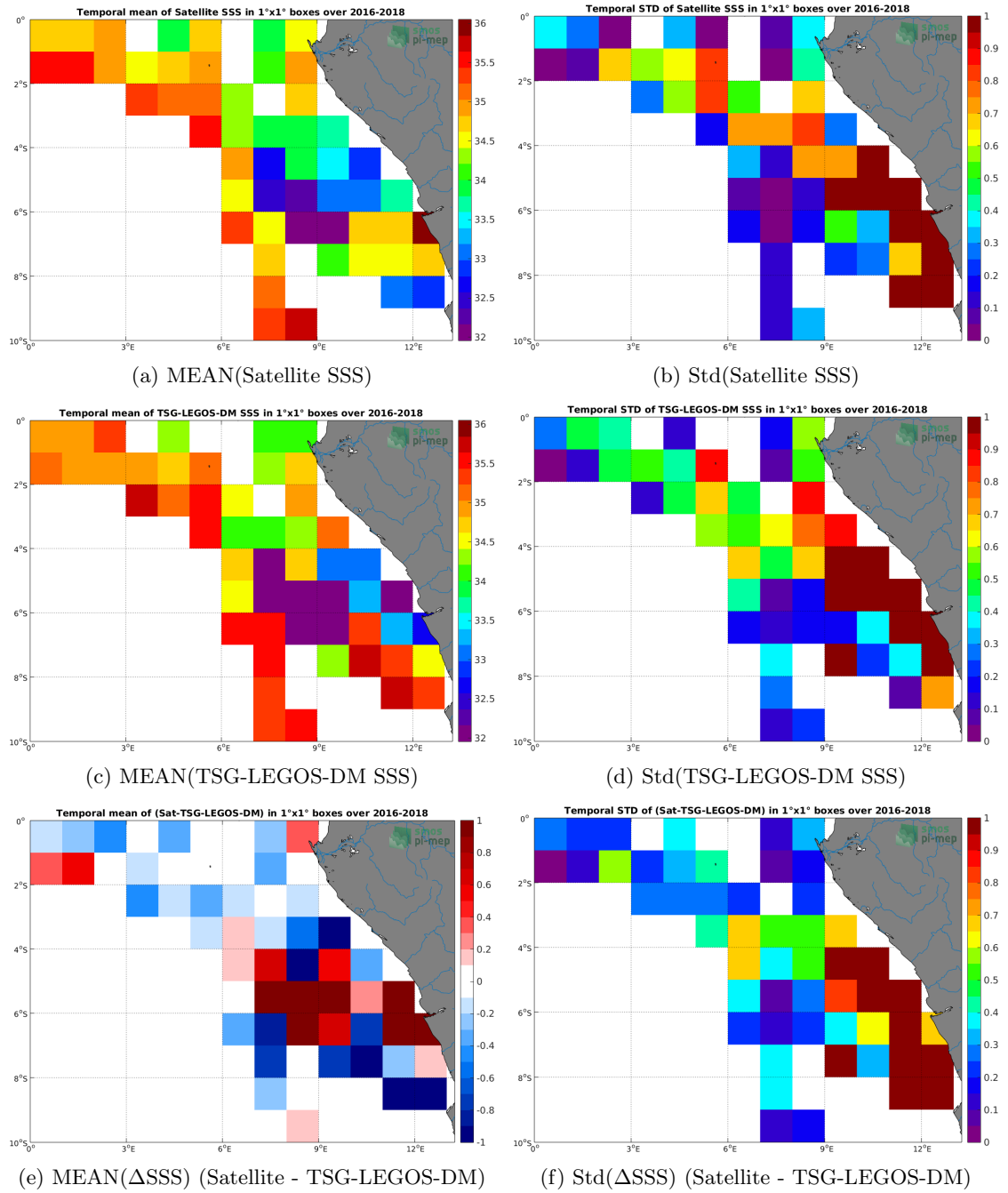
Figure 6: Temporal mean (left) and Std (right) of SSS from SMOS-L3-CATDS-CPDC-V3-MONTHLY-25KM (top), TSG-LEGOS-DM (middle), and of \Delta SSS (Satellite - TSG-LEGOS-DM). Only match-up pairs are used to generate these maps.
