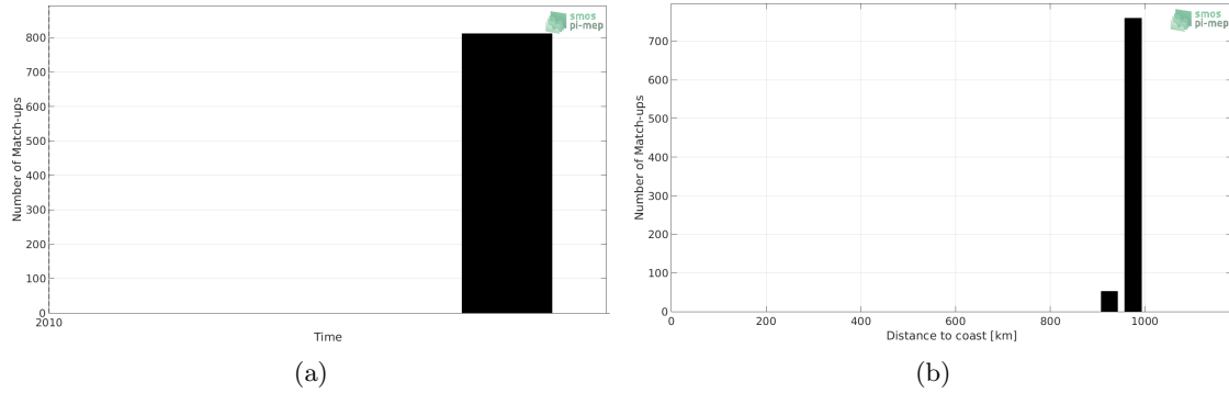
Figure 1: Number of match-ups between TSG-SAMOS and SMOS-L3-CATDS-CPDC-V3-10DAYS-25KM SSS as a function of time (a) and as function of the distance to coast (b) over the Congo river plume Pi-MEP region and for the full satellite product period.
