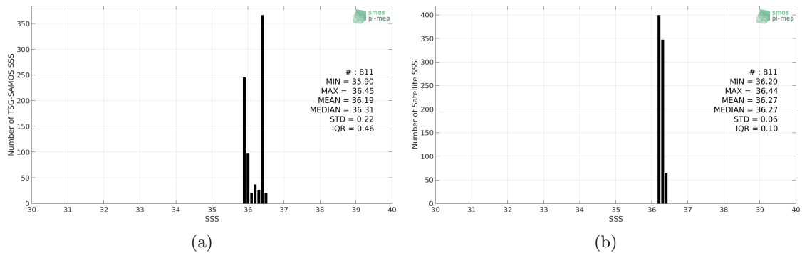
Figure 2: Histograms of SSS from TSG-SAMOS (a) and SMOS-L3-CATDS-CPDC-V3-10DAYS-25KM (b) considering all match-up pairs per bins of 0.1 over the Congo river plume Pi-MEP region and for the full satellite product period.
