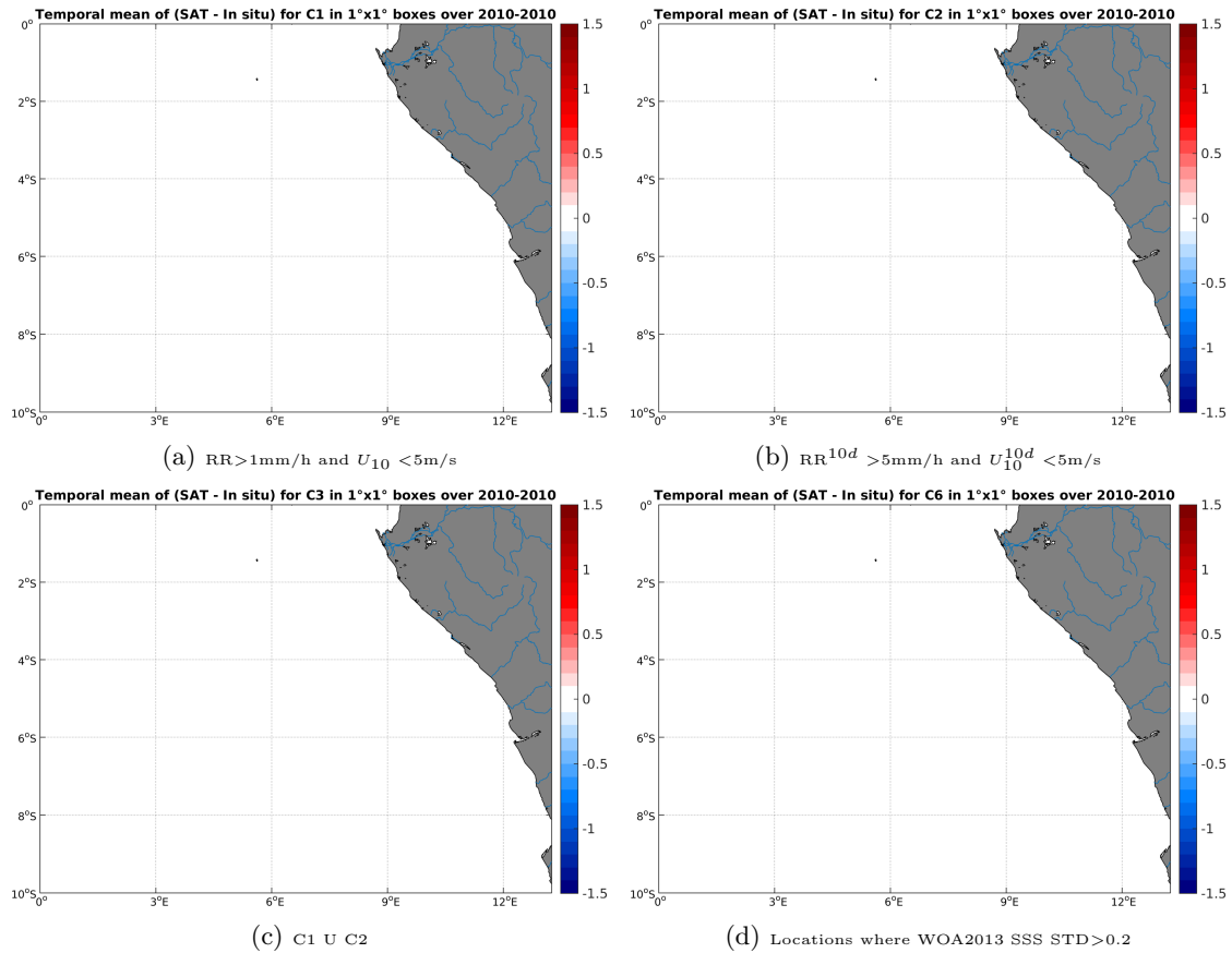
Figure 12: Temporal mean gridded over spatial boxes of size 1^\circ \times 1^\circ of \Delta SSS (SMOS-L3-CATDS-CPDC-V3-10DAYS-25KM - TSG-SAMOS) for 4 different subdatasets corresponding to: RR > 1 mm/h and U_{10} < 5 m/s (a), RR^{10d} > 5 mm/h and U_{10}^{10d} < 5 m/s (b), C1 \cup C2 (c), Locations where WOA2013 SSS STD > 0.2 (d).
