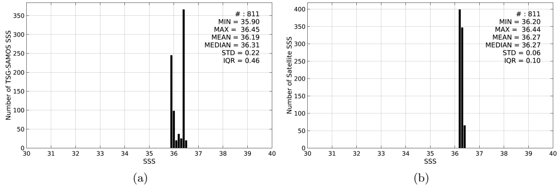
Figure 2: Histograms of SSS from TSG-SAMOS (a) and SMOS-L3-CATDS-CPDC-V3-10DAYS-25KM (b) considering all match-up pairs per bins of 0.1 over the Congo river plume Pi-MEP region and for the full satellite product period.
