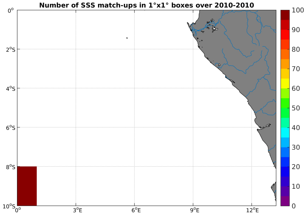
Figure 4: Number of SSS match-ups between TSG-SAMOS SSS and the SMOS-L3-CATDS-CPDC-V3-10DAYS-25KM SSS product for the Congo river plume Pi-MEP region over 1^\circ \times 1^\circ boxes and for the full satellite product period.
