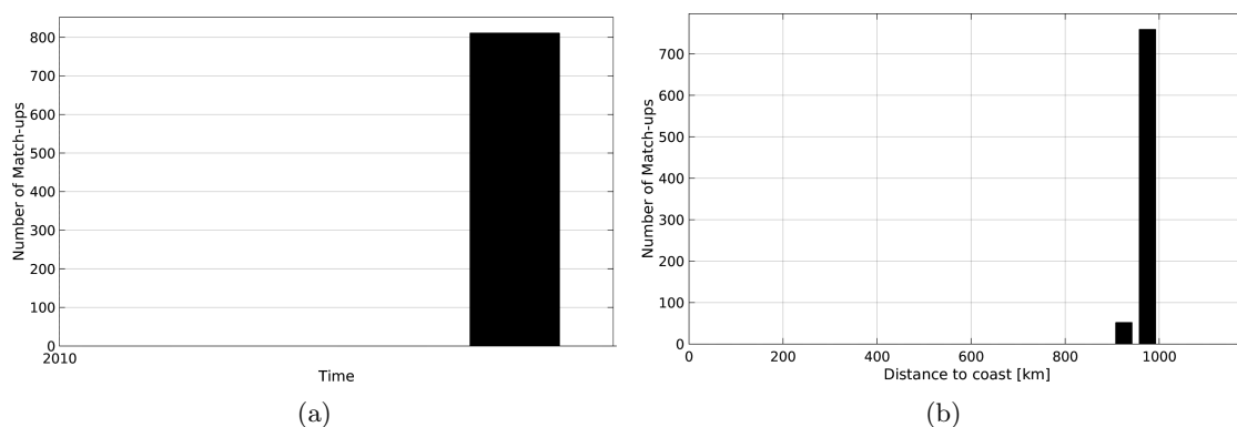
Figure 1: Number of match-ups between TSG-SAMOS and SMOS-L3-CATDS-CPDC-V3-10DAYS-25KM SSS as a function of time (a) and as function of the distance to coast (b) over the Congo river plume Pi-MEP region and for the full satellite product period.
