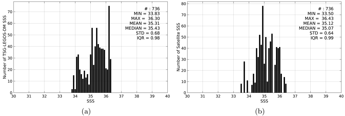
Figure 2: Histograms of SSS from TSG-LEGOS-DM (a) and SMOS-L3-CATDS-CPDC-V3-10DAYS-25KM (b) considering all match-up pairs per bins of 0.1 over the Congo river plume Pi-MEP region and for the full satellite product period.
