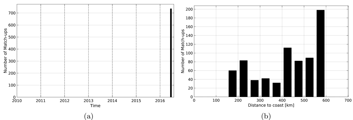
Figure 1: Number of match-ups between TSG-LEGOS-DM and SMOS-L3-CATDS-CPDC-V3-10DAYS-25KM SSS as a function of time (a) and as function of the distance to coast (b) over the Congo river plume Pi-MEP region and for the full satellite product period.
