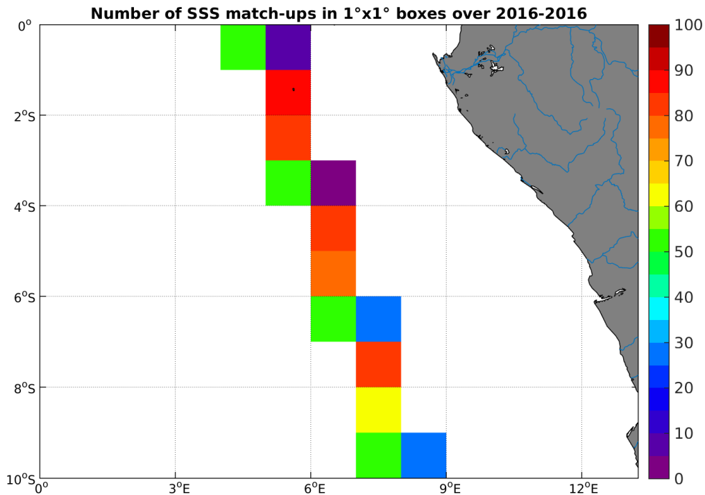
Figure 4: Number of SSS match-ups between TSG-LEGOS-DM SSS and the SMOS-L3-CATDS-CPDC-V3-10DAYS-25KM SSS product for the Congo river plume Pi-MEP region over 1°x1° boxes and for the full satellite product period.
