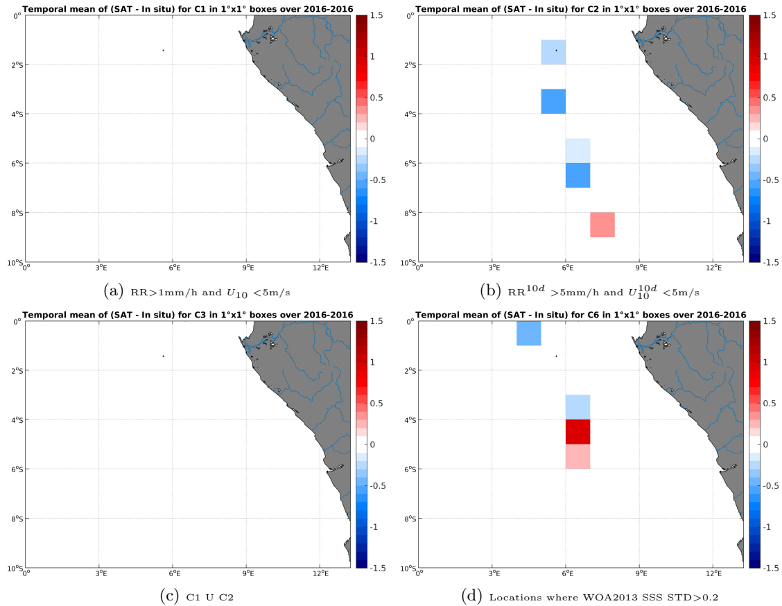
Figure 12: Temporal mean gridded over spatial boxes of size 1^\circ \times 1^\circ of \Delta SSS (SMOS-L3-CATDS-CPDC-V3-10DAYS-25KM - TSG-LEGOS-DM) for 4 different subdatasets corresponding to: RR > 1 mm/h and U_{10} < 5 m/s (a), RR^{10d} > 5 mm/h and U_{10}^{10d} < 5 m/s (b), C1 \cup C2 (c), Locations where WOA2013 SSS STD > 0.2 (d).
