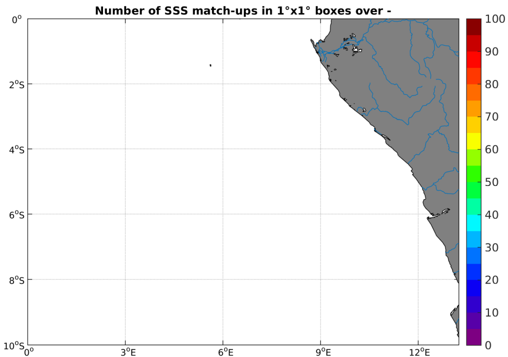
Figure 4: Number of SSS match-ups between TSG-GOSUD-Sailing-ship SSS and the SMOS-L3-CATDS-CPDC-V3-10DAYS-25KM SSS product for the Congo river plume Pi-MEP region over 1^\circ \times 1^\circ boxes and for the full satellite product period.
