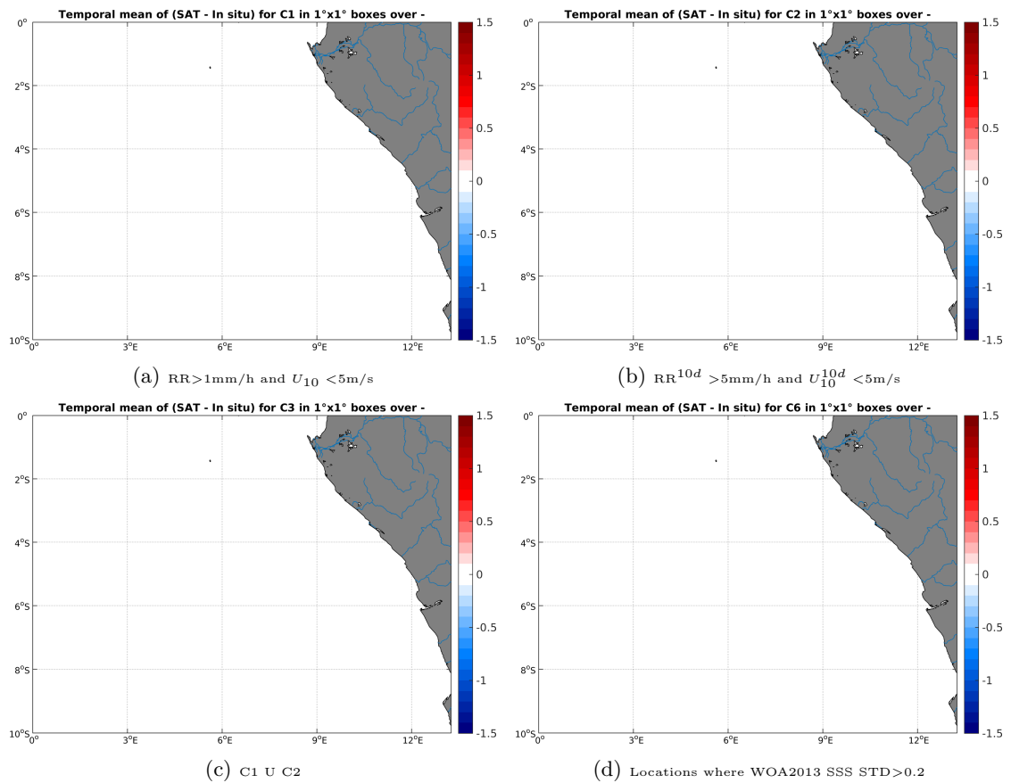
Figure 12: Temporal mean gridded over spatial boxes of size 1^\circ \times 1^\circ of \Delta SSS (SMOS-L3-CATDS-CPDC-V3-10DAYS-25KM - TSG-GOSUD-Sailing-ship) for 4 different subdatasets corresponding to:RR >1 mm/h and U_{10} < 5 m/s (a), RR ^{10d} > 5 mm/h and U_{10}^{10d} < 5 m/s (b), C1 U C2 (c),Locations where WOA2013 SSS STD >0.2 (d).
