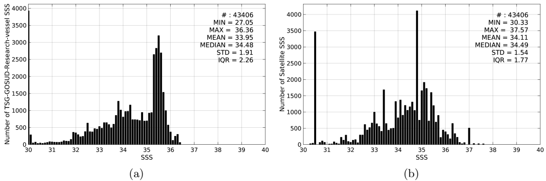
Figure 2: Histograms of SSS from TSG-GOSUD-Research-vessel (a) and SMOS-L3-CATDS-CPDC-V3-10DAYS-25KM (b) considering all match-up pairs per bins of 0.1 over the Congo river plume Pi-MEP region and for the full satellite product period.
