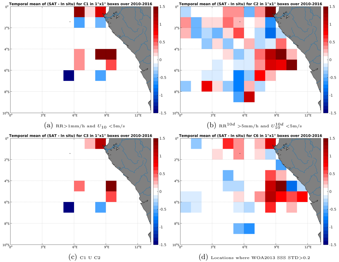
Figure 12: Temporal mean gridded over spatial boxes of size 1^\circ \times 1^\circ of \Delta SSS (SMOS-L3-CATDS-CPDC-V3-10DAYS-25KM - TSG-GOSUD-Research-vessel) for 4 different subdatasets corresponding to:RR >1 mm/h and U_{10} < 5 m/s (a), RR ^{10d} > 5 mm/h and U_{10}^{10d} < 5 m/s (b), C1 U C2 (c),Locations where WOA2013 SSS STD >0.2 (d).
