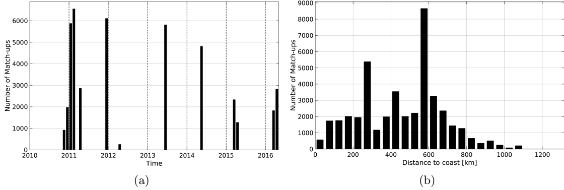
Figure 1: Number of match-ups between TSG-GOSUD-Research-vessel and SMOS-L3-CATDS-CPDC-V3-10DAYS-25KM SSS as a function of time (a) and as function of the distance to coast (b) over the Congo river plume Pi-MEP region and for the full satellite product period.
