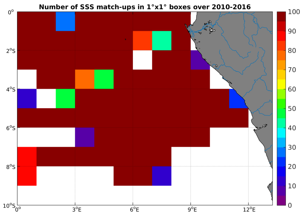
Figure 4: Number of SSS match-ups between TSG-GOSUD-Research-vessel SSS and the SMOS-L3-CATDS-CPDC-V3-10DAYS-25KM SSS product for the Congo river plume Pi-MEP region over 1^\circ \times 1^\circ boxes and for the full satellite product period.
