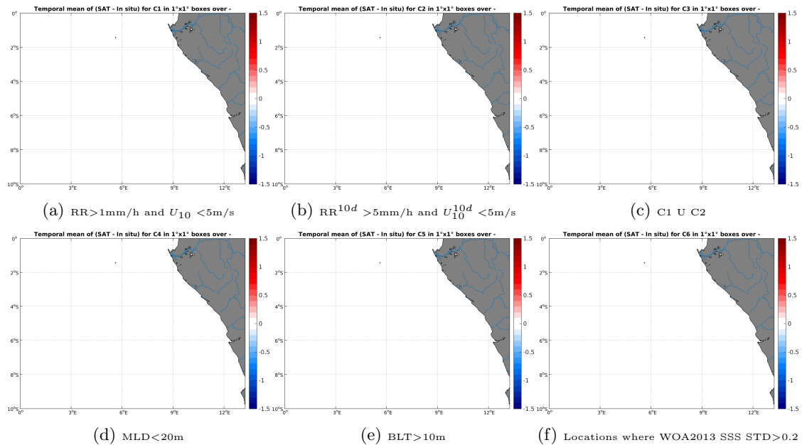
Figure 12: Temporal mean gridded over spatial boxes of size 1^\circ \times 1^\circ of \Delta SSS (SMOS-L3-CATDS-CPDC-V3-10DAYS-25KM - Sea mammals) for 6 different subdatasets corresponding to: RR > 1\text{mm/h} and U_{10} < 5\text{m/s} (a), RR^{10d} > 5\text{mm/h} and U_{10}^{10d} < 5\text{m/s} (b), C1 U C2 (c), MLD < 20\text{m} (d), BLT > 10\text{m} (e), Locations where WOA2013 SSS STD > 0.2 (f).
