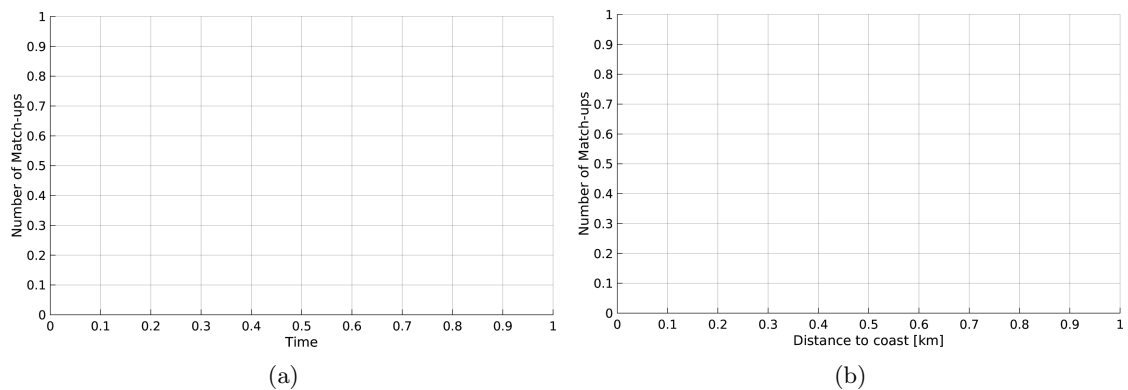
Figure 1: Number of match-ups between Sea mammals and SMOS-L3-CATDS-CPDC-V3-10DAYS-25KM SSS as a function of time (a) and as function of the distance to coast (b) over the Congo river plume Pi-MEP region and for the full satellite product period.
