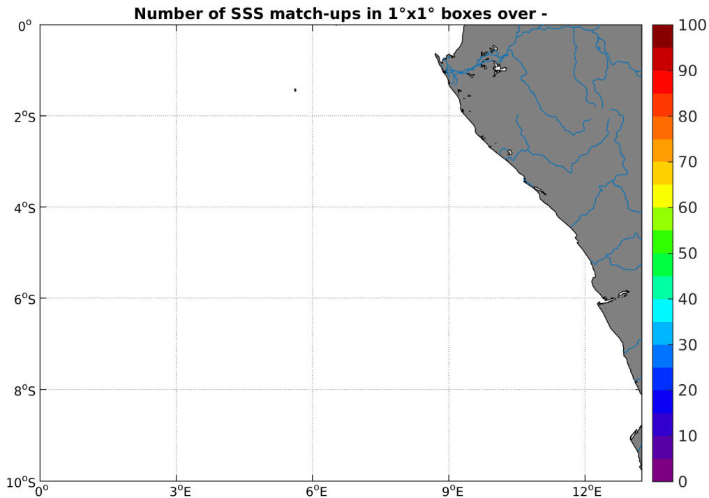
Figure 4: Number of SSS match-ups between Sea mammals SSS and the SMOS-L3-CATDS-CPDC-V3-10DAYS-25KM SSS product for the Congo river plume Pi-MEP region over 1^\circ \times 1^\circ boxes and for the full satellite product period.
