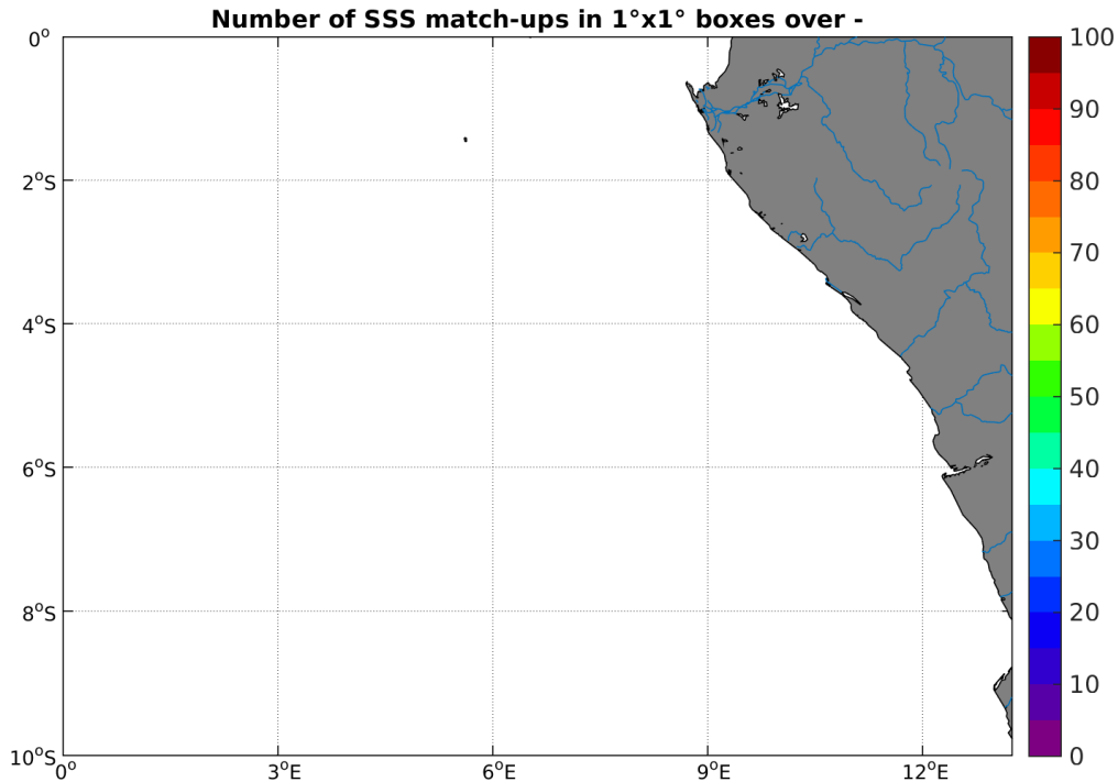
Figure 3: Number of SSS match-ups between Surface drifters SSS and the SMOS-L3-CATDS-CPDC-V3-10DAYS-25KM SSS product for the Congo river plume Pi-MEP region over 1^\circ \times 1^\circ boxes and for the full satellite product period.
