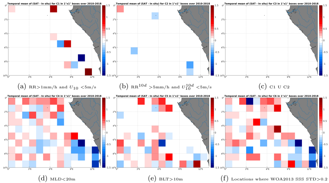
Figure 12: Temporal mean gridded over spatial boxes of size 1^\circ \times 1^\circ of \Delta SSS (SMOS-L3-CATDS-CPDC-V3-10DAYS-25KM - Argo) for 6 different subdatasets corresponding to:RR >1 mm/h and U_{10} < 5 m/s (a), RR^{10d} > 5 mm/h and U_{10}^{10d} < 5 m/s (b), C1 U C2 (c),MLD <20 m (d),BLT >10 m (e),Locations where WOA2013 SSS STD >0.2 (f).
