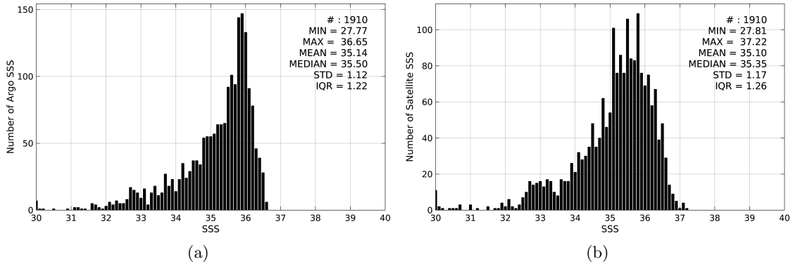
Figure 2: Histograms of SSS from Argo (a) and SMOS-L3-CATDS-CPDC-V3-10DAYS-25KM (b) considering all match-up pairs per bins of 0.1 over the Congo river plume Pi-MEP region and for the full satellite product period.
