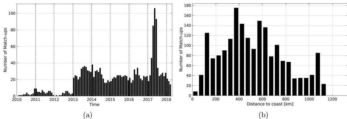
Figure 1: Number of match-ups between Argo and SMOS-L3-CATDS-CPDC-V3-10DAYS-25KM SSS as a function of time (a) and as function of the distance to coast (b) over the Congo river plume Pi-MEP region and for the full satellite product period.
