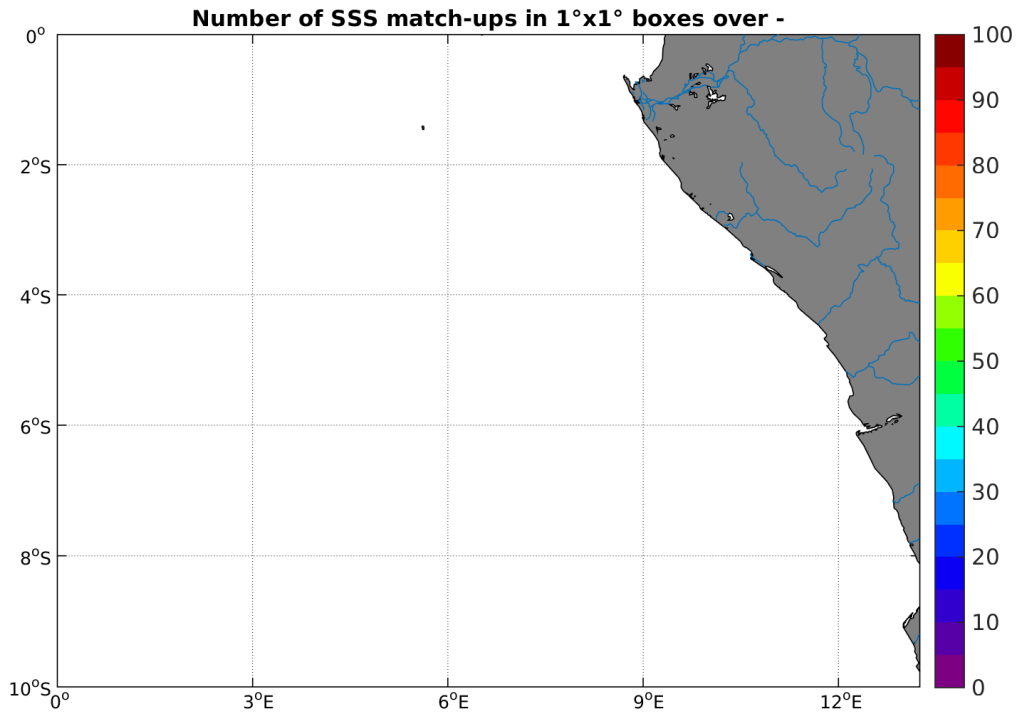
Figure 4: Number of SSS match-ups between TSG-SAMOS SSS and the SMOS-L3-BEC-OA-V1-9DAYS-0.25DEG SSS product for the Congo river plume Pi-MEP region over 1^\circ \times 1^\circ boxes and for the full satellite product period.
