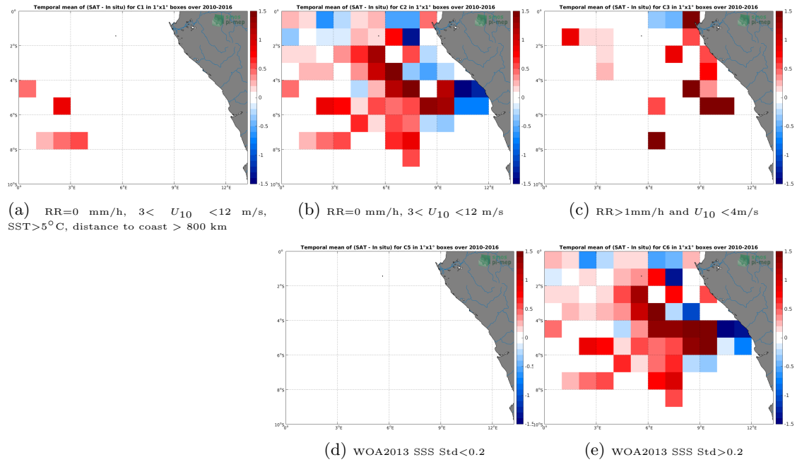
Figure 12: Temporal mean gridded over spatial boxes of size 1^\circ \times 1^\circ of \Delta SSS (SMOS-L3-BEC-OA-V1-9DAYS-0.25DEG - TSG-GOSUD-Research-vessel) for 5 different subdatasets corresponding to: RR=0 mm/h, 3 < U_{10} < 12 m/s, SST >5^\circ C, distance to coast > 800 km (a), RR=0 mm/h, 3 < U_{10} < 12 m/s (b), RR >1 mm/h and U_{10} < 4 m/s (c), WOA2013 SSS Std <0.2 (d), WOA2013 SSS Std >0.2 (e).
