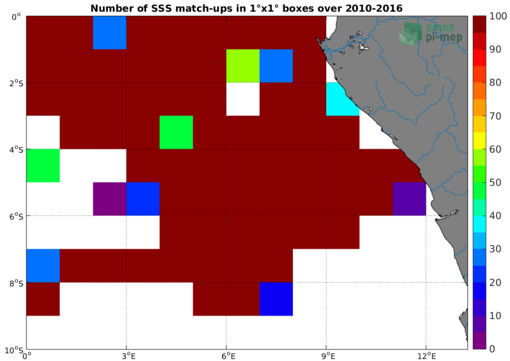
Figure 4: Number of SSS match-ups between TSG-GOSUD-Research-vessel SSS and the SMOS-L3-BEC-OA-V1-9DAYS-0.25DEG SSS product for the Congo river plume Pi-MEP region over 1^\circ \times 1^\circ boxes and for the full satellite product period.
