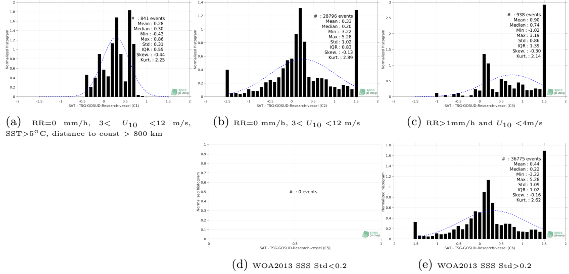
Figure 13: Normalized histogram of \Delta\text{SSS} (SMOS-L3-BEC-OA-V1-9DAYS-0.25DEG - TSG-GOSUD-Research-vessel) for 5 different subdatasets corresponding to: RR=0 mm/h, 3 < U_{10} < 12 m/s, SST > 5^\circ\text{C} , distance to coast > 800 km (a), RR=0 mm/h, 3 < U_{10} < 12 m/s (b), RR > 1\text{mm/h} and U_{10} < 4\text{m/s} (c), WOA2013 SSS \text{Std} < 0.2 (d), WOA2013 SSS \text{Std} > 0.2 (e).
