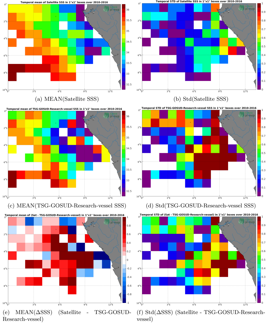
Figure 6: Temporal mean (left) and Std (right) of SSS from SMOS-L3-BEC-OA-V1-9DAYS-0.25DEG (top), TSG-GOSUD-Research-vessel (middle), and of \Delta SSS (Satellite - TSG-GOSUD-Research-vessel). Only match-up pairs are used to generate these maps.
