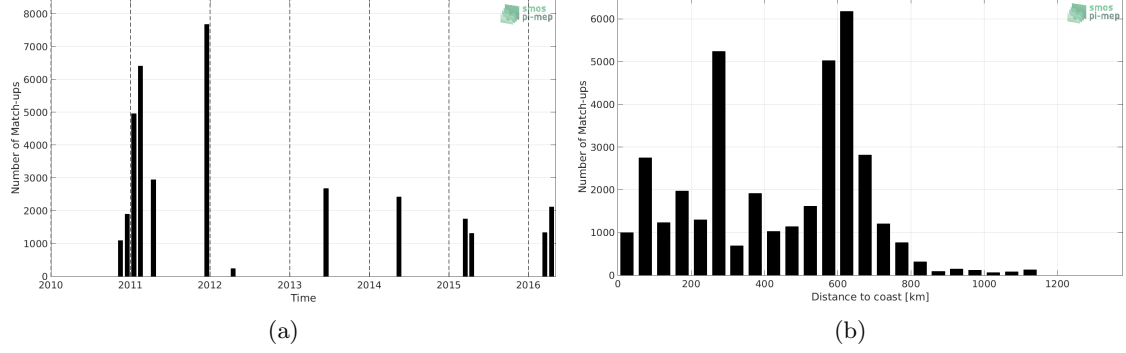
Figure 1: Number of match-ups between TSG-GOSUD-Research-vessel and SMOS-L3-BEC-OA-V1-9DAYS-0.25DEG SSS as a function of time (a) and as function of the distance to coast (b) over the Congo river plume Pi-MEP region and for the full satellite product period.
