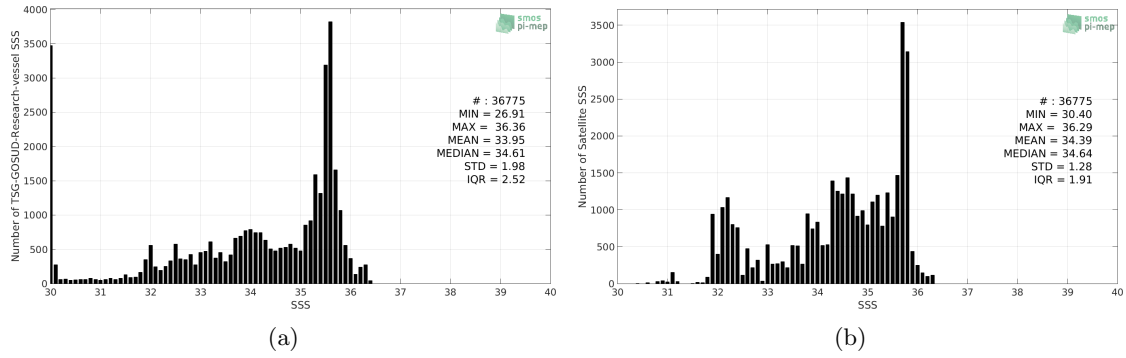
Figure 2: Histograms of SSS from TSG-GOSUD-Research-vessel (a) and SMOS-L3-BEC-OA-V1-9DAYS-0.25DEG (b) considering all match-up pairs per bins of 0.1 over the Congo river plume Pi-MEP region and for the full satellite product period.
