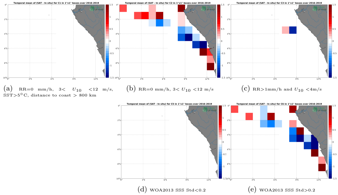
Figure 12: Temporal mean gridded over spatial boxes of size 1^\circ \times 1^\circ of \Delta SSS (SMOS SSS L2 v700 (ESA) - TSG (LEGOS-DM)) for 5 different subdatasets corresponding to: RR=0 mm/h, 3 < U_{10} < 12 m/s, SST > 5^\circ C , distance to coast > 800 km (a), RR=0 mm/h, 3 < U_{10} < 12 m/s (b), RR > 1 mm/h and U_{10} < 4 m/s (c), WOA2013 SSS Std < 0.2 (d), WOA2013 SSS Std > 0.2 (e).
