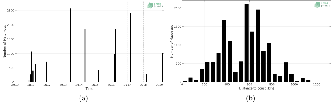
Figure 1: Number of match-ups between TSG (GOSUD-Research-vessel) and SMOS SSS L2 v700 (ESA) SSS as a function of time (a) and as function of the distance to coast (b) over the Congo river plume Pi-MEP region and for the full satellite product period.
