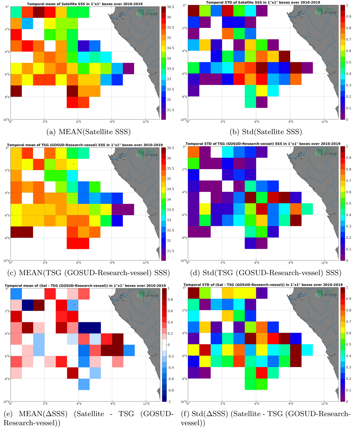
Figure 6: Temporal mean (left) and Std (right) of SSS from SMOS SSS L2 v700 (ESA) (top), TSG (GOSUD-Research-vessel) (middle), and of \Delta SSS (Satellite - TSG (GOSUD-Research-vessel)). Only match-up pairs are used to generate these maps.
