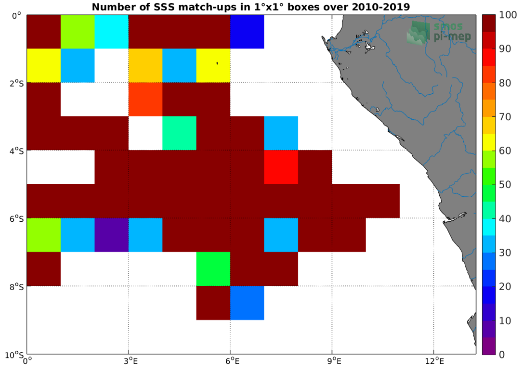
Figure 4: Number of SSS match-ups between TSG (GOSUD-Research-vessel) SSS and the SMOS SSS L2 v700 (ESA) SSS product for the Congo river plume Pi-MEP region over 1^\circ \times 1^\circ boxes and for the full satellite product period.
