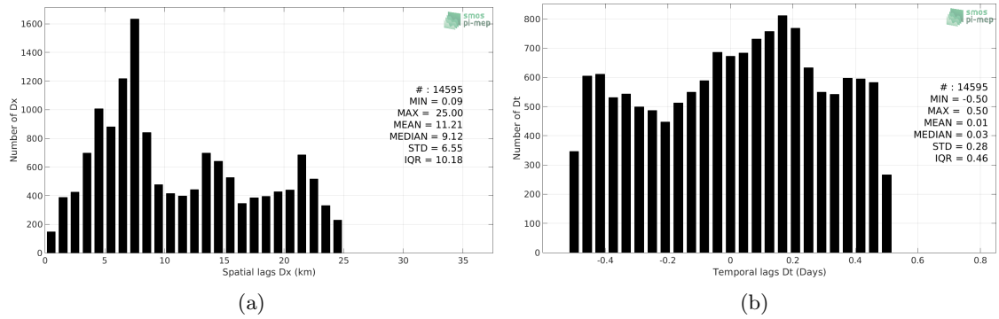
Figure 5: Histograms of the spatial (a) and temporal (b) lags between the location/time of the TSG (GOSUD-Research-vessel) measurement and the date of the corresponding SMOS SSS L2 v700 (ESA) SSS pixel.
