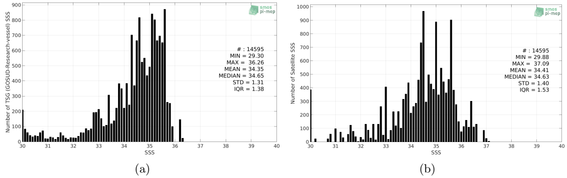
Figure 2: Histograms of SSS from TSG (GOSUD-Research-vessel) (a) and SMOS SSS L2 v700 (ESA) (b) considering all match-up pairs per bins of 0.1 over the Congo river plume Pi-MEP region and for the full satellite product period.
