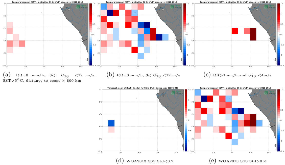
Figure 12: Temporal mean gridded over spatial boxes of size 1^\circ \times 1^\circ of \Delta SSS (SMOS SSS L2 v700 (ESA) - TSG (GOSUD-Research-vessel)) for 5 different subdatasets corresponding to: RR=0 mm/h, 3 < U_{10} < 12 m/s, SST > 5^\circ C , distance to coast > 800 km (a), RR=0 mm/h, 3 < U_{10} < 12 m/s (b), RR > 1 mm/h and U_{10} < 4 m/s (c), WOA2013 SSS Std < 0.2 (d), WOA2013 SSS Std > 0.2 (e).
