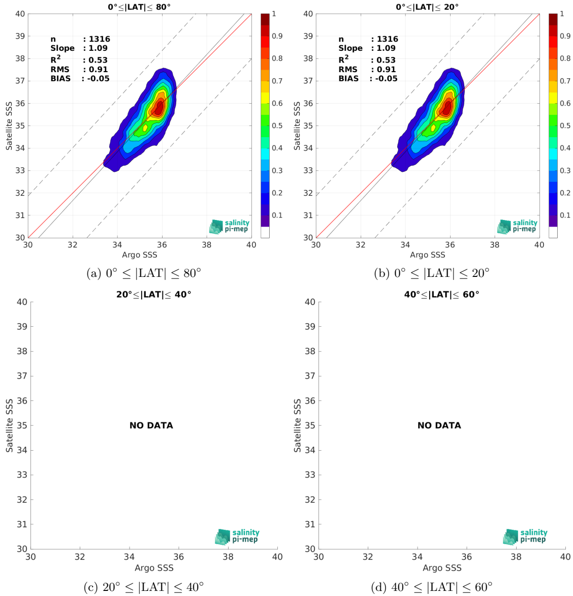
Figure 10: Contour maps of the concentration of SMOS SSS L2 v700 (ESA) SSS (y-axis) versus Argo SSS (x-axis) at match-up pairs for different latitude bands. For each plot, the red line shows x=y . The black thin and dashed lines indicate a linear fit through the data cloud and the \pm 95\% confidence levels, respectively. The number match-up pairs n , the slope and R^2 coefficient of the linear fit, the root mean square (RMS) and the mean bias between satellite and in situ data are indicated for each latitude band in each plots.
