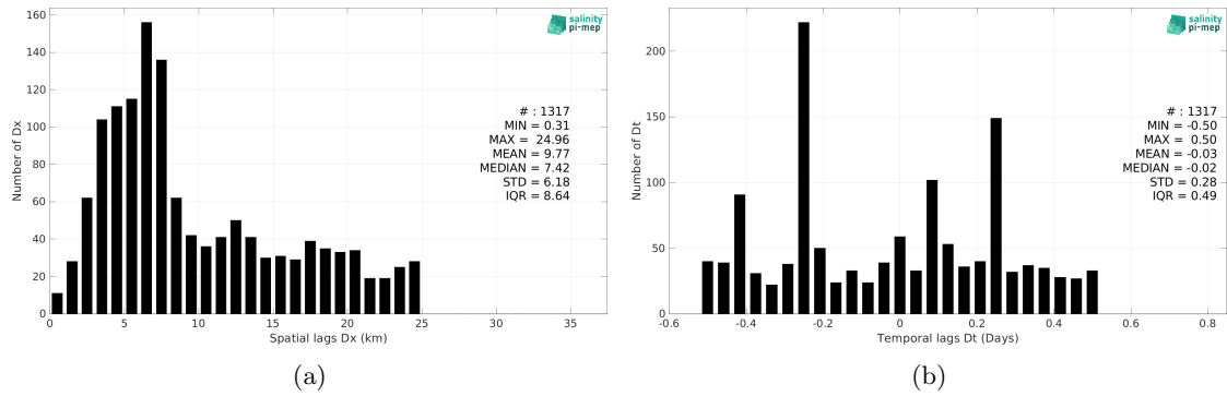
Figure 6: Histograms of the spatial (a) and temporal (b) lags between the location/time of the Argo measurement and the date of the corresponding SMOS SSS L2 v700 (ESA) SSS pixel.
