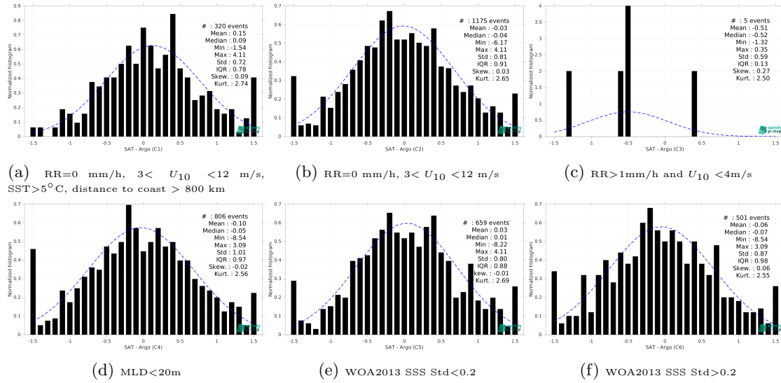
Figure 15: Normalized histogram of \Delta\text{SSS} (SMOS SSS L2 v700 (ESA) - Argo) for 6 different subdatasets corresponding to: RR=0 mm/h, 3 < U_{10} < 12 m/s, SST>5°C, distance to coast > 800 km (a), RR=0 mm/h, 3 < U_{10} < 12 m/s (b), RR>1mm/h and U_{10} < 4 m/s (c), MLD<20m (d), WOA2013 SSS Std<0.2 (e), WOA2013 SSS Std>0.2 (f).
