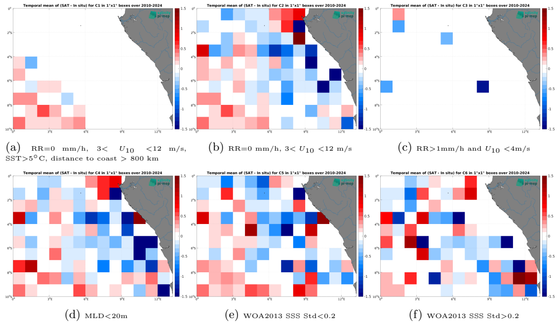
Figure 14: Temporal mean gridded over spatial boxes of size 1^\circ \times 1^\circ of \Delta SSS (SMOS SSS L2 v700 (ESA) - Argo) for 6 different subdatasets corresponding to:RR=0 mm/h, 3 < U_{10} < 12 m/s, SST >5^\circ\text{C} , distance to coast > 800 km (a), RR=0 mm/h, 3 < U_{10} < 12 m/s (b), RR >1 mm/h and U_{10} < 4 m/s (c),MLD <20 m (d),WOA2013 SSS Std <0.2 (e),WOA2013 SSS Std >0.2 (f).
