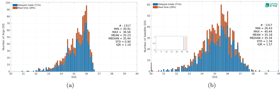
Figure 3: Histograms of SSS from Argo (a) and SMOS SSS L2 v700 (ESA) (b) considering all match-up pairs per bins of 0.1 over the Congo river plume Pi-MEP region and for the full satellite product period.
