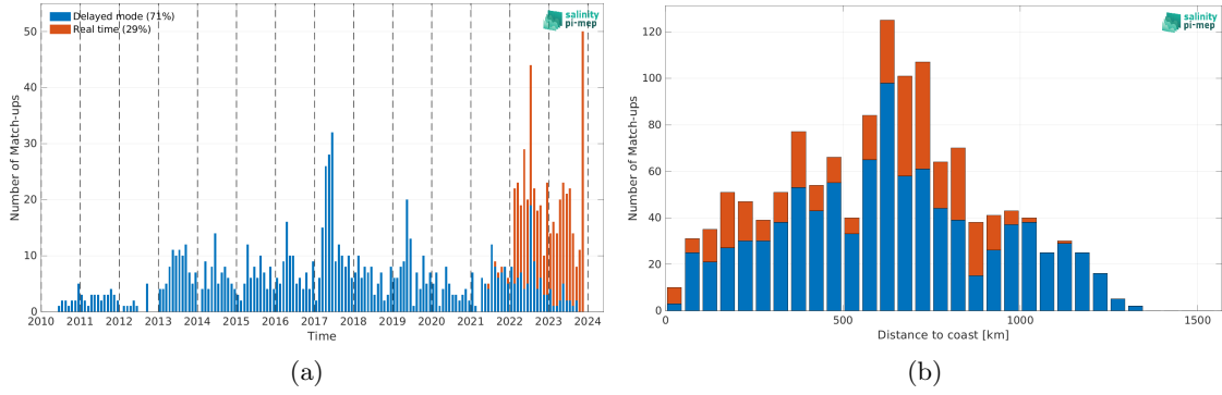
Figure 2: Number of match-ups between Argo and SMOS SSS L2 v700 (ESA) SSS as a function of time (a) and as function of the distance to coast (b) over the Congo river plume Pi-MEP region and for the full satellite product period.
