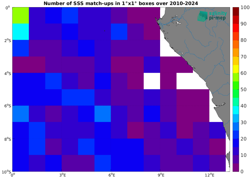
Figure 5: Number of SSS match-ups between Argo SSS and the SMOS SSS L2 v700 (ESA) SSS product for the Congo river plume Pi-MEP region over 1^\circ \times 1^\circ boxes and for the full satellite product period.
