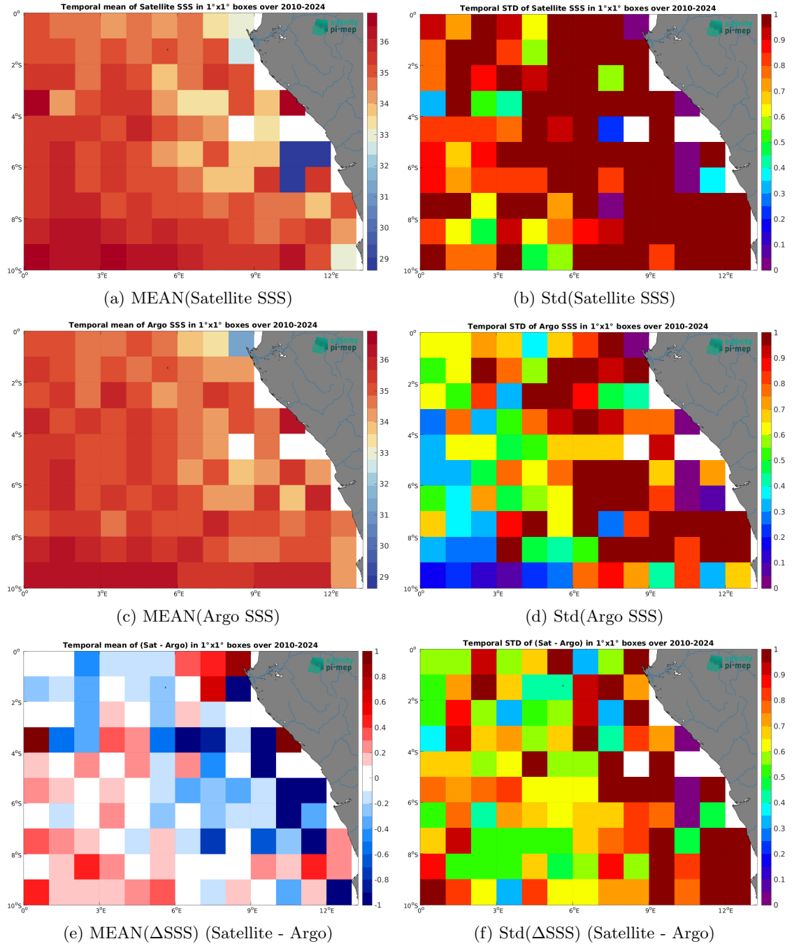
Figure 7: Temporal mean (left) and Std (right) of SSS from SMOS SSS L2 v700 (ESA) (top), Argo (middle), and of \Delta SSS (Satellite - Argo). Only match-up pairs are used to generate these maps.
