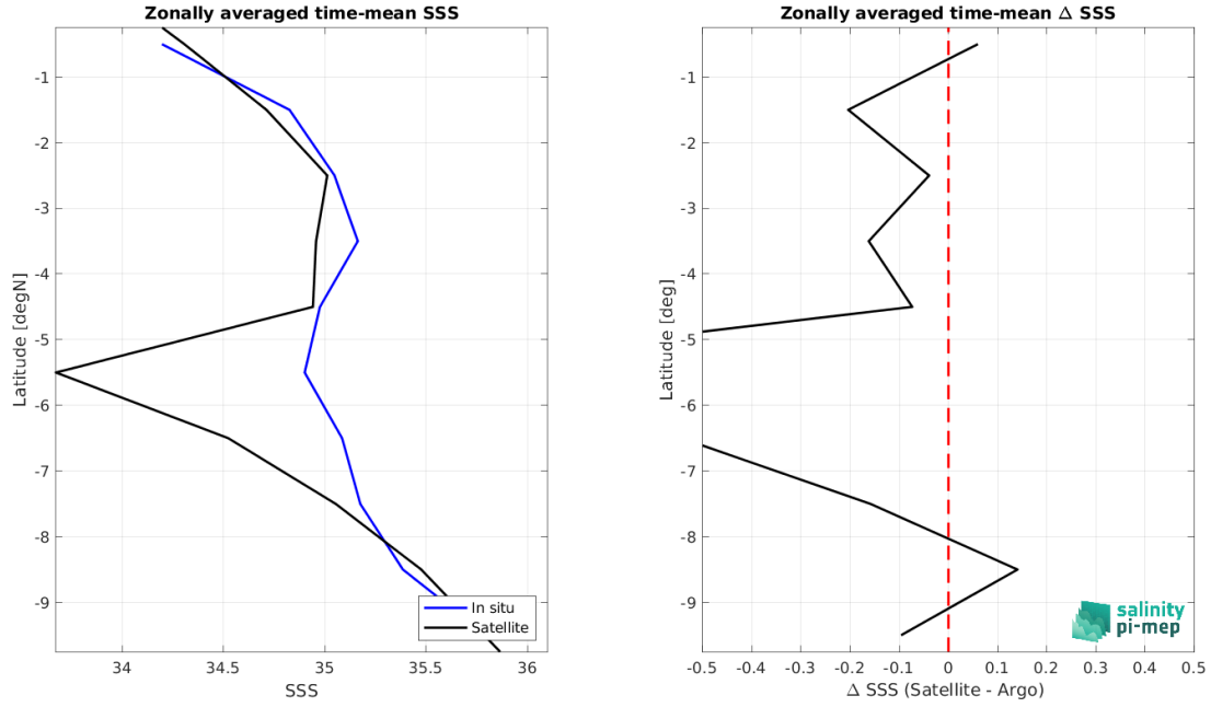
Figure 9: Left panel: Zonal mean SSS from SMOS SSS L2 v700 (ESA) satellite product (black) and from Argo (blue). Right panel: Zonal mean of \Delta SSS (Satellite - Argo) for all the collected Pi-MEP match-up pairs estimated over the full satellite product period.
