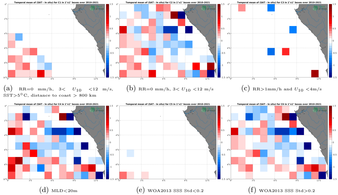
Figure 12: Temporal mean gridded over spatial boxes of size 1^\circ \times 1^\circ of \Delta SSS (SMOS SSS L2 v700 (ESA) - Argo) for 6 different subdatasets corresponding to: RR=0 mm/h, 3 < U_{10} < 12 m/s, SST >5^\circ\text{C} , distance to coast > 800 km (a), RR=0 mm/h, 3 < U_{10} < 12 m/s (b), RR >1 mm/h and U_{10} < 4 m/s (c), MLD <20 m (d), WOA2013 SSS Std <0.2 (e), WOA2013 SSS Std >0.2 (f).
