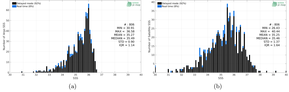
Figure 2: Histograms of SSS from Argo (a) and SMOS SSS L2 v700 (ESA) (b) considering all match-up pairs per bins of 0.1 over the Congo river plume Pi-MEP region and for the full satellite product period.
