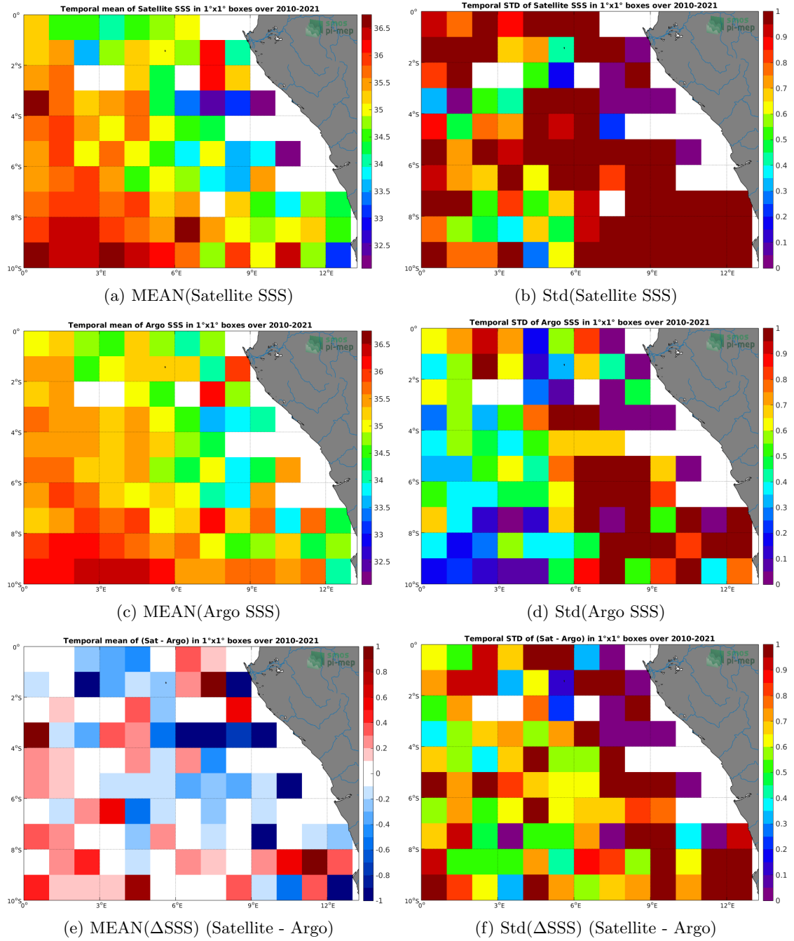
Figure 6: Temporal mean (left) and Std (right) of SSS from SMOS SSS L2 v700 (ESA) (top), Argo (middle), and of \Delta SSS (Satellite - Argo). Only match-up pairs are used to generate these maps.
