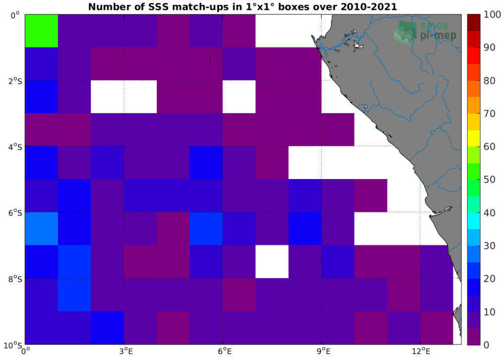
Figure 4: Number of SSS match-ups between Argo SSS and the SMOS SSS L2 v700 (ESA) SSS product for the Congo river plume Pi-MEP region over 1^\circ \times 1^\circ boxes and for the full satellite product period.
