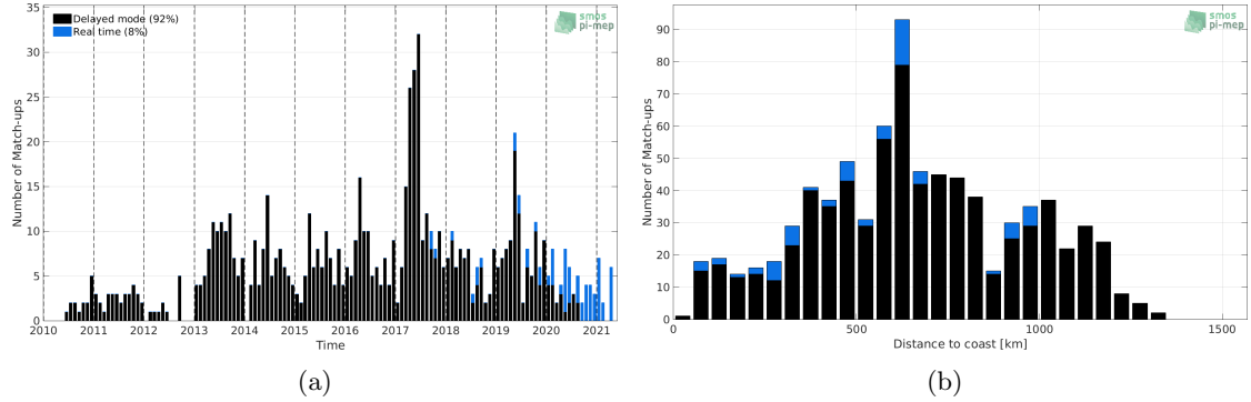
Figure 1: Number of match-ups between Argo and SMOS SSS L2 v700 (ESA) SSS as a function of time (a) and as function of the distance to coast (b) over the Congo river plume Pi-MEP region and for the full satellite product period.
