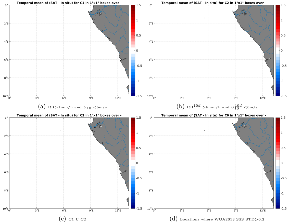
Figure 12: Temporal mean gridded over spatial boxes of size 1^\circ \times 1^\circ of \Delta SSS (SMOS-L2-DPGS-v662 - TSG-SAMOS) for 4 different subdatasets corresponding to: RR > 1\text{mm/h} and U_{10} < 5\text{m/s} (a), RR^{10d} > 5\text{mm/h} and U_{10}^{10d} < 5\text{m/s} (b), C1 \cup C2 (c), Locations where WOA2013 SSS STD > 0.2 (d).
