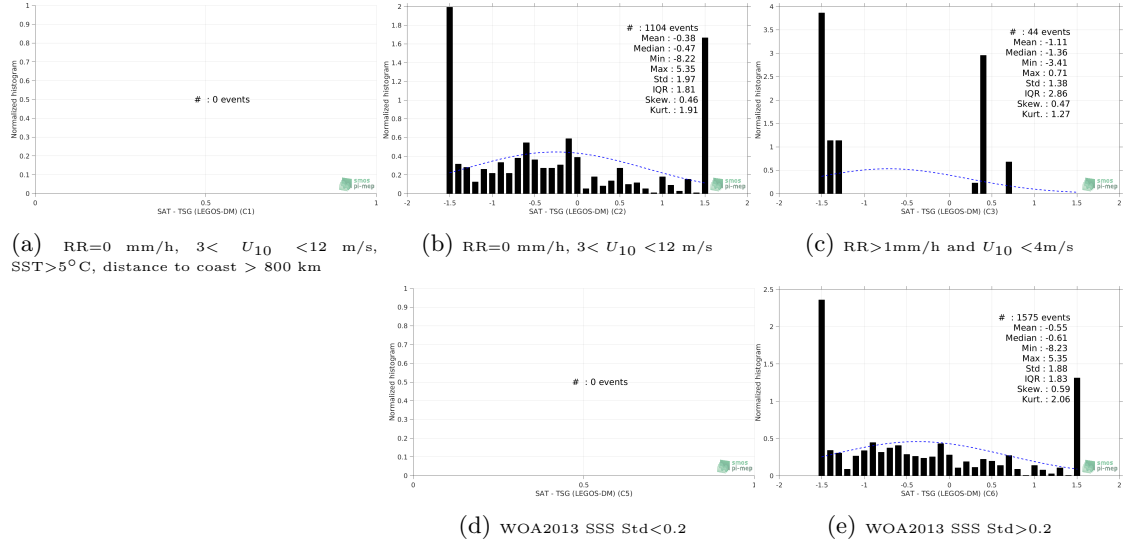
Figure 13: Normalized histogram of \Delta SSS (SMOS SSS L2 v662 (ESA) - TSG (LEGOS-DM)) for 5 different subdatasets corresponding to: RR=0 mm/h, 3 < U_{10} < 12 m/s, SST>5°C, distance to coast > 800 km (a), RR=0 mm/h, 3 < U_{10} < 12 m/s (b), RR>1mm/h and U_{10} < 4 m/s (c), WOA2013 SSS Std<0.2 (d), WOA2013 SSS Std>0.2 (e).
