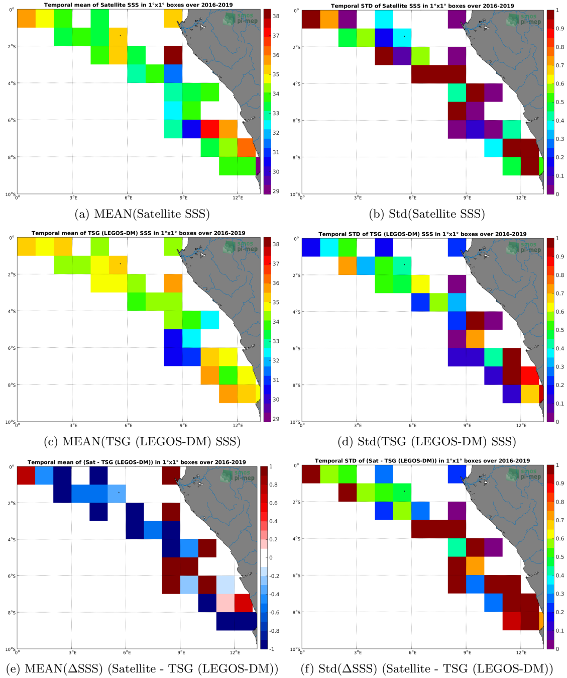
Figure 6: Temporal mean (left) and Std (right) of SSS from SMOS SSS L2 v662 (ESA) (top), TSG (LEGOS-DM) (middle), and of \Delta SSS (Satellite - TSG (LEGOS-DM)). Only match-up pairs are used to generate these maps.
