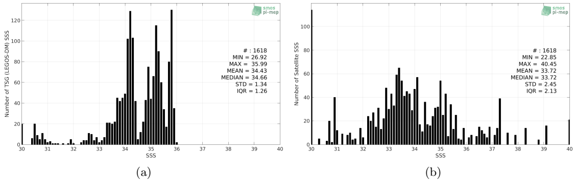
Figure 2: Histograms of SSS from TSG (LEGOS-DM) (a) and SMOS SSS L2 v662 (ESA) (b) considering all match-up pairs per bins of 0.1 over the Congo river plume Pi-MEP region and for the full satellite product period.
