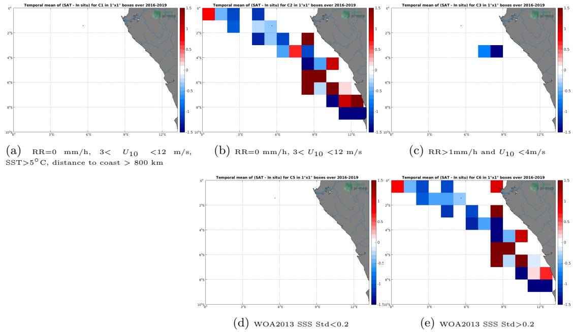
Figure 12: Temporal mean gridded over spatial boxes of size 1^\circ \times 1^\circ of \Delta SSS (SMOS SSS L2 v662 (ESA) - TSG (LEGOS-DM)) for 5 different subdatasets corresponding to: RR=0 mm/h, 3 < U_{10} < 12 m/s, SST > 5^\circ C , distance to coast > 800 km (a), RR=0 mm/h, 3 < U_{10} < 12 m/s (b), RR > 1 mm/h and U_{10} < 4 m/s (c), WOA2013 SSS Std < 0.2 (d), WOA2013 SSS Std > 0.2 (e).
