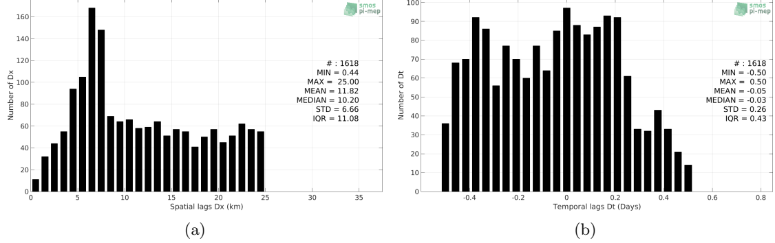
Figure 5: Histograms of the spatial (a) and temporal (b) lags between the time of the TSG (LEGOS-DM) measurements and the date of the corresponding SMOS SSS L2 v662 (ESA) SSS product.
