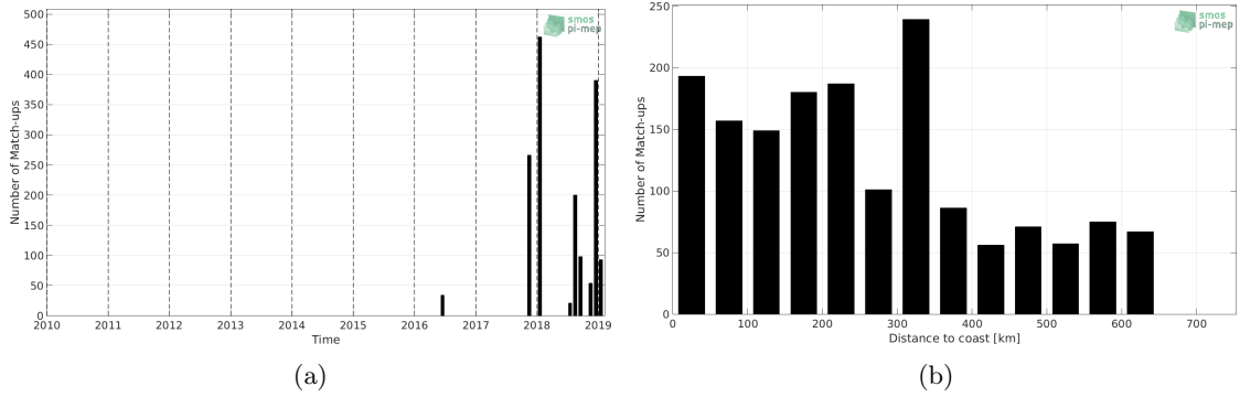
Figure 1: Number of match-ups between TSG (LEGOS-DM) and SMOS SSS L2 v662 (ESA) SSS as a function of time (a) and as function of the distance to coast (b) over the Congo river plume Pi-MEP region and for the full satellite product period.
