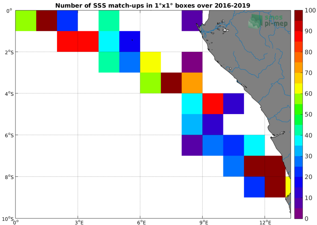
Figure 4: Number of SSS match-ups between TSG (LEGOS-DM) SSS and the SMOS SSS L2 v662 (ESA) SSS product for the Congo river plume Pi-MEP region over 1°x1° boxes and for the full satellite product period.
