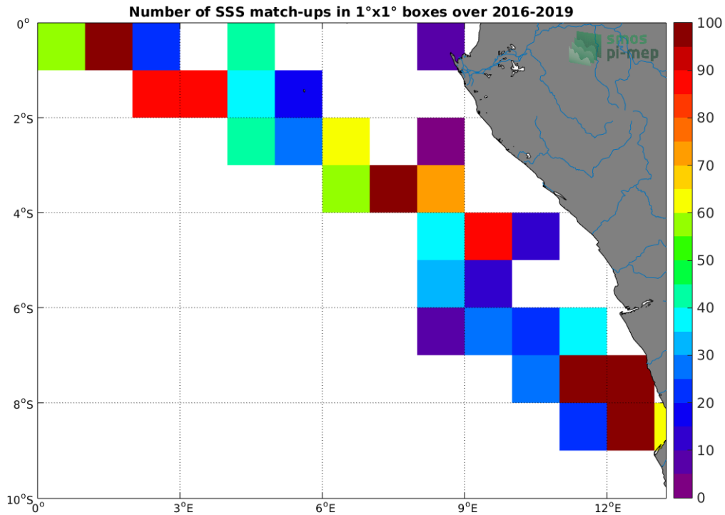
Figure 4: Number of SSS match-ups between TSG-LEGOS-DM SSS and the SMOS L2 v662 (ESA) SSS product for the Congo river plume Pi-MEP region over 1°x1° boxes and for the full satellite product period.
