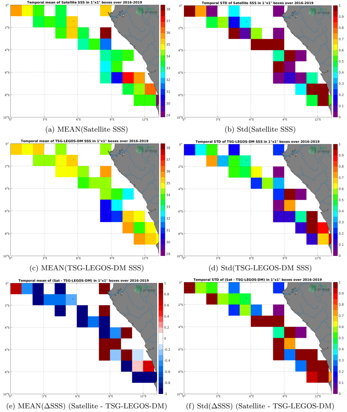
Figure 6: Temporal mean (left) and Std (right) of SSS from SMOS L2 v662 (ESA) (top), TSG-LEGOS-DM (middle), and of \Delta SSS (Satellite - TSG-LEGOS-DM). Only match-up pairs are used to generate these maps.
