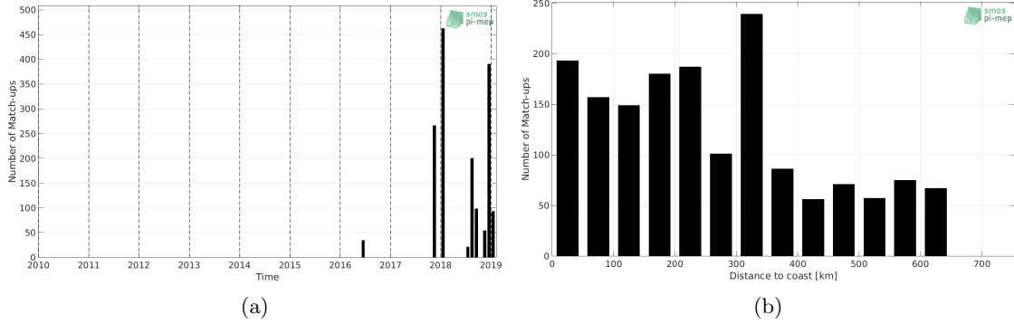
Figure 1: Number of match-ups between TSG-LEGOS-DM and SMOS L2 v662 (ESA) SSS as a function of time (a) and as function of the distance to coast (b) over the Congo river plume Pi-MEP region and for the full satellite product period.
