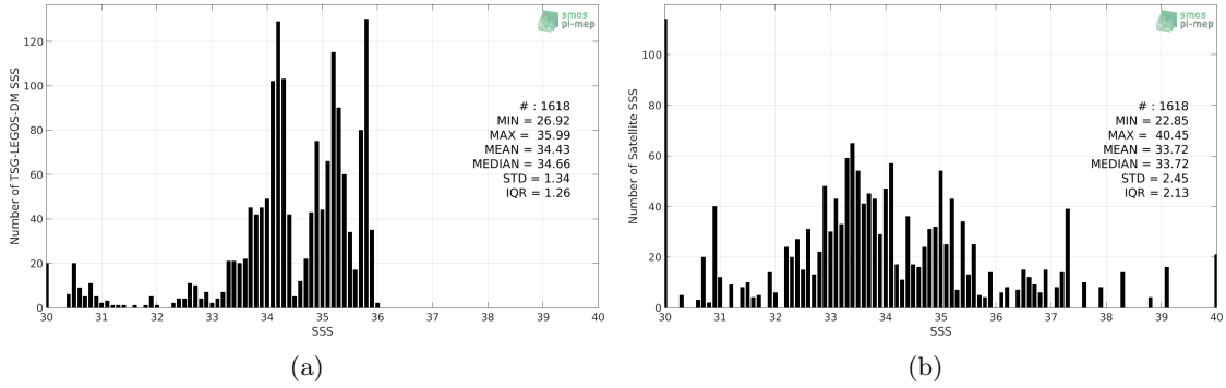
Figure 2: Histograms of SSS from TSG-LEGOS-DM (a) and SMOS L2 v662 (ESA) (b) considering all match-up pairs per bins of 0.1 over the Congo river plume Pi-MEP region and for the full satellite product period.
