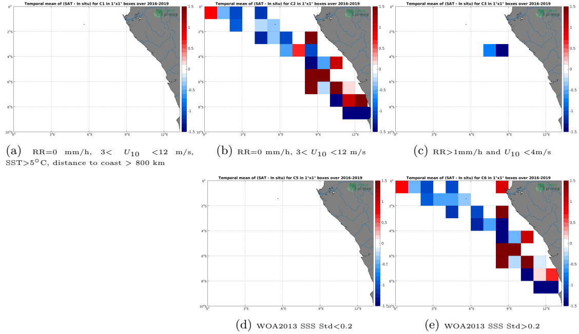
Figure 12: Temporal mean gridded over spatial boxes of size 1^\circ \times 1^\circ of \Delta SSS (SMOS L2 v662 (ESA) - TSG-LEGOS-DM) for 5 different subdatasets corresponding to: RR=0 mm/h, 3 < U_{10} < 12 m/s, SST > 5^\circ\text{C} , distance to coast > 800 km (a), RR=0 mm/h, 3 < U_{10} < 12 m/s (b), RR > 1\text{mm/h} and U_{10} < 4\text{m/s} (c), WOA2013 SSS Std < 0.2 (d), WOA2013 SSS Std > 0.2 (e).
