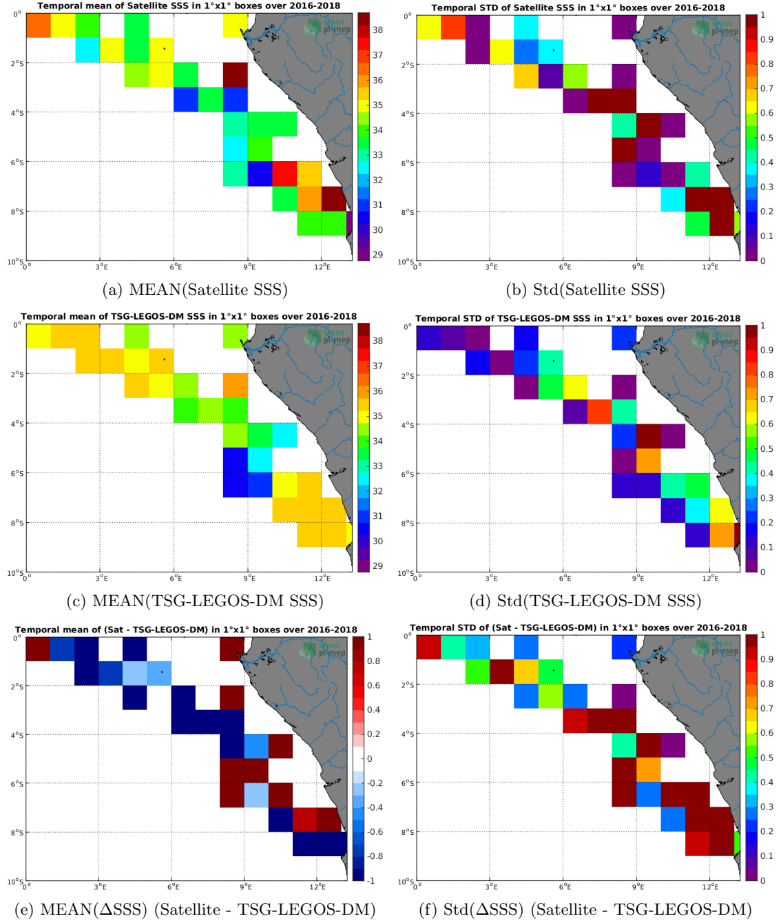
Figure 6: Temporal mean (left) and Std (right) of SSS from SMOS-L2-DPGS-v662 (top), TSG-LEGOS-DM (middle), and of \Delta SSS (Satellite - TSG-LEGOS-DM). Only match-up pairs are used to generate these maps.
