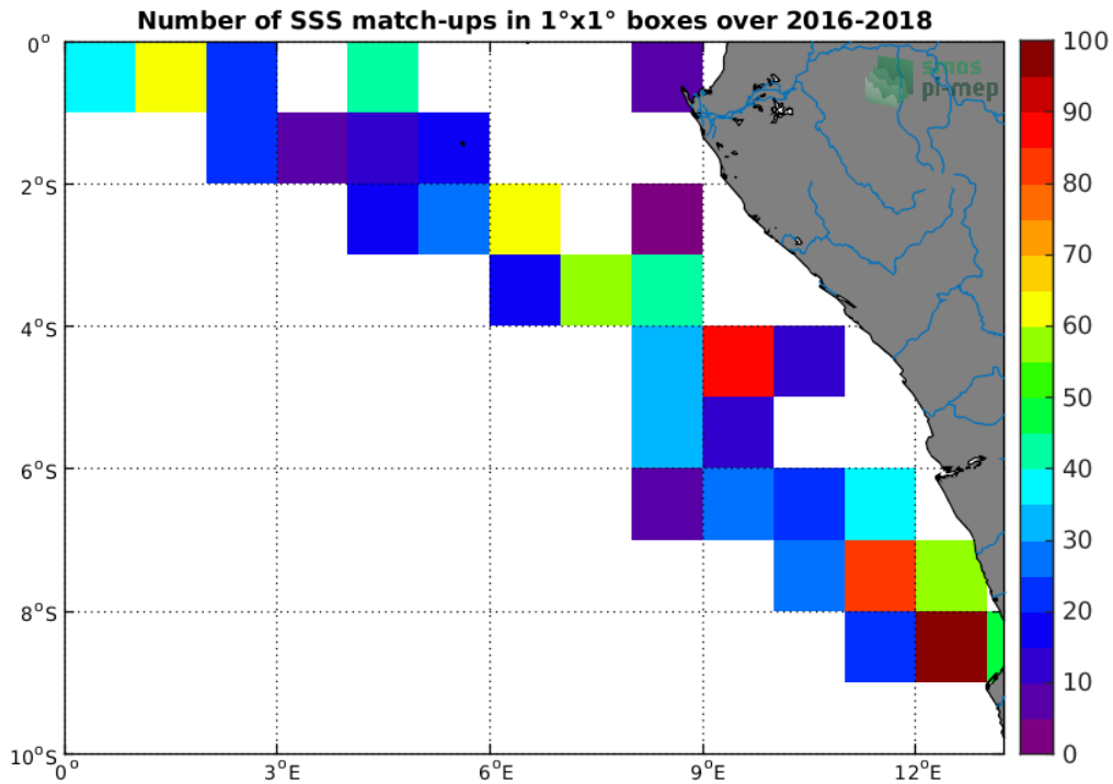
Figure 4: Number of SSS match-ups between TSG-LEGOS-DM SSS and the SMOS-L2-DPGS-v662 SSS product for the Congo river plume Pi-MEP region over 1°x1° boxes and for the full satellite product period.
