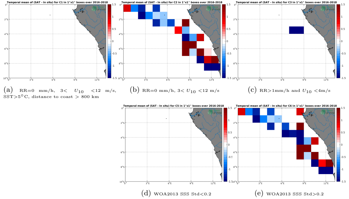
Figure 12: Temporal mean gridded over spatial boxes of size 1^\circ \times 1^\circ of \Delta SSS (SMOS-L2-DPGS-v662 - TSG-LEGOS-DM) for 5 different subdatasets corresponding to:RR=0 mm/h, 3 < U_{10} < 12 m/s, SST >5^\circ\text{C} , distance to coast > 800 km (a), RR=0 mm/h, 3 < U_{10} < 12 m/s (b), RR >1 mm/h and U_{10} < 4 m/s (c), WOA2013 SSS Std <0.2 (d), WOA2013 SSS Std >0.2 (e).
