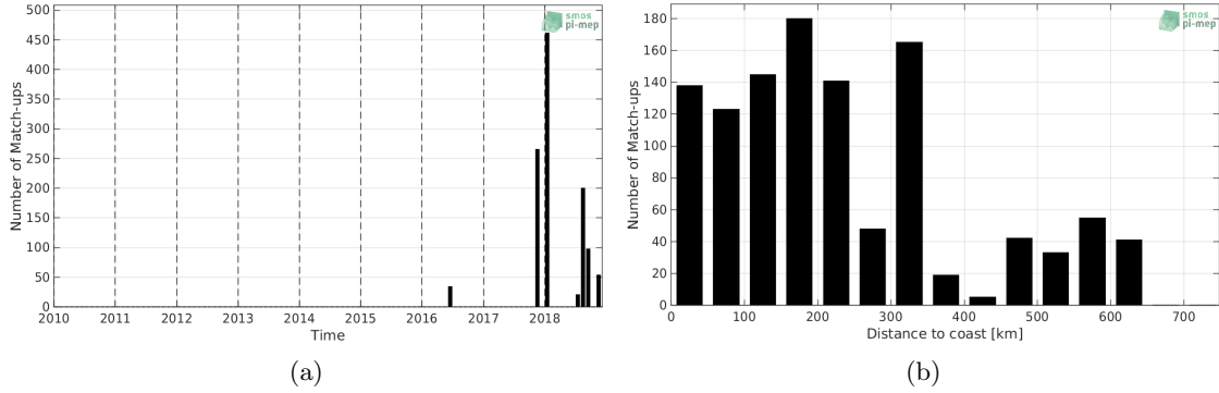
Figure 1: Number of match-ups between TSG-LEGOS-DM and SMOS-L2-DPGS-v662 SSS as a function of time (a) and as function of the distance to coast (b) over the Congo river plume Pi-MEP region and for the full satellite product period.
