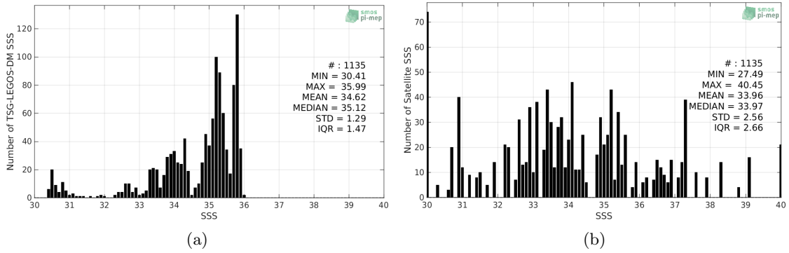
Figure 2: Histograms of SSS from TSG-LEGOS-DM (a) and SMOS-L2-DPGS-v662 (b) considering all match-up pairs per bins of 0.1 over the Congo river plume Pi-MEP region and for the full satellite product period.
