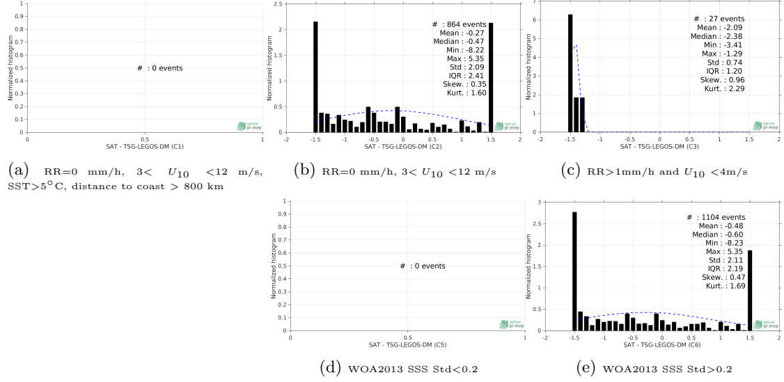
Figure 13: Normalized histogram of \Delta\text{SSS} (SMOS-L2-DPGS-v662 - TSG-LEGOS-DM) for 5 different subdatasets corresponding to: RR=0 mm/h, 3 < U_{10} < 12 m/s, SST > 5^\circ\text{C} , distance to coast > 800 km (a), RR=0 mm/h, 3 < U_{10} < 12 m/s (b), RR > 1 mm/h and U_{10} < 4 m/s (c), WOA2013 SSS Std < 0.2 (d), WOA2013 SSS Std > 0.2 (e).
