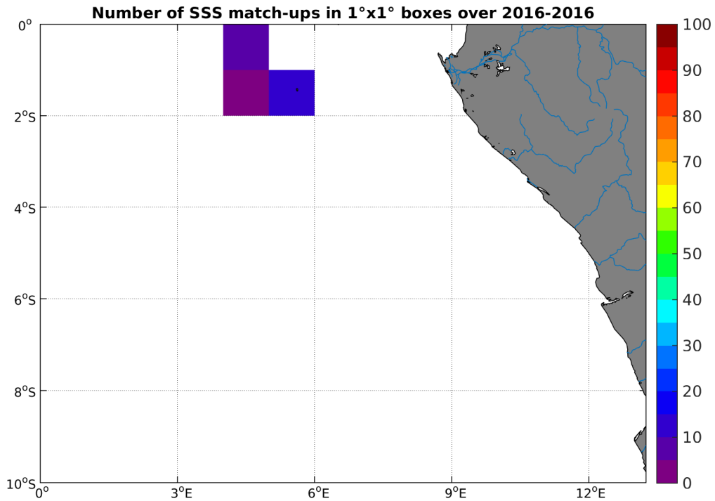
Figure 4: Number of SSS match-ups between TSG-LEGOS-DM SSS and the SMOS-L2-DPGS-v662 SSS product for the Congo river plume Pi-MEP region over 1^\circ \times 1^\circ boxes and for the full satellite product period.
