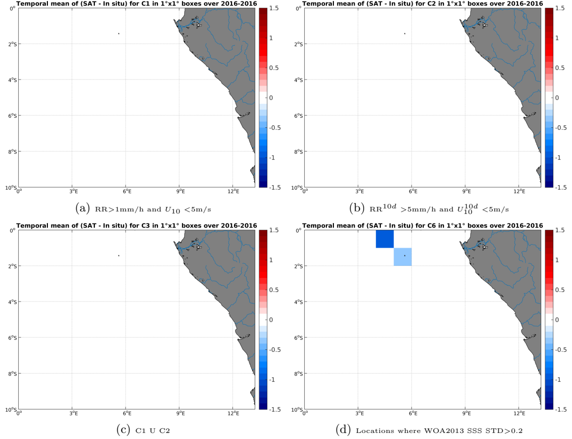
Figure 12: Temporal mean gridded over spatial boxes of size 1^\circ \times 1^\circ of \Delta SSS (SMOS-L2-DPGS-v662 - TSG-LEGOS-DM) for 4 different subdatasets corresponding to: RR > 1\text{mm/h} and U_{10} < 5\text{m/s} (a), RR^{10d} > 5\text{mm/h} and U_{10}^{10d} < 5\text{m/s} (b), C1 \cup C2 (c), Locations where WOA2013 SSS STD > 0.2 (d).
