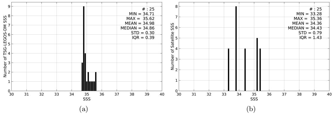
Figure 2: Histograms of SSS from TSG-LEGOS-DM (a) and SMOS-L2-DPGS-v662 (b) considering all match-up pairs per bins of 0.1 over the Congo river plume Pi-MEP region and for the full satellite product period.
