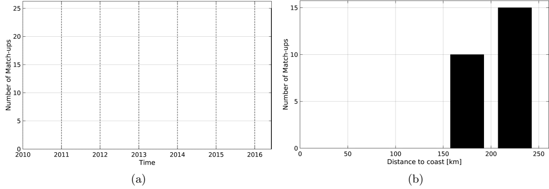
Figure 1: Number of match-ups between TSG-LEGOS-DM and SMOS-L2-DPGS-v662 SSS as a function of time (a) and as function of the distance to coast (b) over the Congo river plume Pi-MEP region and for the full satellite product period.
