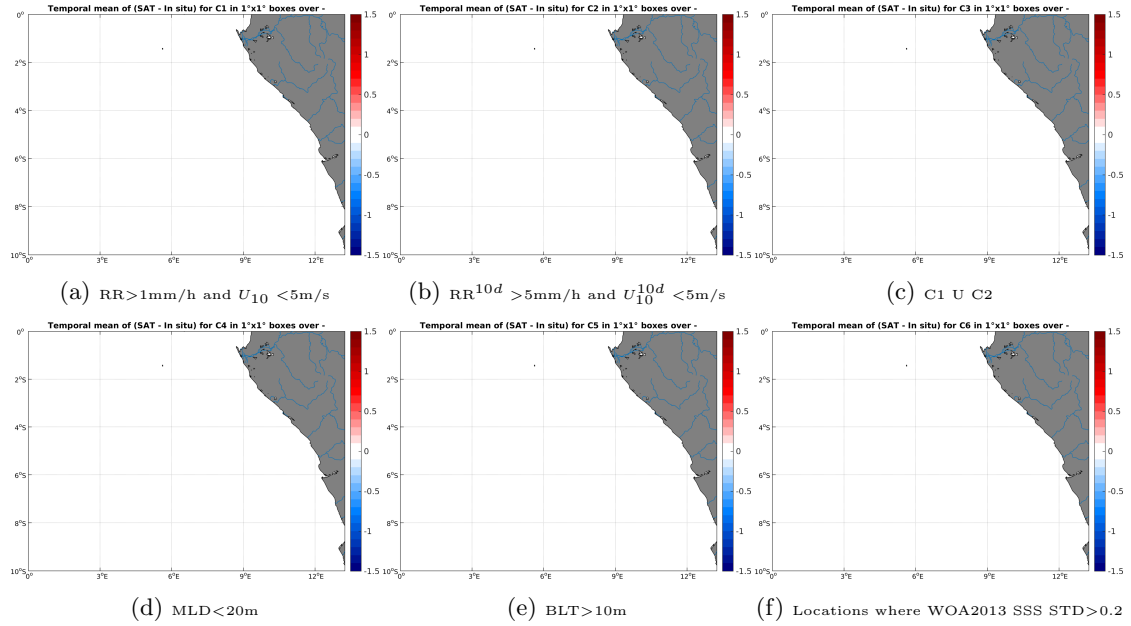
Figure 12: Temporal mean gridded over spatial boxes of size 1^\circ \times 1^\circ of \Delta SSS (SMOS-L2-DPGS-v662 - Sea mammals) for 6 different subdatasets corresponding to: RR > 1mm/h and U_{10} < 5\text{m/s} (a), RR^{10d} > 5\text{mm/h} and U_{10}^{10d} < 5\text{m/s} (b), C1 U C2 (c), MLD < 20m (d), BLT > 10m (e), Locations where WOA2013 SSS STD > 0.2 (f).
