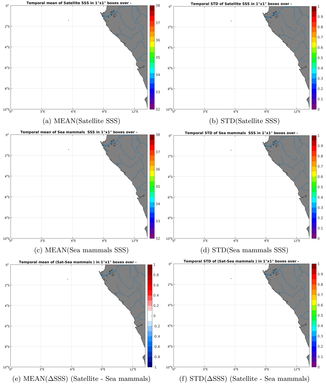
Figure 6: Temporal mean (left) and STD (right) of SSS from SMOS-L2-DPGS-v662 (top), Sea mammals (middle), and of \Delta SSS (Satellite - Sea mammals). Only match-up pairs are used to generate these maps.
