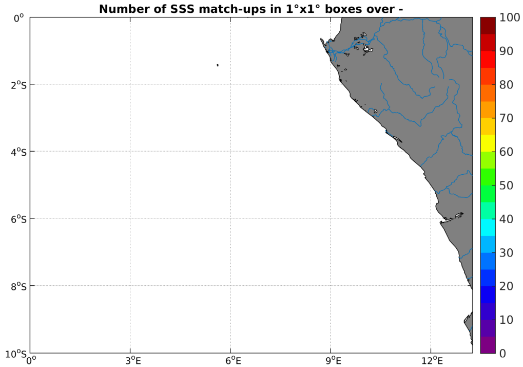
Figure 3: Number of SSS match-ups between Surface drifters SSS and the SMOS-L2-DPGS-v662 SSS product for the Congo river plume Pi-MEP region over 1°x1° boxes and for the full satellite product period.
