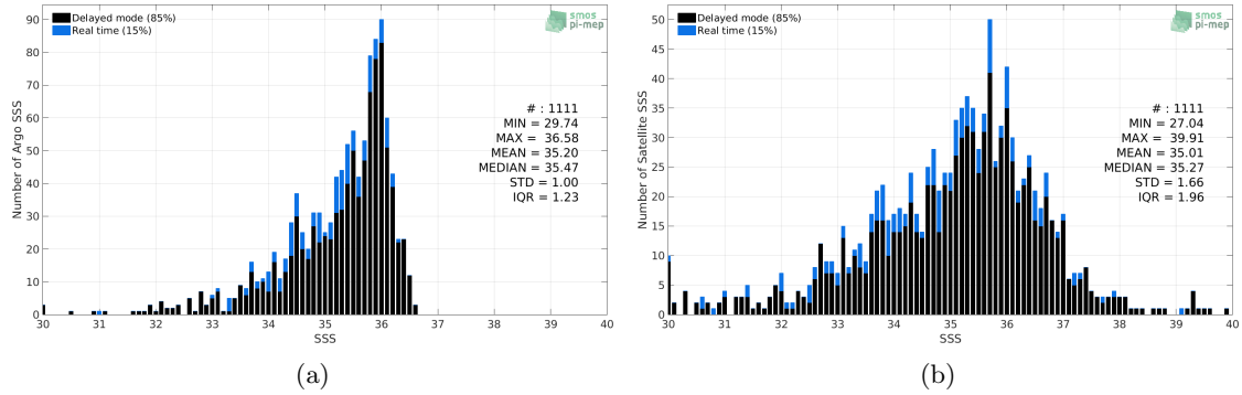
Figure 2: Histograms of SSS from Argo (a) and SMOS SSS L2 v662 (ESA) (b) considering all match-up pairs per bins of 0.1 over the Congo river plume Pi-MEP region and for the full satellite product period.
