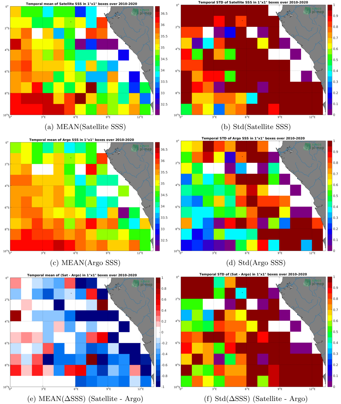
Figure 6: Temporal mean (left) and Std (right) of SSS from SMOS SSS L2 v662 (ESA) (top), Argo (middle), and of \Delta SSS (Satellite - Argo). Only match-up pairs are used to generate these maps.
