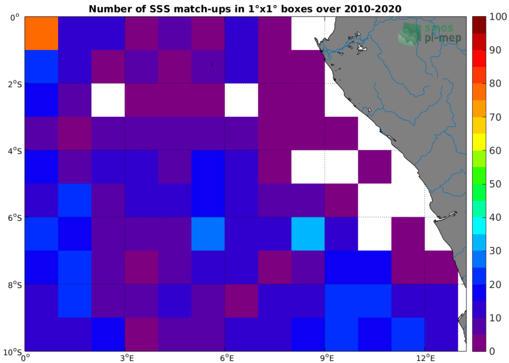
Figure 4: Number of SSS match-ups between Argo SSS and the SMOS SSS L2 v662 (ESA) SSS product for the Congo river plume Pi-MEP region over 1°x1° boxes and for the full satellite product period.
