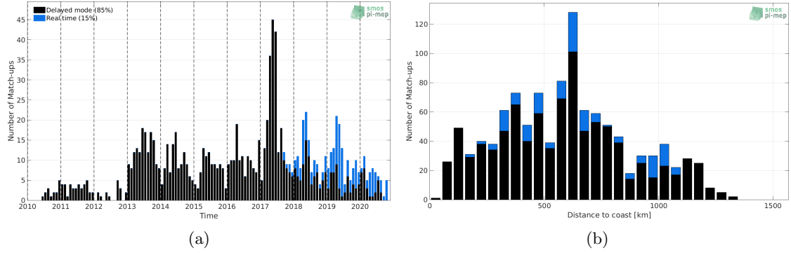
Figure 1: Number of match-ups between Argo and SMOS SSS L2 v662 (ESA) SSS as a function of time (a) and as function of the distance to coast (b) over the Congo river plume Pi-MEP region and for the full satellite product period.
