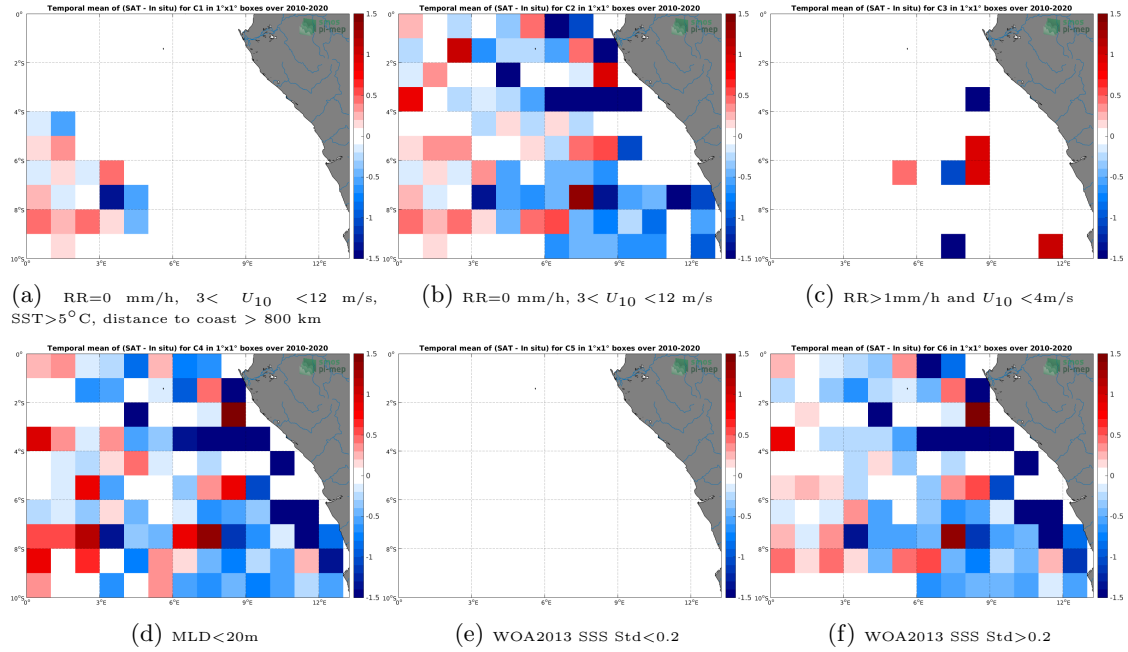
Figure 12: Temporal mean gridded over spatial boxes of size 1^\circ \times 1^\circ of \Delta SSS (SMOS SSS L2 v662 (ESA) - Argo) for 6 different subdatasets corresponding to: RR=0 mm/h, 3 < U_{10} < 12 m/s, SST > 5^\circ C , distance to coast > 800 km (a), RR=0 mm/h, 3 < U_{10} < 12 m/s (b), RR > 1 mm/h and U_{10} < 4 m/s (c), MLD < 20 m (d), WOA2013 SSS Std < 0.2 (e), WOA2013 SSS Std > 0.2 (f).
