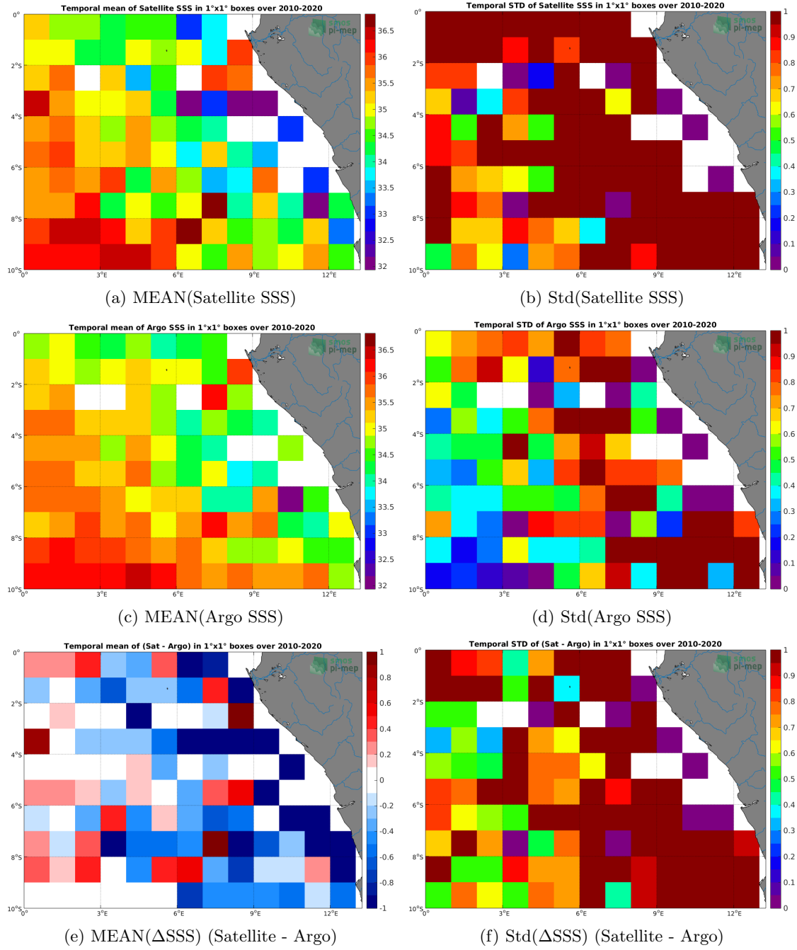
Figure 6: Temporal mean (left) and Std (right) of SSS from SMOS L2 v662 (ESA) (top), Argo (middle), and of \Delta SSS (Satellite - Argo). Only match-up pairs are used to generate these maps.
