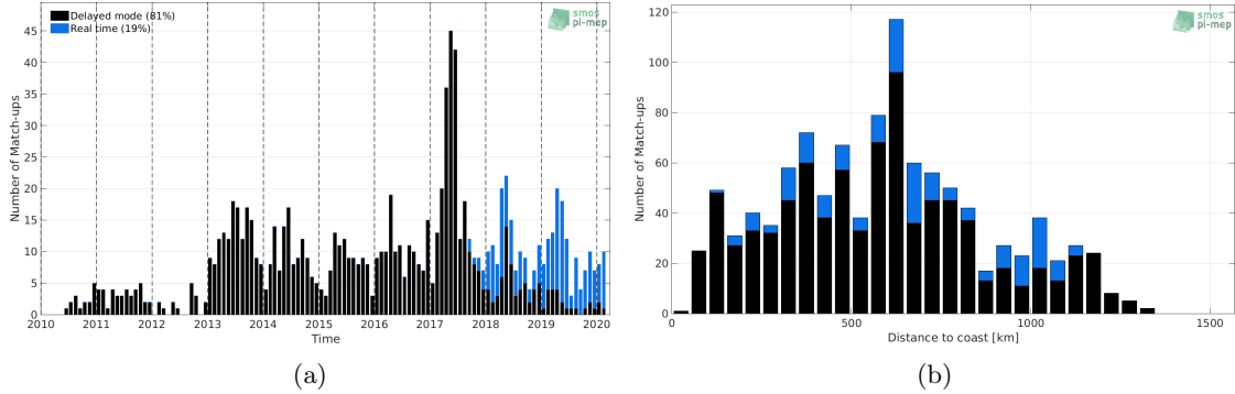
Figure 1: Number of match-ups between Argo and SMOS L2 v662 (ESA) SSS as a function of time (a) and as function of the distance to coast (b) over the Congo river plume Pi-MEP region and for the full satellite product period.
