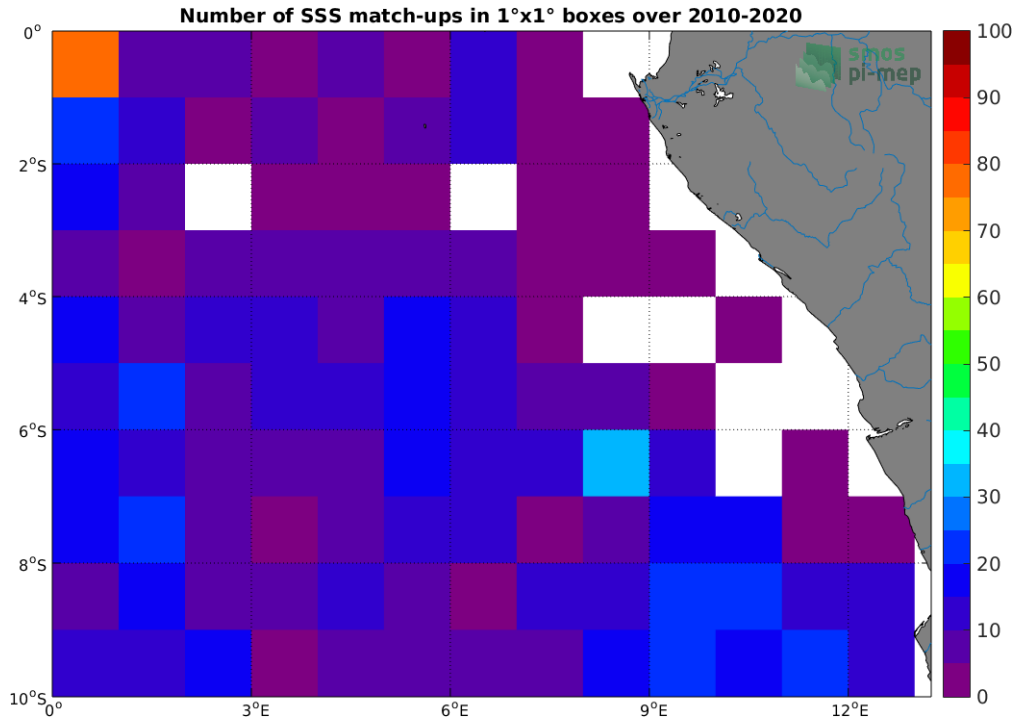
Figure 4: Number of SSS match-ups between Argo SSS and the SMOS L2 v662 (ESA) SSS product for the Congo river plume Pi-MEP region over 1°x1° boxes and for the full satellite product period.
