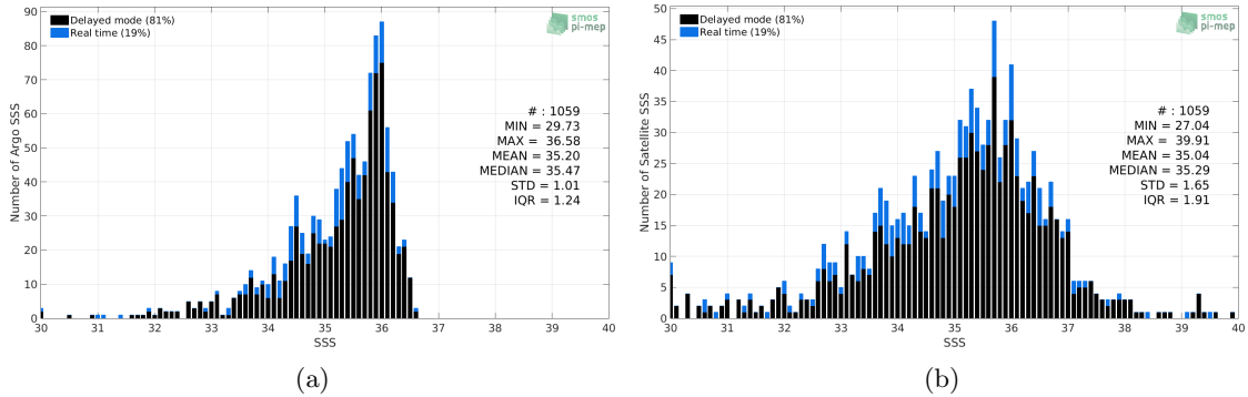
Figure 2: Histograms of SSS from Argo (a) and SMOS L2 v662 (ESA) (b) considering all match-up pairs per bins of 0.1 over the Congo river plume Pi-MEP region and for the full satellite product period.
