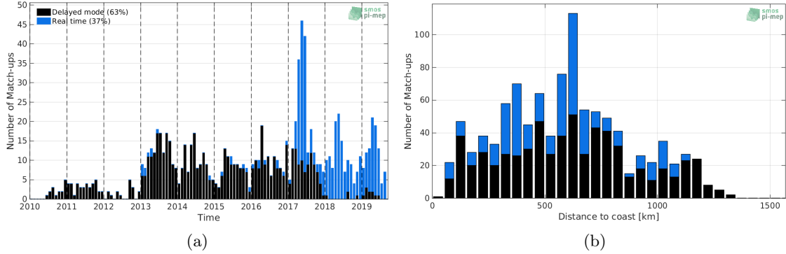
Figure 1: Number of match-ups between Argo and SMOS-L2-DPGS-v662 SSS as a function of time (a) and as function of the distance to coast (b) over the Congo river plume Pi-MEP region and for the full satellite product period.
