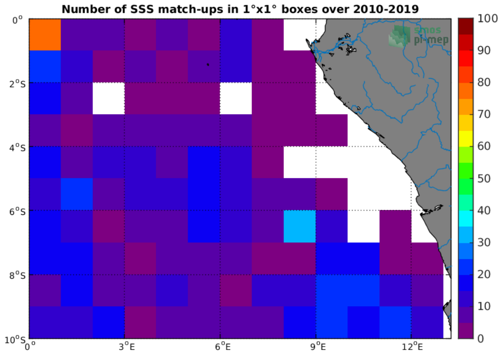
Figure 4: Number of SSS match-ups between Argo SSS and the SMOS-L2-DPGS-v662 SSS product for the Congo river plume Pi-MEP region over 1°x1° boxes and for the full satellite product period.
