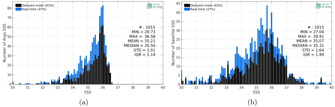
Figure 2: Histograms of SSS from Argo (a) and SMOS-L2-DPGS-v662 (b) considering all match-up pairs per bins of 0.1 over the Congo river plume Pi-MEP region and for the full satellite product period.
