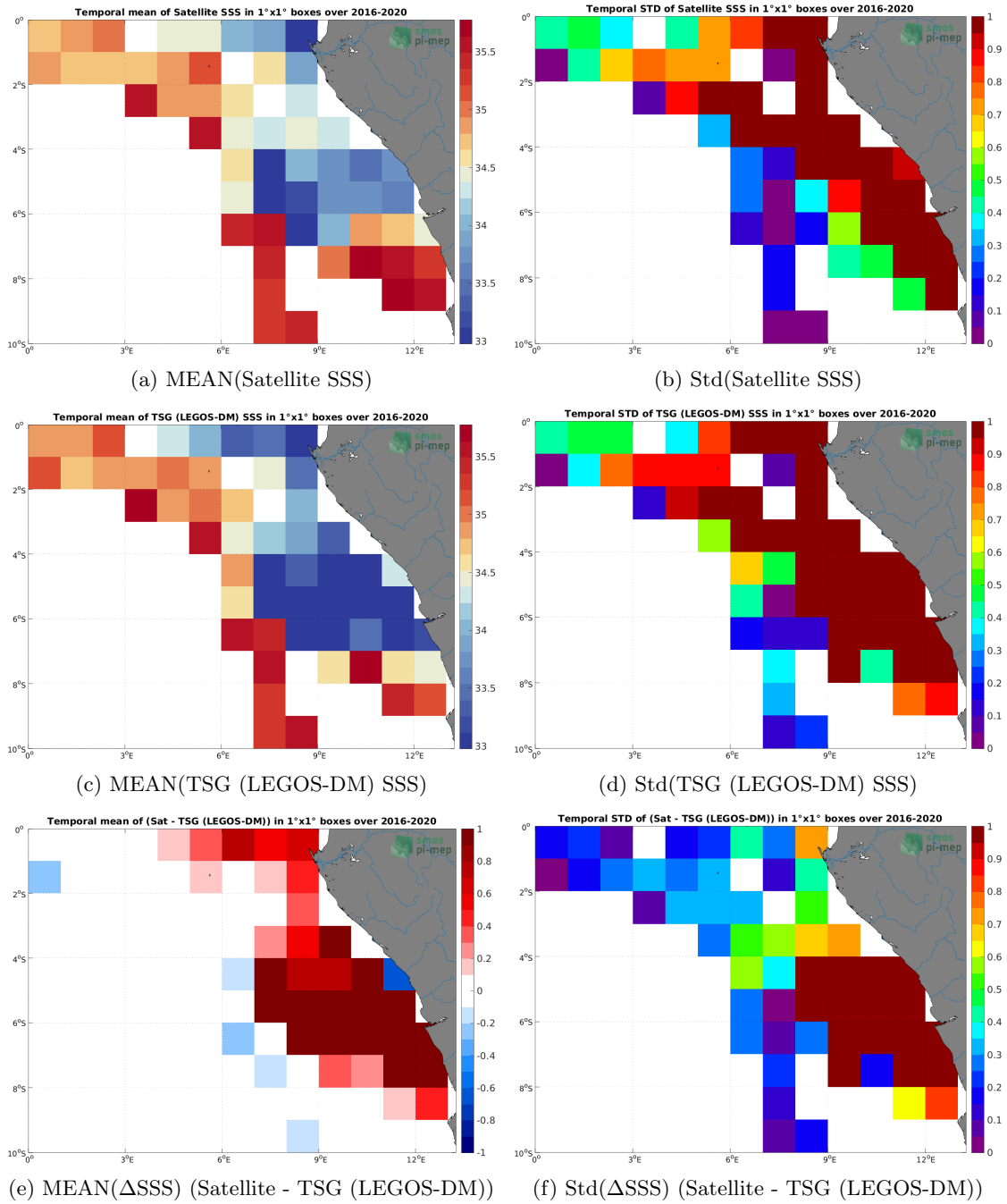
Figure 6: Temporal mean (left) and Std (right) of SSS from SMAP SSS L4 OI v1 - 7 Days (IPRC) (top), TSG (LEGOS-DM) (middle), and of \Delta SSS (Satellite - TSG (LEGOS-DM)). Only match-up pairs are used to generate these maps.
