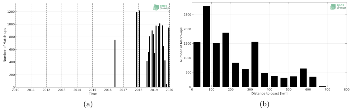
Figure 1: Number of match-ups between TSG (LEGOS-DM) and SMAP SSS L4 OI v1 - 7 Days (IPRC) SSS as a function of time (a) and as function of the distance to coast (b) over the Congo river plume Pi-MEP region and for the full satellite product period.
