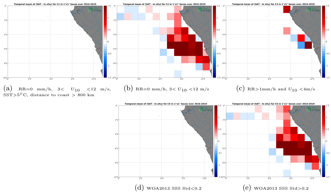
Figure 12: Temporal mean gridded over spatial boxes of size 1^\circ \times 1^\circ of \Delta SSS (SMAP SSS L4 OI v1 - 7 Days (IPRC) - TSG (LEGOS-DM)) for 5 different subdatasets corresponding to:RR=0 mm/h, 3 < U_{10} < 12 m/s, SST > 5°C, distance to coast > 800 km (a), RR=0 mm/h, 3 < U_{10} < 12 m/s (b), RR > 1mm/h and U_{10} < 4 m/s (c), WOA2013 SSS Std < 0.2 (d), WOA2013 SSS Std > 0.2 (e).
