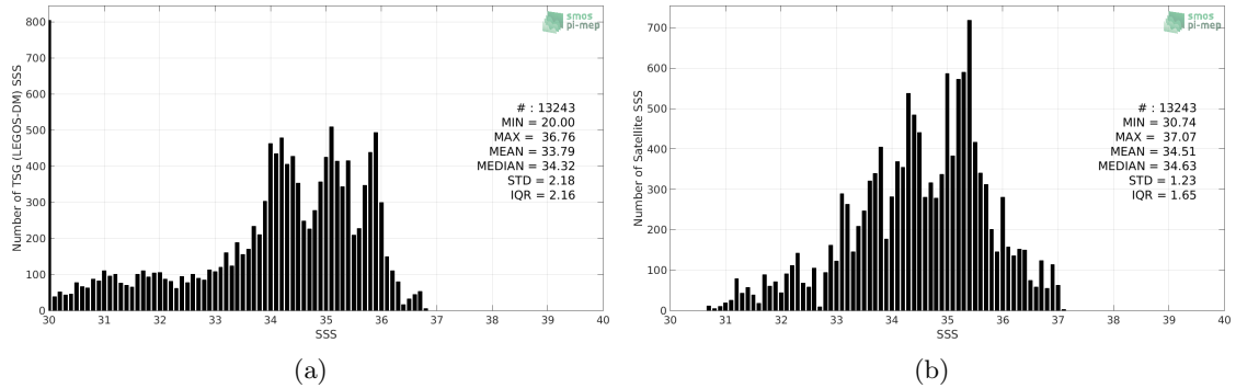
Figure 2: Histograms of SSS from TSG (LEGOS-DM) (a) and SMAP SSS L4 OI v1 - 7 Days (IPRC) (b) considering all match-up pairs per bins of 0.1 over the Congo river plume Pi-MEP region and for the full satellite product period.
