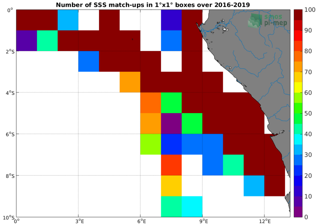
Figure 4: Number of SSS match-ups between TSG (LEGOS-DM) SSS and the SMAP SSS L4 OI v1 - 7 Days (IPRC) SSS product for the Congo river plume Pi-MEP region over 1^\circ \times 1^\circ boxes and for the full satellite product period.
