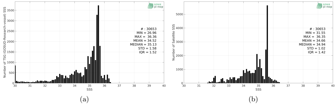
Figure 2: Histograms of SSS from TSG (GOSUD-Research-vessel) (a) and SMAP SSS L4 OI v1 - 7 Days (IPRC) (b) considering all match-up pairs per bins of 0.1 over the Congo river plume Pi-MEP region and for the full satellite product period.
