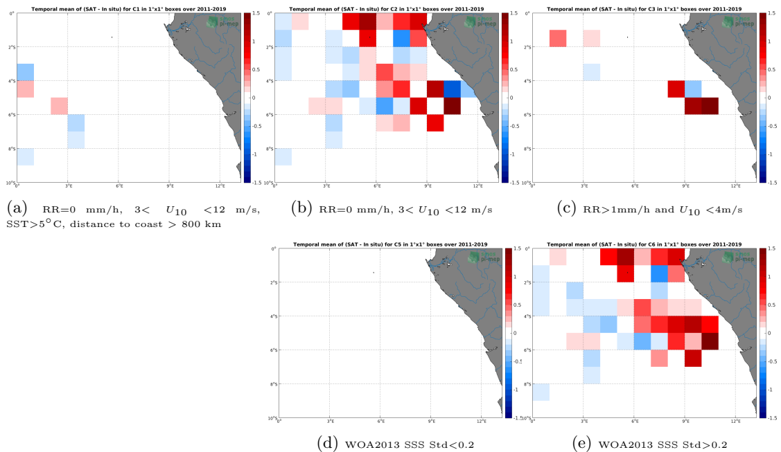
Figure 12: Temporal mean gridded over spatial boxes of size 1^\circ \times 1^\circ of \Delta SSS (SMAP SSS L4 OI v1 - 7 Days (IPRC) - TSG (GOSUD-Research-vessel)) for 5 different subdatasets corresponding to:RR=0 mm/h, 3 < U_{10} < 12 m/s, SST>5°C, distance to coast > 800 km (a), RR=0 mm/h, 3 < U_{10} < 12 m/s (b), RR>1mm/h and U_{10} < 4 m/s (c), WOA2013 SSS Std<0.2 (d), WOA2013 SSS Std>0.2 (e).
