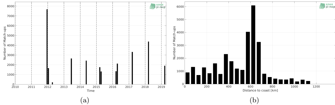
Figure 1: Number of match-ups between TSG (GOSUD-Research-vessel) and SMAP SSS L4 OI v1 - 7 Days (IPRC) SSS as a function of time (a) and as function of the distance to coast (b) over the Congo river plume Pi-MEP region and for the full satellite product period.
