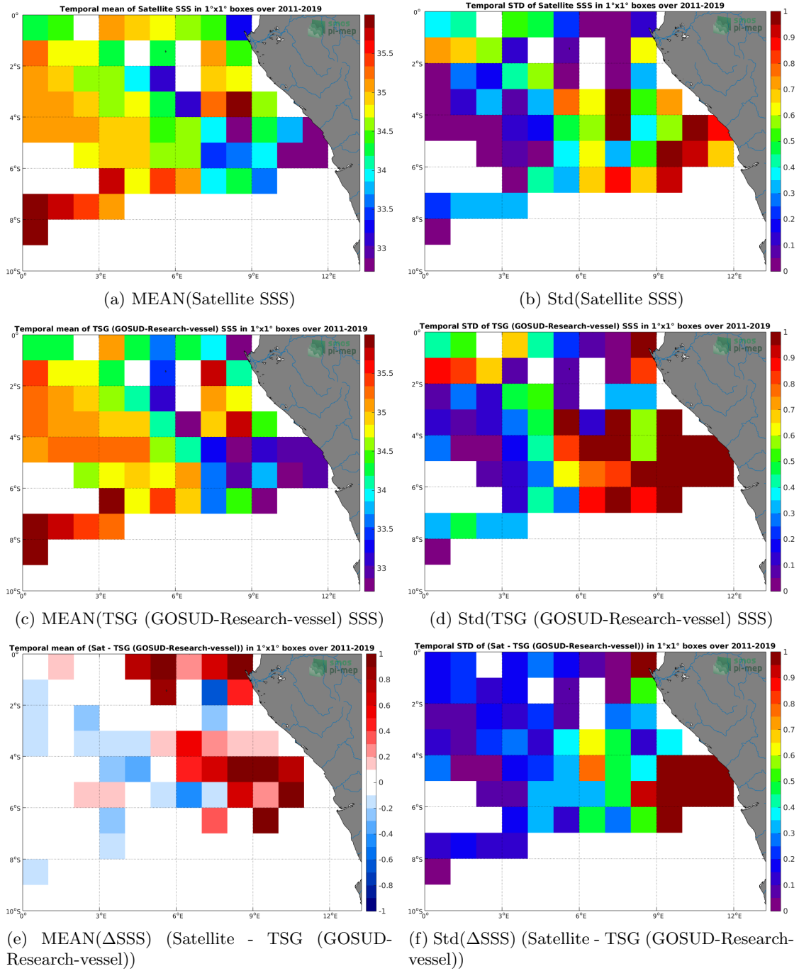
Figure 6: Temporal mean (left) and Std (right) of SSS from SMAP SSS L4 OI v1 - 7 Days (IPRC) (top), TSG (GOSUD-Research-vessel) (middle), and of \Delta SSS (Satellite - TSG (GOSUD-Research-vessel)). Only match-up pairs are used to generate these maps.
