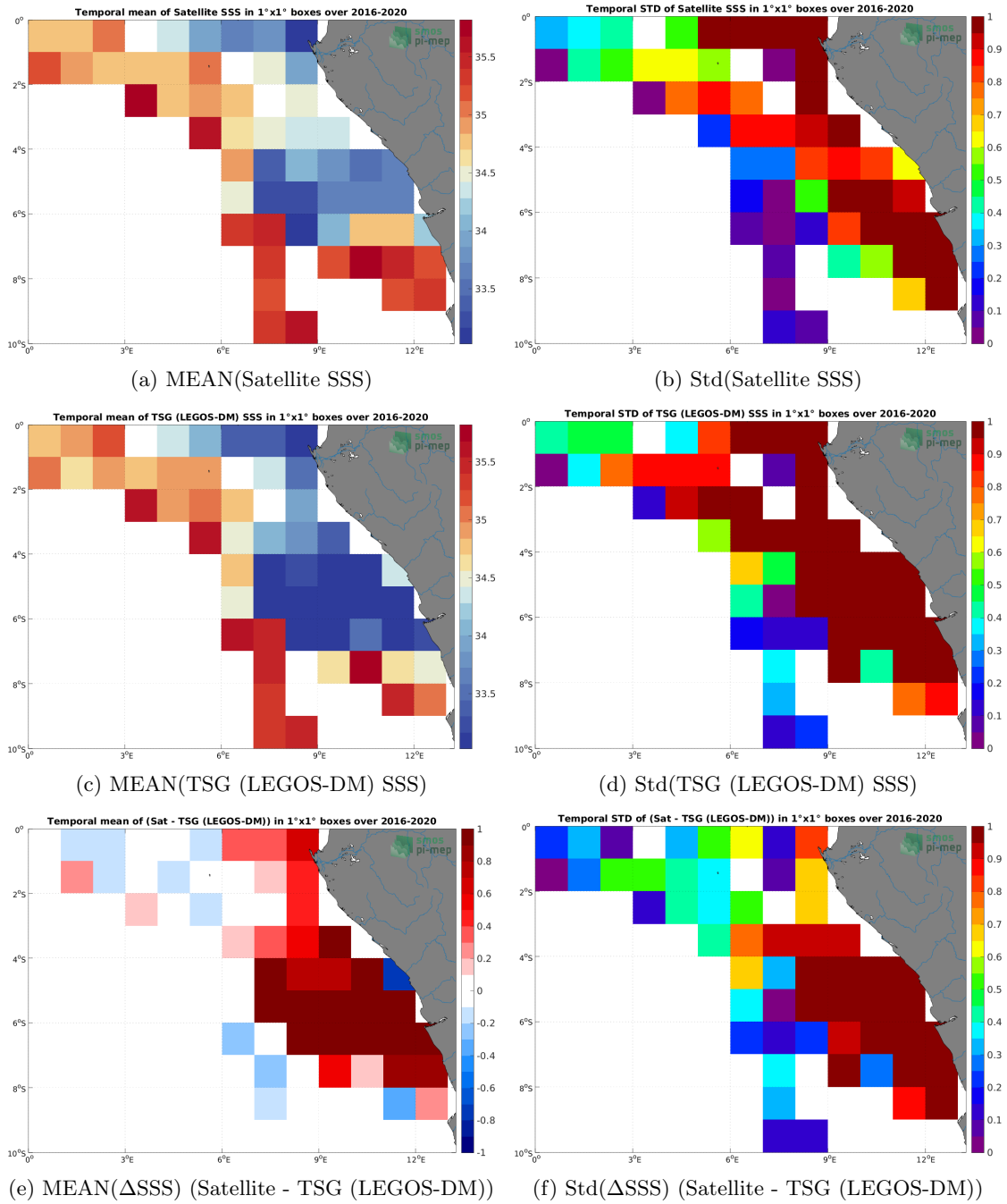
Figure 6: Temporal mean (left) and Std (right) of SSS from SMAP SSS L4 OI v1 - Monthly (IPRC) (top), TSG (LEGOS-DM) (middle), and of \Delta SSS (Satellite - TSG (LEGOS-DM)). Only match-up pairs are used to generate these maps.
