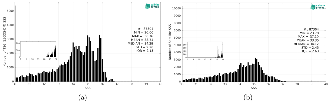
Figure 3: Histograms of SSS from TSG (LEGOS-DM) (a) and SMAP SSS L4 OI v3 - Daily (ESR) (b) considering all match-up pairs per bins of 0.1 over the Congo river plume Pi-MEP region and for the full satellite product period.
