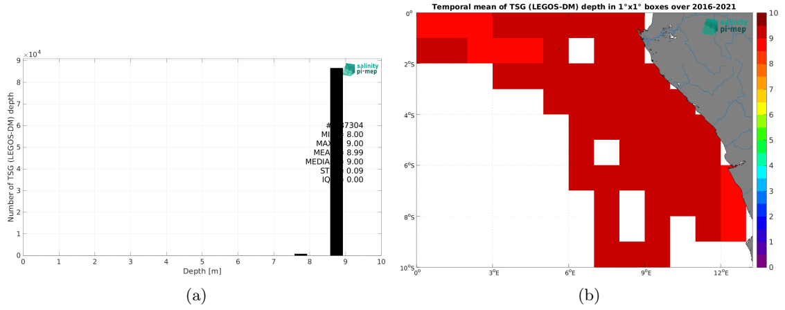
Figure 4: Histograms of the depth of the upper level SSS measurements from TSG (LEGOS-DM) in the Match-up DataBase for the Congo river plume Pi-MEP region (a) and temporal mean spatial distribution of pressure of the in situ SSS data over 1^\circ \times 1^\circ boxes and for the full satellite product period (b).
