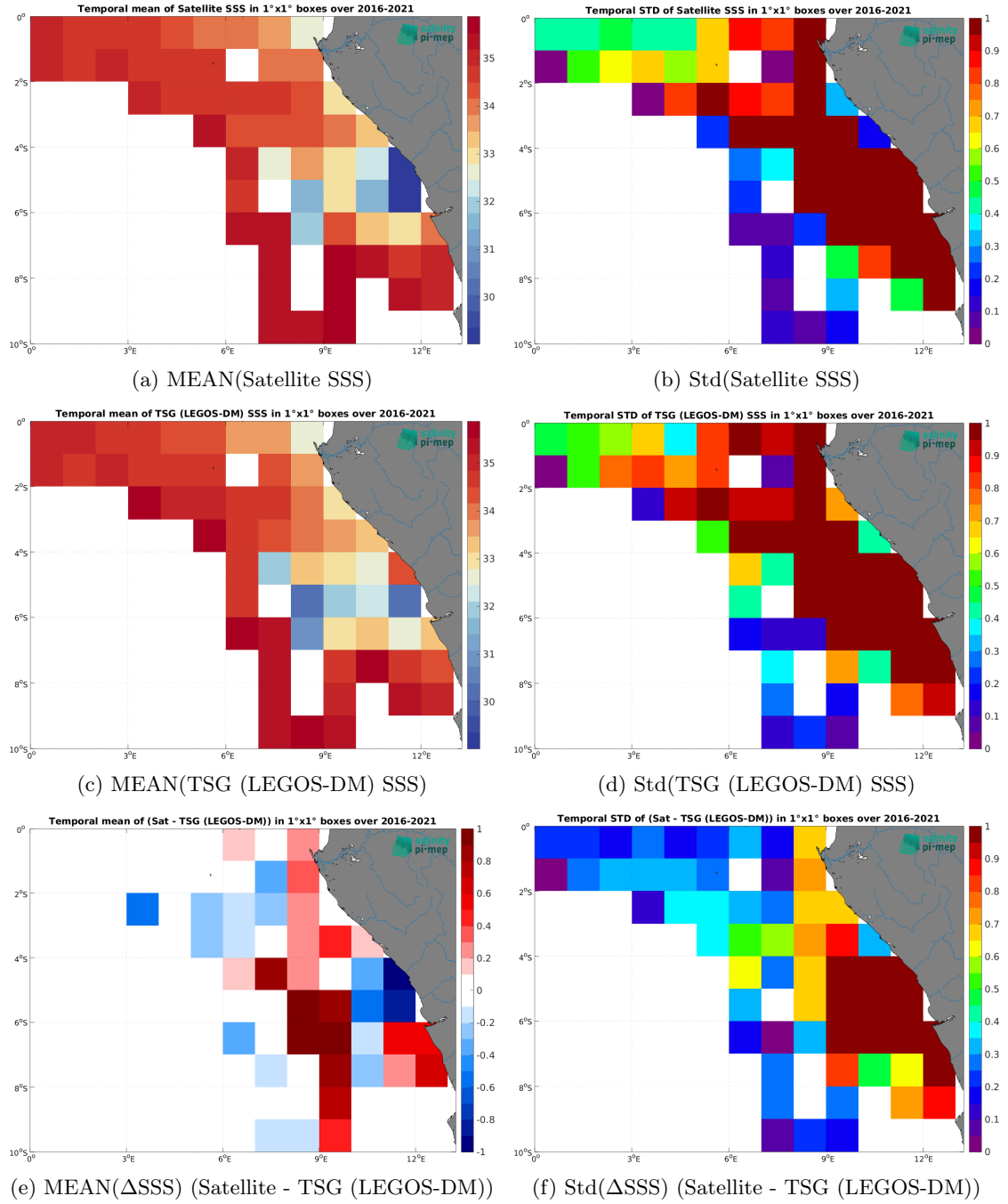
Figure 7: Temporal mean (left) and Std (right) of SSS from SMAP SSS L4 OI v3 - Daily (ESR) (top), TSG (LEGOS-DM) (middle), and of \Delta SSS (Satellite - TSG (LEGOS-DM)). Only match-up pairs are used to generate these maps.
