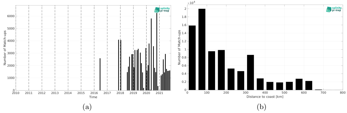
Figure 2: Number of match-ups between TSG (LEGOS-DM) and SMAP SSS L4 OI v3 - Daily (ESR) SSS as a function of time (a) and as function of the distance to coast (b) over the Congo river plume Pi-MEP region and for the full satellite product period.
