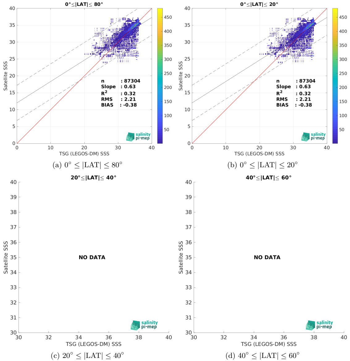
Figure 10: Contour maps of the concentration of SMAP SSS L4 OI v3 - Daily (ESR) SSS (y-axis) versus TSG (LEGOS-DM) SSS (x-axis) at match-up pairs for different latitude bands. For each plot, the red line shows x=y . The black thin and dashed lines indicate a linear fit through the data cloud and the \pm 95\% confidence levels, respectively. The number match-up pairs n , the slope and R^2 coefficient of the linear fit, the root mean square (RMS) and the mean bias between satellite and in situ data are indicated for each latitude band in each plots.
