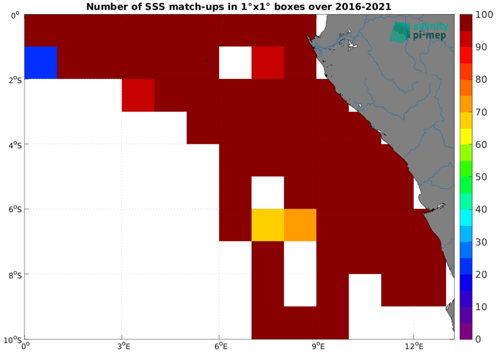
Figure 5: Number of SSS match-ups between TSG (LEGOS-DM) SSS and the SMAP SSS L4 OI v3 - Daily (ESR) SSS product for the Congo river plume Pi-MEP region over 1^\circ \times 1^\circ boxes and for the full satellite product period.
