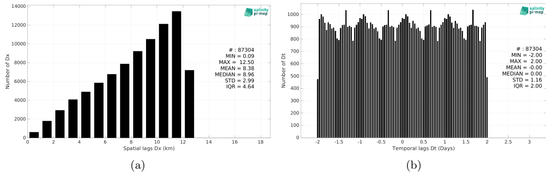
Figure 6: Histograms of the spatial (a) and temporal (b) lags between the location/time of the TSG (LEGOS-DM) measurement and the date of the corresponding SMAP SSS L4 OI v3 - Daily (ESR) SSS pixel.
