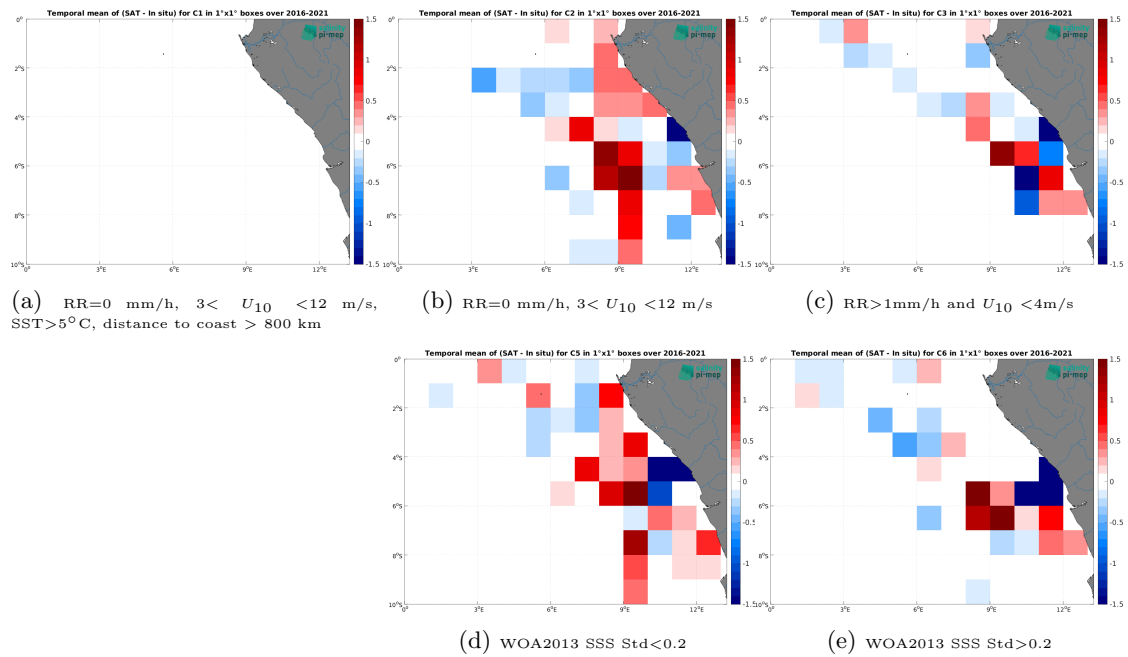
Figure 14: Temporal mean gridded over spatial boxes of size 1^\circ \times 1^\circ of \Delta SSS (SMAP SSS L4 OI v3 - Daily (ESR) - TSG (LEGOS-DM)) for 5 different subdatasets corresponding to:RR=0 mm/h, 3 < U_{10} < 12 m/s, SST >5^\circ\text{C} , distance to coast > 800 km (a), RR=0 mm/h, 3 < U_{10} < 12 m/s (b), RR >1 mm/h and U_{10} < 4 m/s (c), WOA2013 SSS Std <0.2 (d), WOA2013 SSS Std >0.2 (e).
