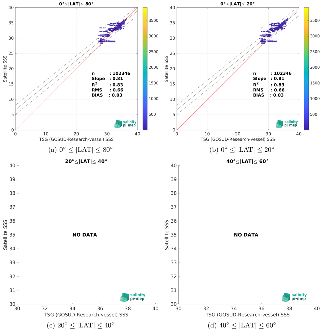
Figure 10: Contour maps of the concentration of SMAP SSS L4 OI v3 - Daily (ESR) SSS (y-axis) versus TSG (GOSUD-Research-vessel) SSS (x-axis) at match-up pairs for different latitude bands. For each plot, the red line shows x=y . The black thin and dashed lines indicate a linear fit through the data cloud and the \pm 95\% confidence levels, respectively. The number match-up pairs n , the slope and R^2 coefficient of the linear fit, the root mean square (RMS) and the mean bias between satellite and in situ data are indicated for each latitude band in each plots.
