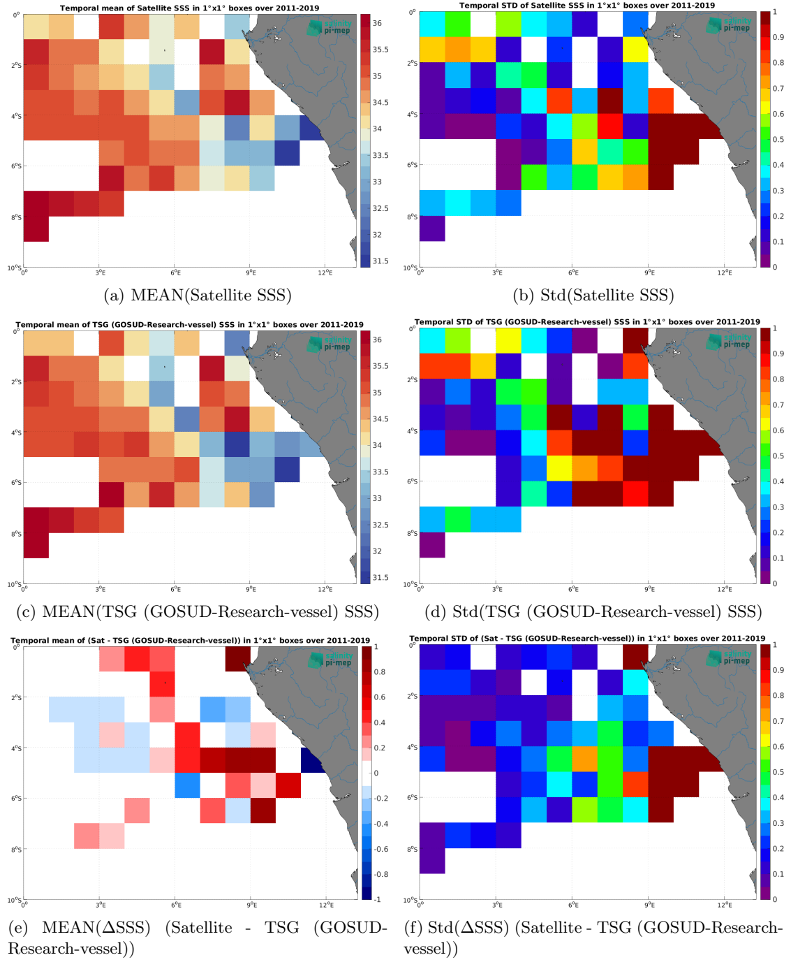
Figure 7: Temporal mean (left) and Std (right) of SSS from SMAP SSS L4 OI v3 - Daily (ESR) (top), TSG (GOSUD-Research-vessel) (middle), and of \Delta SSS (Satellite - TSG (GOSUD-Research-vessel)). Only match-up pairs are used to generate these maps.
