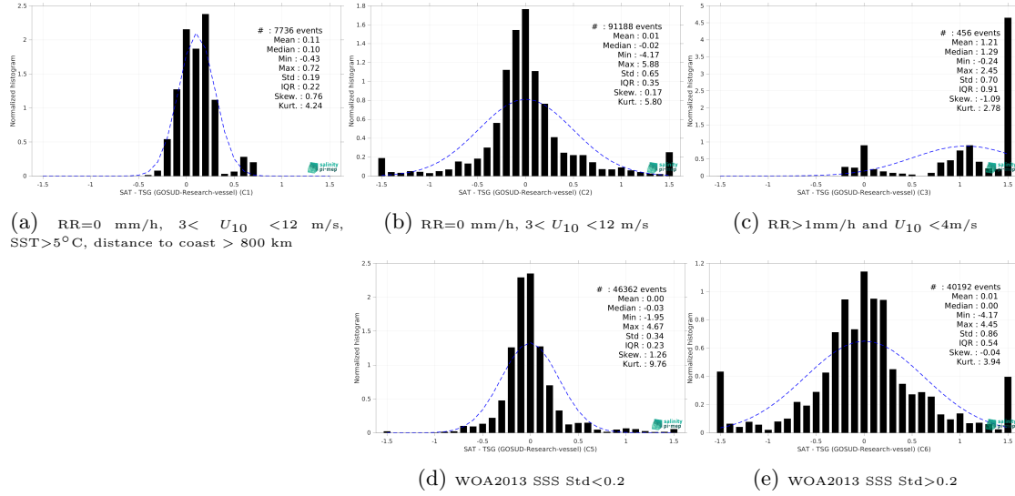
Figure 15: Normalized histogram of \Delta\text{SSS} (SMAP SSS L4 OI v3 - Daily (ESR) - TSG (GOSUD-Research-vessel)) for 5 different subdatasets corresponding to: RR=0 mm/h, 3 < U_{10} < 12 m/s, SST > 5^\circ\text{C} , distance to coast > 800 km (a), RR=0 mm/h, 3 < U_{10} < 12 m/s (b), RR > 1 mm/h and U_{10} < 4 m/s (c), WOA2013 SSS \text{Std} < 0.2 (d), WOA2013 SSS \text{Std} > 0.2 (e).
