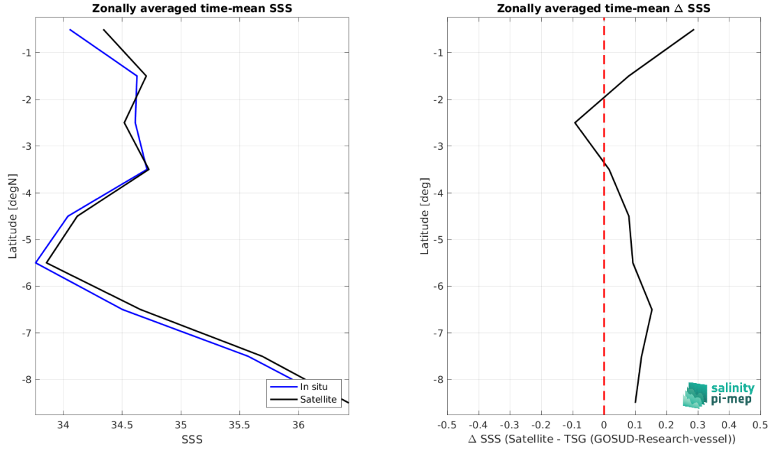
Figure 9: Left panel: Zonal mean SSS from SMAP SSS L4 OI v3 - Daily (ESR) satellite product (black) and from TSG (GOSUD-Research-vessel) (blue). Right panel: Zonal mean of \Delta SSS (Satellite - TSG (GOSUD-Research-vessel)) for all the collected Pi-MEP match-up pairs estimated over the full satellite product period.
