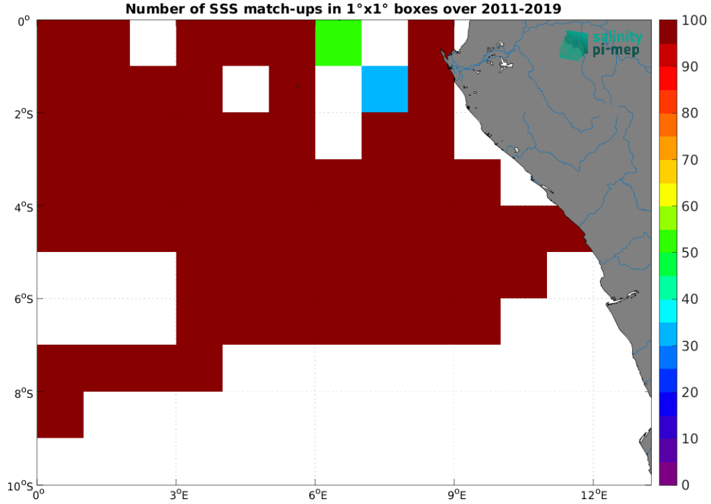
Figure 5: Number of SSS match-ups between TSG (GOSUD-Research-vessel) SSS and the SMAP SSS L4 OI v3 - Daily (ESR) SSS product for the Congo river plume Pi-MEP region over 1^\circ \times 1^\circ boxes and for the full satellite product period.
