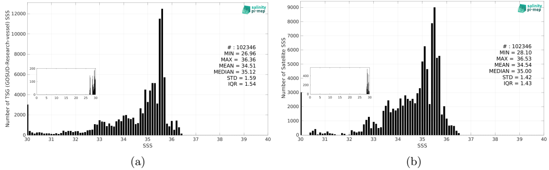
Figure 3: Histograms of SSS from TSG (GOSUD-Research-vessel) (a) and SMAP SSS L4 OI v3 - Daily (ESR) (b) considering all match-up pairs per bins of 0.1 over the Congo river plume Pi-MEP region and for the full satellite product period.
