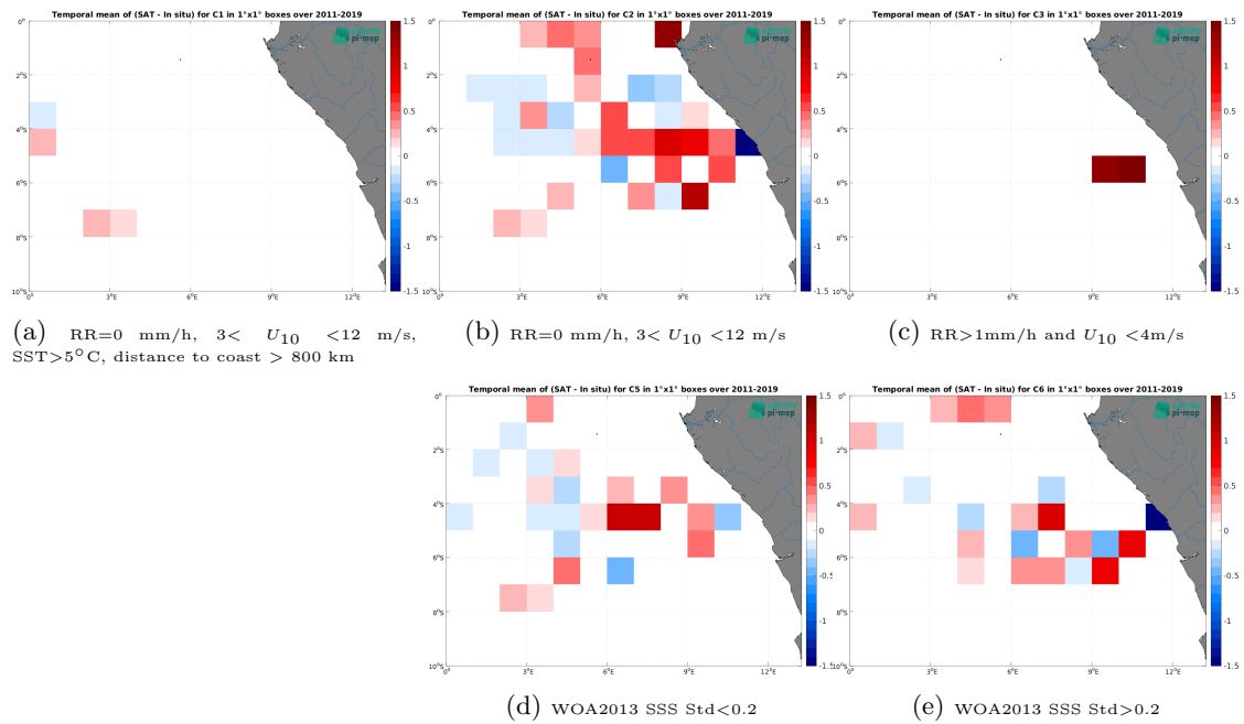
Figure 14: Temporal mean gridded over spatial boxes of size 1^\circ \times 1^\circ of \Delta SSS (SMAP SSS L4 OI v3 - Daily (ESR) - TSG (GOSUD-Research-vessel)) for 5 different subdatasets corresponding to:RR=0 mm/h, 3 < U_{10} < 12 m/s, SST >5^\circ C, distance to coast > 800 km (a), RR=0 mm/h, 3 < U_{10} < 12 m/s (b), RR >1 mm/h and U_{10} < 4 m/s (c), WOA2013 SSS Std <0.2 (d), WOA2013 SSS Std >0.2 (e).
