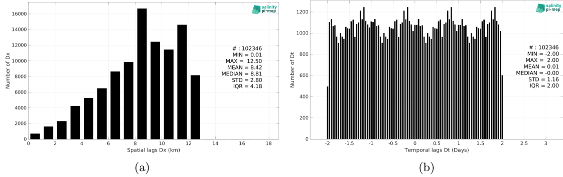
Figure 6: Histograms of the spatial (a) and temporal (b) lags between the location/time of the TSG (GOSUD-Research-vessel) measurement and the date of the corresponding SMAP SSS L4 OI v3 - Daily (ESR) SSS pixel.
