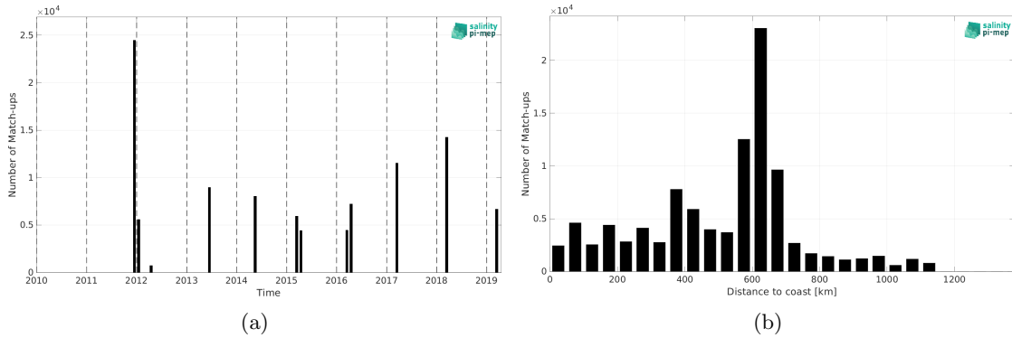
Figure 2: Number of match-ups between TSG (GOSUD-Research-vessel) and SMAP SSS L4 OI v3 - Daily (ESR) SSS as a function of time (a) and as function of the distance to coast (b) over the Congo river plume Pi-MEP region and for the full satellite product period.
