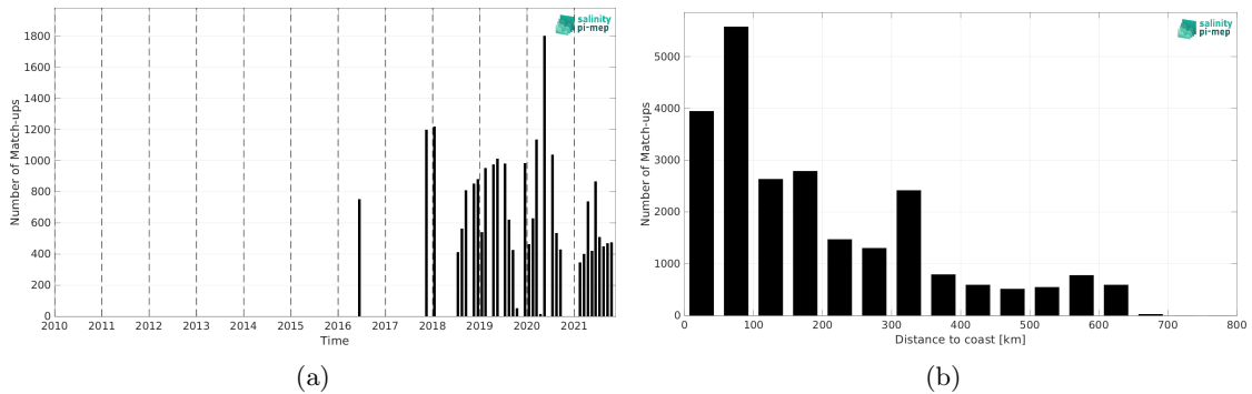
Figure 1: Number of match-ups between TSG (LEGOS-DM) and SMAP SSS L4 OI v2 - 7 Days (ESR) SSS as a function of time (a) and as function of the distance to coast (b) over the Congo river plume Pi-MEP region and for the full satellite product period.
