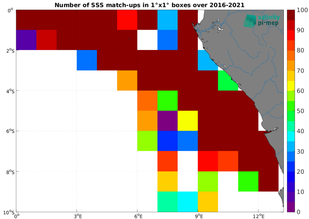
Figure 4: Number of SSS match-ups between TSG (LEGOS-DM) SSS and the SMAP SSS L4 OI v2 - 7 Days (ESR) SSS product for the Congo river plume Pi-MEP region over 1^\circ \times 1^\circ boxes and for the full satellite product period.
