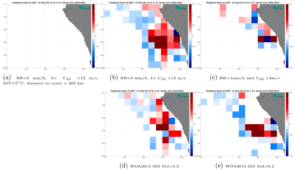
Figure 12: Temporal mean gridded over spatial boxes of size 1^\circ \times 1^\circ of \Delta SSS (SMAP SSS L4 OI v2 - 7 Days (ESR) - TSG (LEGOS-DM)) for 5 different subdatasets corresponding to:RR=0 mm/h, 3 < U_{10} < 12 m/s, SST > 5^\circ C, distance to coast > 800 km (a), RR=0 mm/h, 3 < U_{10} < 12 m/s (b), RR > 1 mm/h and U_{10} < 4 m/s (c), WOA2013 SSS Std < 0.2 (d), WOA2013 SSS Std > 0.2 (e).
