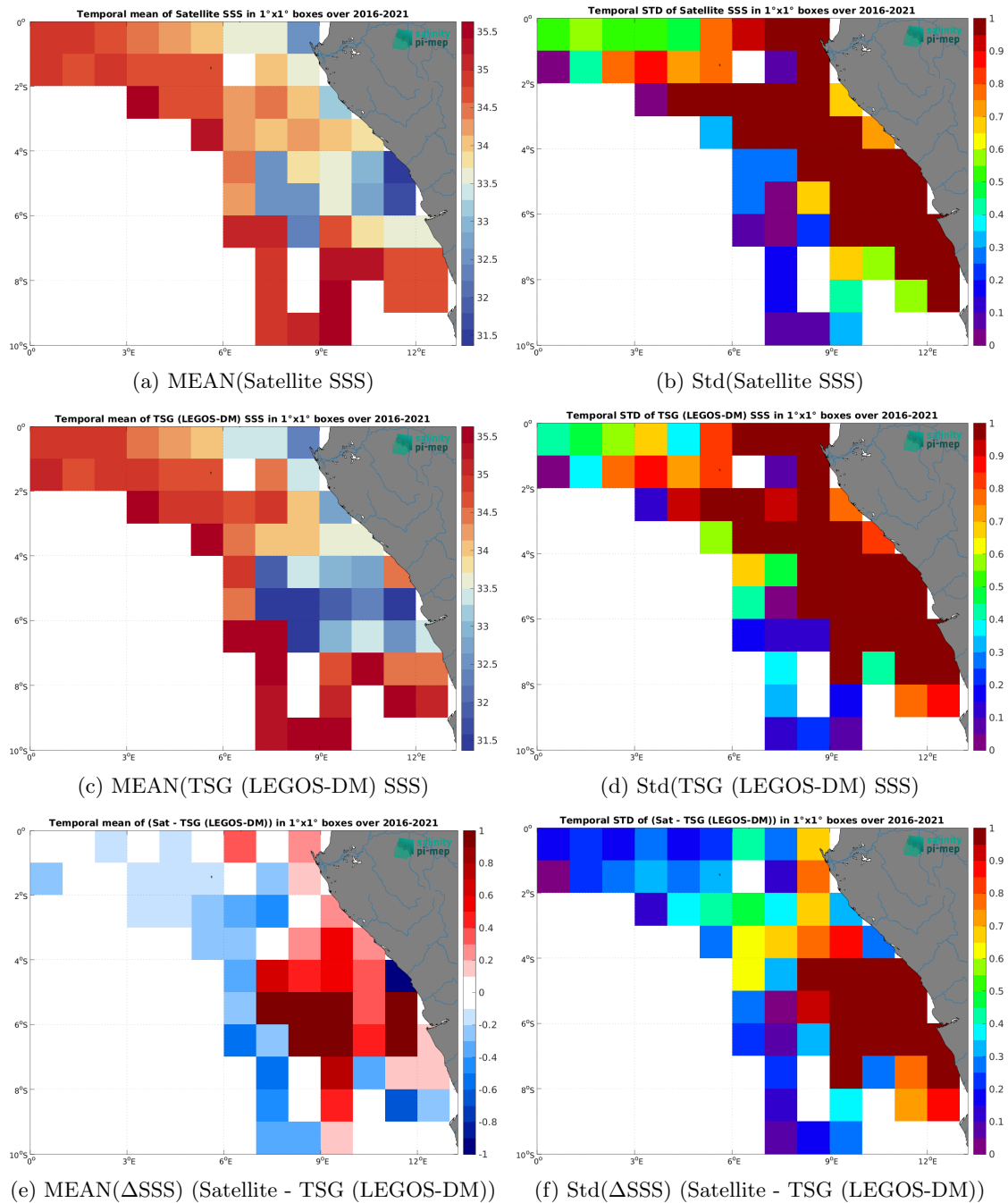
Figure 6: Temporal mean (left) and Std (right) of SSS from SMAP SSS L4 OI v2 - 7 Days (ESR) (top), TSG (LEGOS-DM) (middle), and of \Delta SSS (Satellite - TSG (LEGOS-DM)). Only match-up pairs are used to generate these maps.
