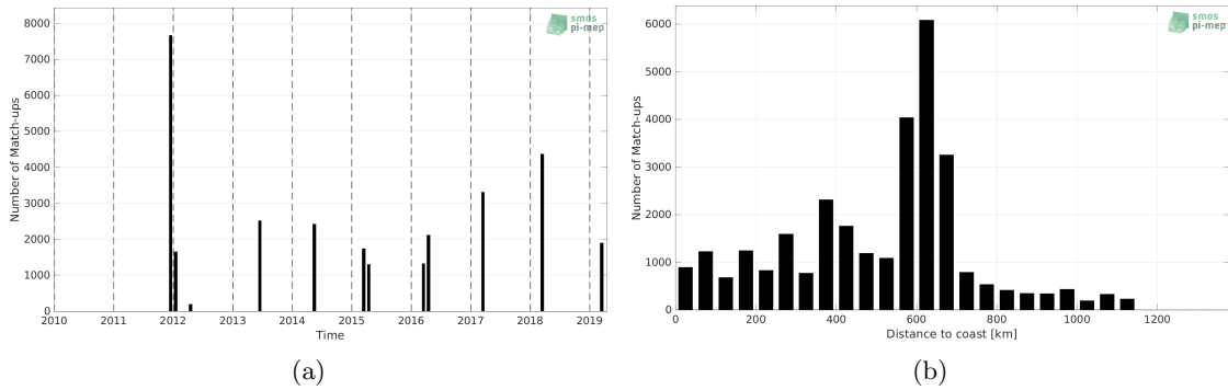
Figure 1: Number of match-ups between TSG (GOSUD-Research-vessel) and SMAP SSS L4 OI v2 - 7 Days (ESR) SSS as a function of time (a) and as function of the distance to coast (b) over the Congo river plume Pi-MEP region and for the full satellite product period.
