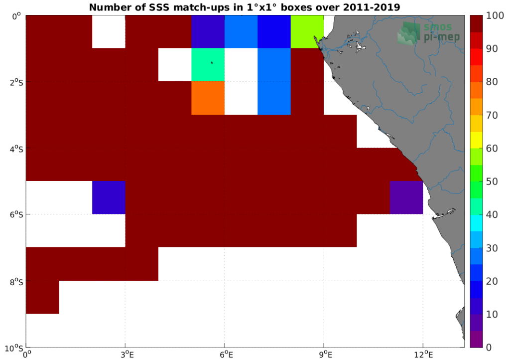
Figure 4: Number of SSS match-ups between TSG (GOSUD-Research-vessel) SSS and the SMAP SSS L4 OI v2 - 7 Days (ESR) SSS product for the Congo river plume Pi-MEP region over 1^\circ \times 1^\circ boxes and for the full satellite product period.
