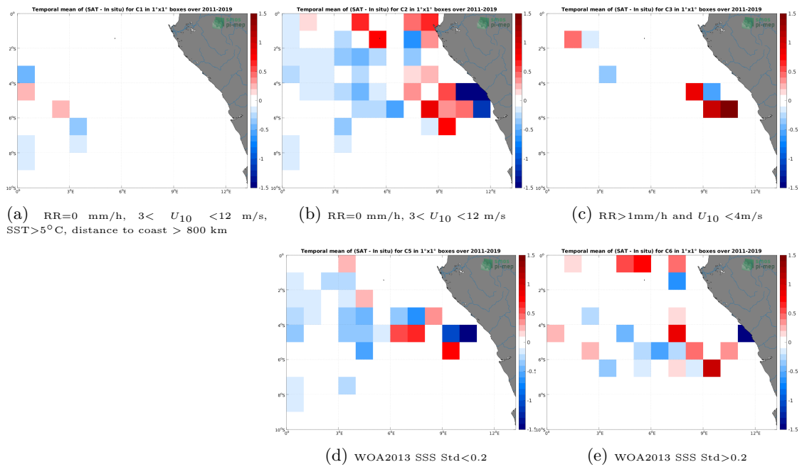
Figure 12: Temporal mean gridded over spatial boxes of size 1^\circ \times 1^\circ of \Delta SSS (SMAP SSS L4 OI v2 - 7 Days (ESR) - TSG (GOSUD-Research-vessel)) for 5 different subdatasets corresponding to: RR=0 mm/h, 3 < U_{10} < 12 m/s, SST > 5°C, distance to coast > 800 km (a), RR=0 mm/h, 3 < U_{10} < 12 m/s (b), RR > 1mm/h and U_{10} < 4 m/s (c), WOA2013 SSS Std < 0.2 (d), WOA2013 SSS Std > 0.2 (e).
