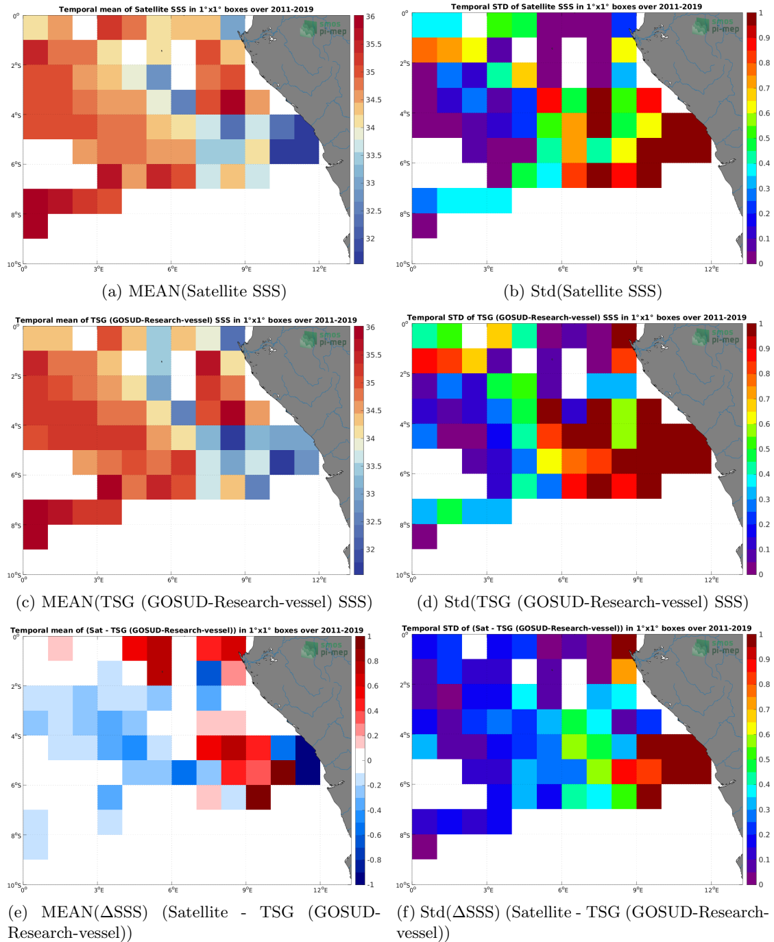
Figure 6: Temporal mean (left) and Std (right) of SSS from SMAP SSS L4 OI v2 - 7 Days (ESR) (top), TSG (GOSUD-Research-vessel) (middle), and of \Delta SSS (Satellite - TSG (GOSUD-Research-vessel)). Only match-up pairs are used to generate these maps.
