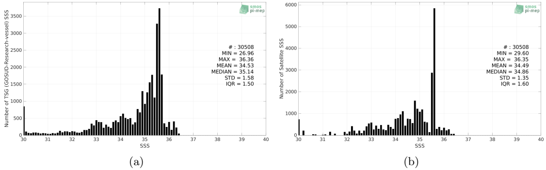
Figure 2: Histograms of SSS from TSG (GOSUD-Research-vessel) (a) and SMAP SSS L4 OI v2 - 7 Days (ESR) (b) considering all match-up pairs per bins of 0.1 over the Congo river plume Pi-MEP region and for the full satellite product period.
