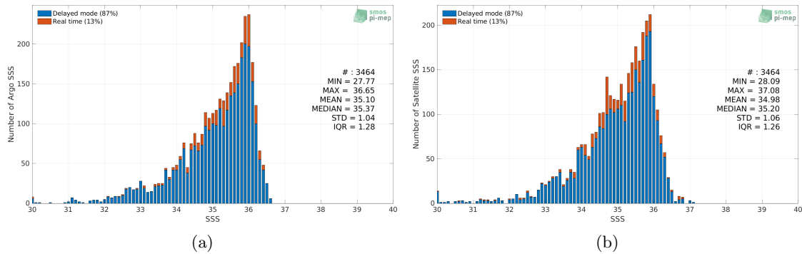
Figure 2: Histograms of SSS from Argo (a) and SMAP SSS L4 OI v2 - 7 Days (ESR) (b) considering all match-up pairs per bins of 0.1 over the Congo river plume Pi-MEP region and for the full satellite product period.
