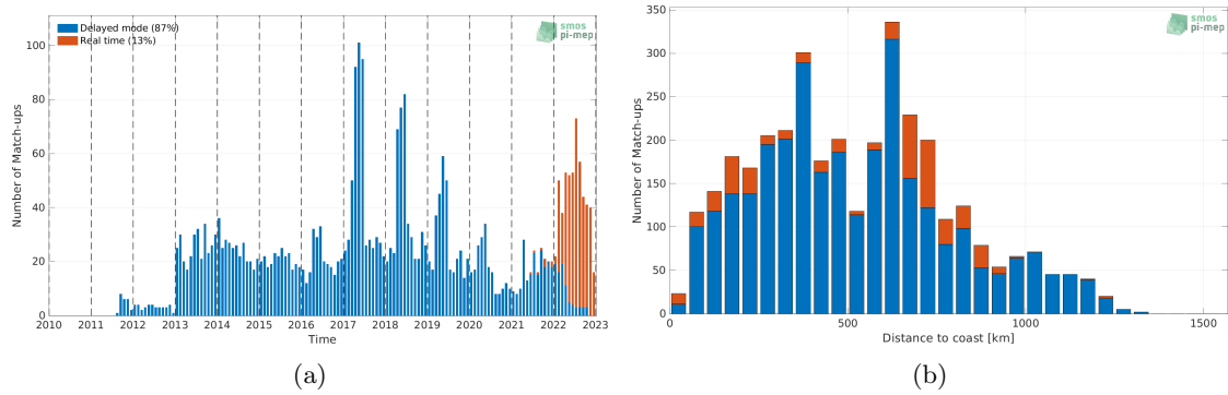
Figure 1: Number of match-ups between Argo and SMAP SSS L4 OI v2 - 7 Days (ESR) SSS as a function of time (a) and as function of the distance to coast (b) over the Congo river plume Pi-MEP region and for the full satellite product period.
