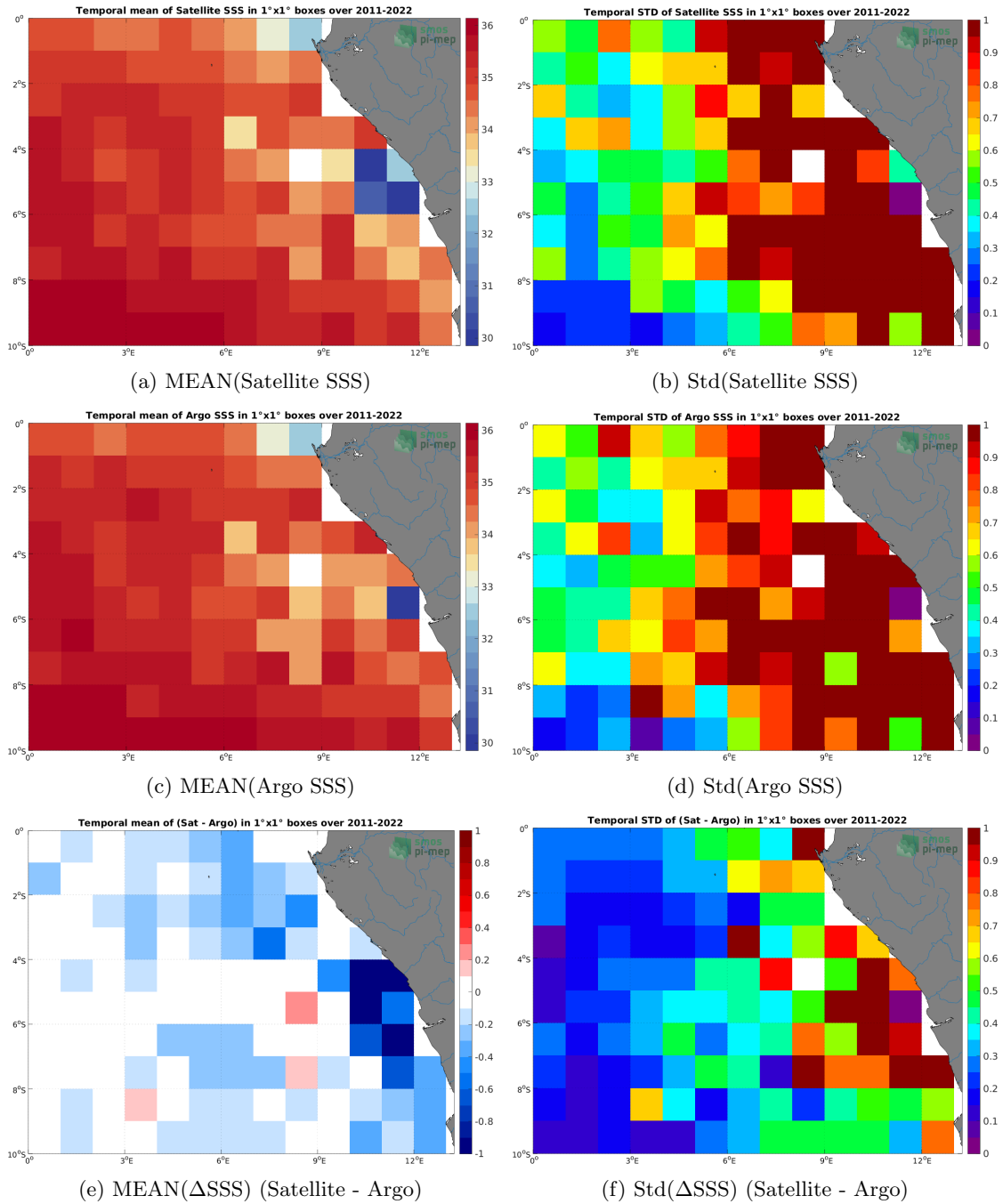
Figure 6: Temporal mean (left) and Std (right) of SSS from SMAP SSS L4 OI v2 - 7 Days (ESR) (top), Argo (middle), and of \Delta SSS (Satellite - Argo). Only match-up pairs are used to generate these maps.
