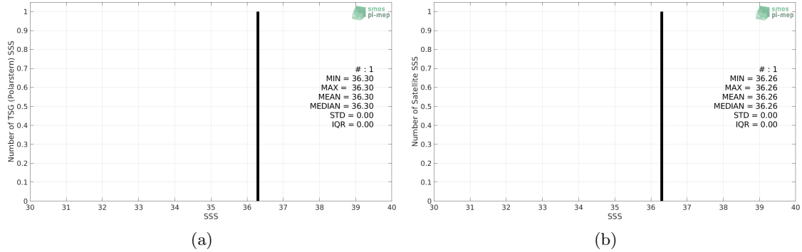
Figure 2: Histograms of SSS from TSG (Polarstern) (a) and SMAP SSS L3 v4 - 8-Day running (RSS) (b) considering all match-up pairs per bins of 0.1 over the Congo river plume Pi-MEP region and for the full satellite product period.
