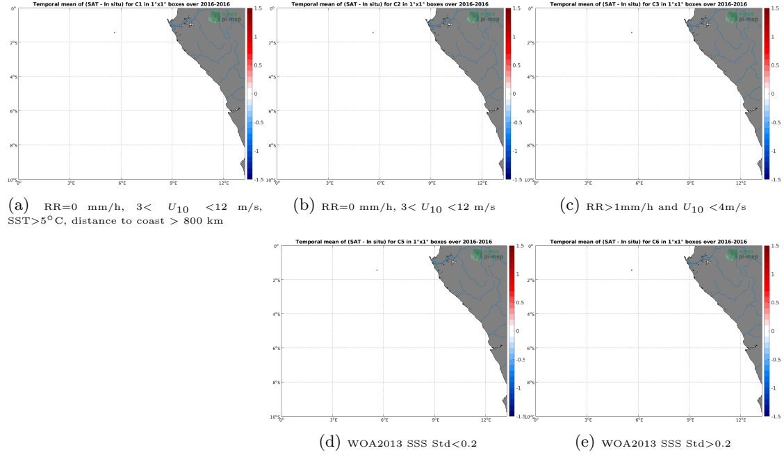
Figure 12: Temporal mean gridded over spatial boxes of size 1^{\circ}\times 1^{\circ} of \Delta\text{SSS} (SMAP SSS L3 v4 - 8-Day running (RSS) - TSG (Polarstern)) for 5 different subdatasets corresponding to:RR=0 mm/h, 3 < U_{10} < 12 m/s, SST >5^{\circ}\text{C} , distance to coast > 800 km (a), RR=0 mm/h, 3 < U_{10} < 12 m/s (b), RR >1 mm/h and U_{10} < 4 m/s (c), WOA2013 SSS Std <0.2 (d), WOA2013 SSS Std >0.2 (e).
