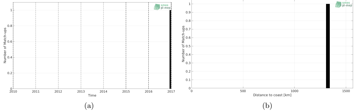
Figure 1: Number of match-ups between TSG (Polarstern) and SMAP SSS L3 v4 - 8-Day running (RSS) SSS as a function of time (a) and as function of the distance to coast (b) over the Congo river plume Pi-MEP region and for the full satellite product period.
