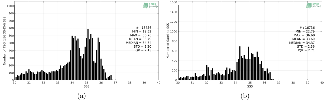
Figure 2: Histograms of SSS from TSG (LEGOS-DM) (a) and SMAP SSS L3 v4 - 8-Day running (RSS) (b) considering all match-up pairs per bins of 0.1 over the Congo river plume Pi-MEP region and for the full satellite product period.
