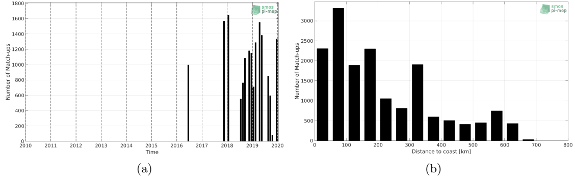
Figure 1: Number of match-ups between TSG (LEGOS-DM) and SMAP SSS L3 v4 - 8-Day running (RSS) SSS as a function of time (a) and as function of the distance to coast (b) over the Congo river plume Pi-MEP region and for the full satellite product period.
