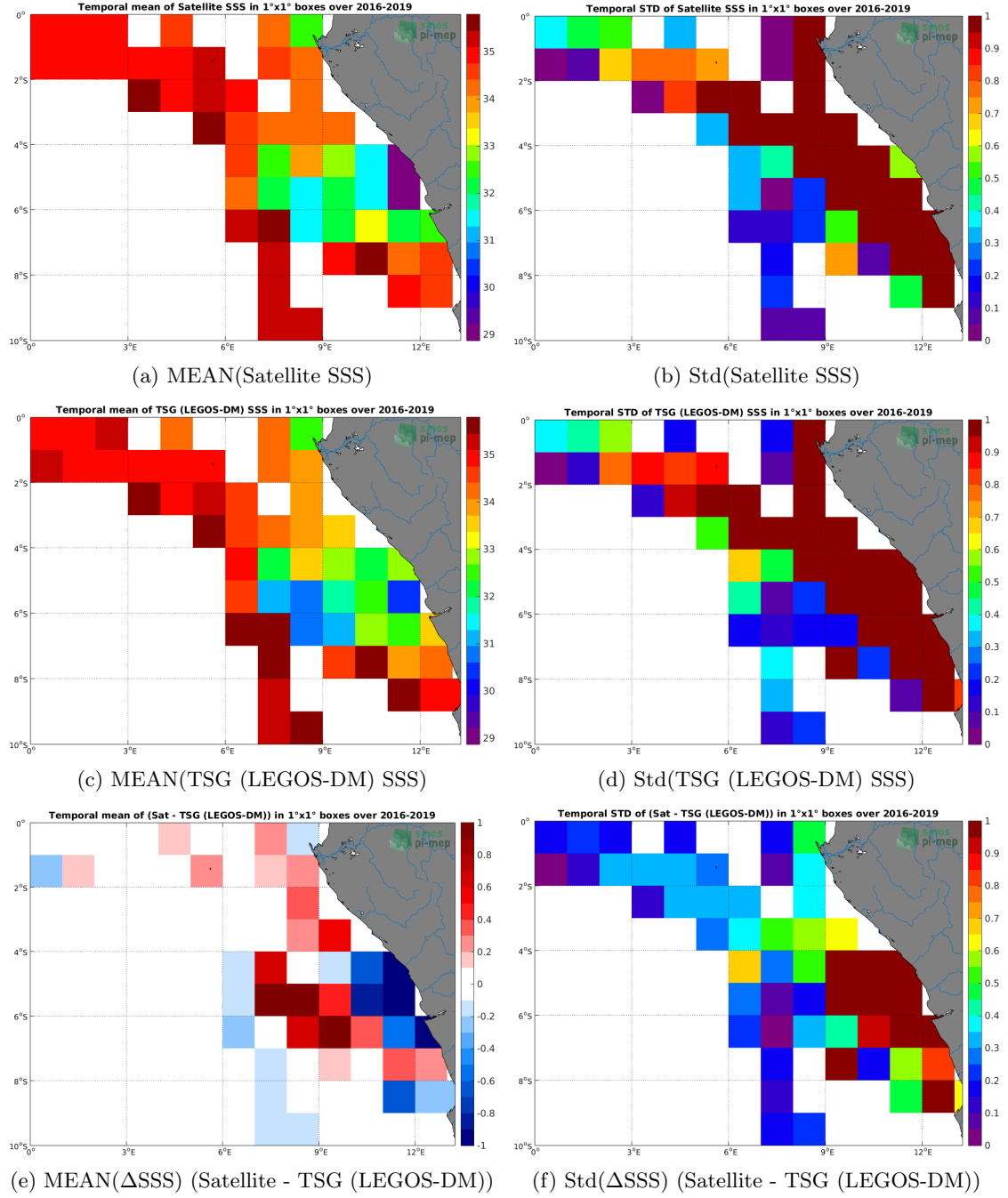
Figure 6: Temporal mean (left) and Std (right) of SSS from SMAP SSS L3 v4 - 8-Day running (RSS) (top), TSG (LEGOS-DM) (middle), and of \Delta SSS (Satellite - TSG (LEGOS-DM)). Only match-up pairs are used to generate these maps.
