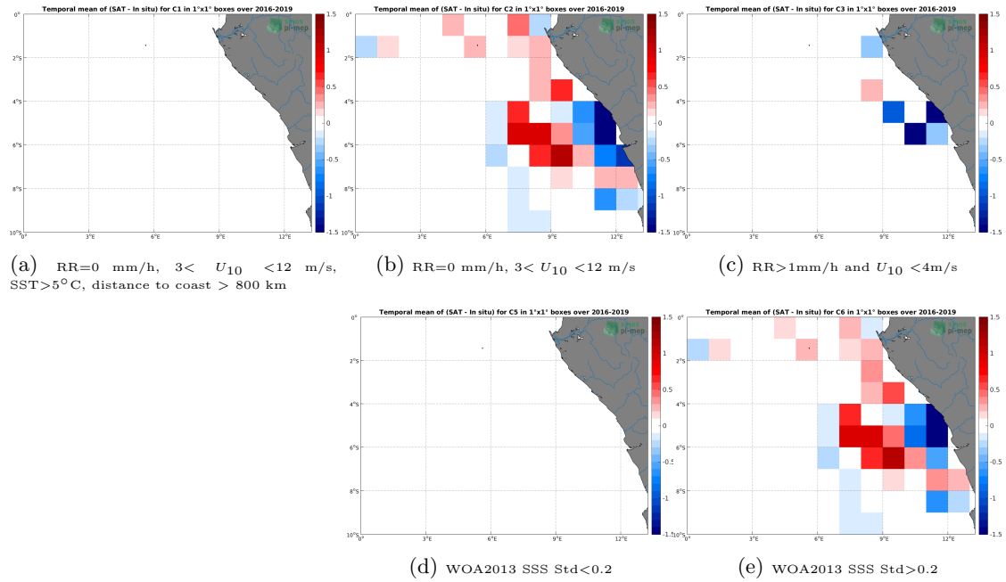
Figure 12: Temporal mean gridded over spatial boxes of size 1^\circ \times 1^\circ of \Delta SSS (SMAP SSS L3 v4 - 8-Day running (RSS) - TSG (LEGOS-DM)) for 5 different subdatasets corresponding to: RR=0 mm/h, 3 < U_{10} < 12 m/s, SST > 5^\circ C , distance to coast > 800 km (a), RR=0 mm/h, 3 < U_{10} < 12 m/s (b), RR > 1 mm/h and U_{10} < 4 m/s (c), WOA2013 SSS Std < 0.2 (d), WOA2013 SSS Std > 0.2 (e).
