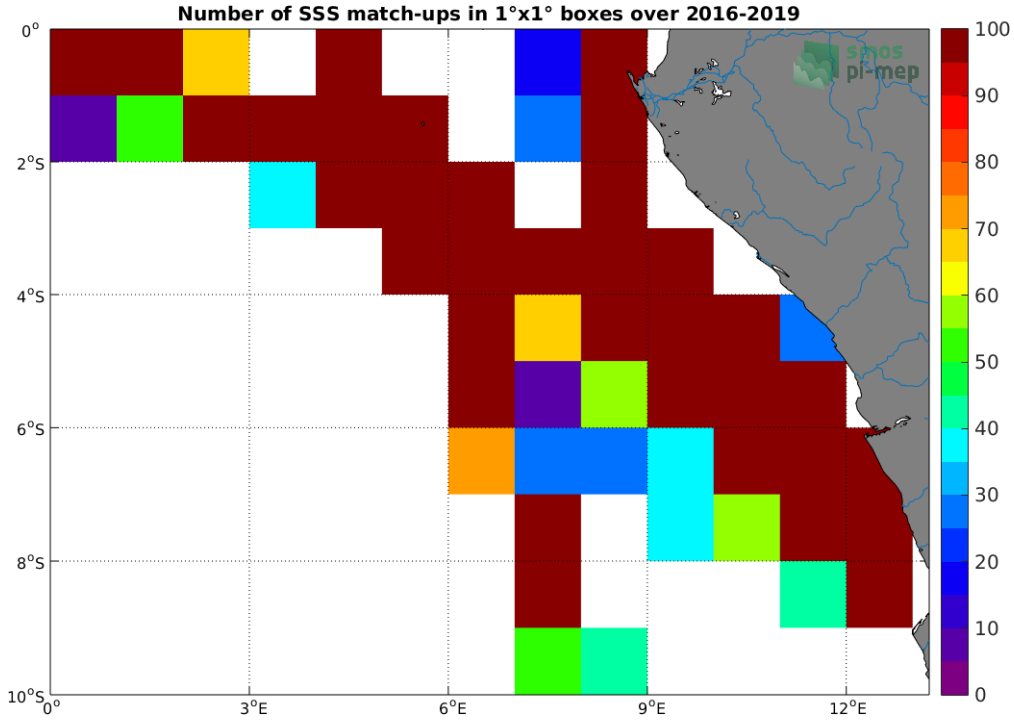
Figure 4: Number of SSS match-ups between TSG (LEGOS-DM) SSS and the SMAP SSS L3 v4 - 8-Day running (RSS) SSS product for the Congo river plume Pi-MEP region over 1^\circ \times 1^\circ boxes and for the full satellite product period.
