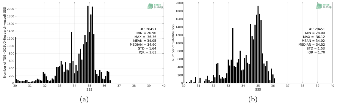
Figure 2: Histograms of SSS from TSG (GOSUD-Research-vessel) (a) and SMAP SSS L3 v4 - 8-Day running (RSS) (b) considering all match-up pairs per bins of 0.1 over the Congo river plume Pi-MEP region and for the full satellite product period.
