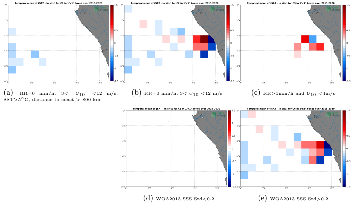
Figure 12: Temporal mean gridded over spatial boxes of size 1^\circ \times 1^\circ of \Delta SSS (SMAP SSS L3 v4 - 8-Day running (RSS) - TSG (GOSUD-Research-vessel)) for 5 different subdatasets corresponding to: RR=0 mm/h, 3 < U_{10} < 12 m/s, SST > 5^\circ C , distance to coast > 800 km (a), RR=0 mm/h, 3 < U_{10} < 12 m/s (b), RR > 1 mm/h and U_{10} < 4 m/s (c), WOA2013 SSS Std < 0.2 (d), WOA2013 SSS Std > 0.2 (e).
