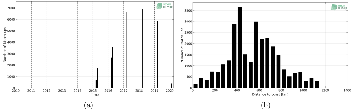
Figure 1: Number of match-ups between TSG (GOSUD-Research-vessel) and SMAP SSS L3 v4 - 8-Day running (RSS) SSS as a function of time (a) and as function of the distance to coast (b) over the Congo river plume Pi-MEP region and for the full satellite product period.
