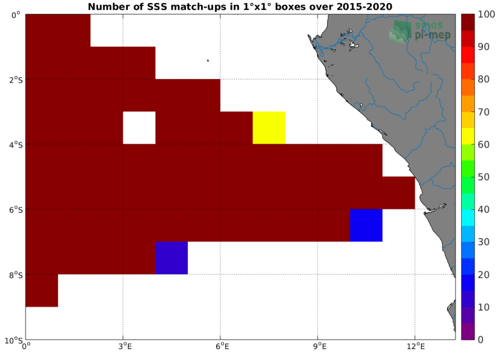
Figure 4: Number of SSS match-ups between TSG (GOSUD-Research-vessel) SSS and the SMAP SSS L3 v4 - 8-Day running (RSS) SSS product for the Congo river plume Pi-MEP region over 1^\circ \times 1^\circ boxes and for the full satellite product period.
