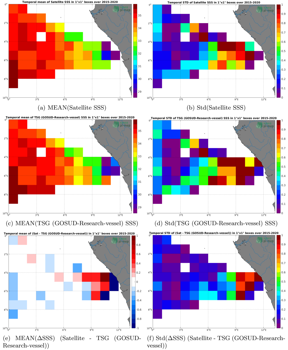
Figure 6: Temporal mean (left) and Std (right) of SSS from SMAP SSS L3 v4 - 8-Day running (RSS) (top), TSG (GOSUD-Research-vessel) (middle), and of \Delta SSS (Satellite - TSG (GOSUD-Research-vessel)). Only match-up pairs are used to generate these maps.
