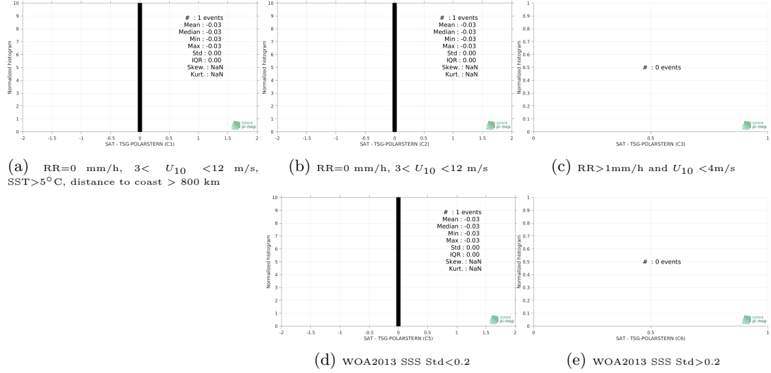
Figure 13: Normalized histogram of \Delta\text{SSS} (SMAP-L3-RSS-V4-MONTHLY - TSG-POLARSTERN) for 5 different subdatasets corresponding to: RR=0 mm/h, 3 < U_{10} < 12 m/s, SST > 5^\circ\text{C} , distance to coast > 800 km (a), RR=0 mm/h, 3 < U_{10} < 12 m/s (b), RR > 1\text{mm/h} and U_{10} < 4\text{m/s} (c), WOA2013 SSS Std <0.2 (d), WOA2013 SSS Std >0.2 (e).
