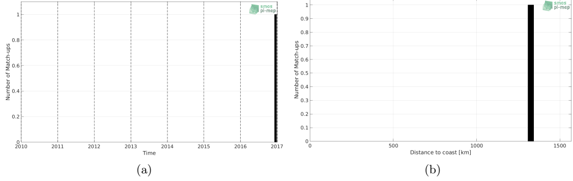
Figure 1: Number of match-ups between TSG-POLARSTERN and SMAP-L3-RSS-V4-MONTHLY SSS as a function of time (a) and as function of the distance to coast (b) over the Congo river plume Pi-MEP region and for the full satellite product period.
