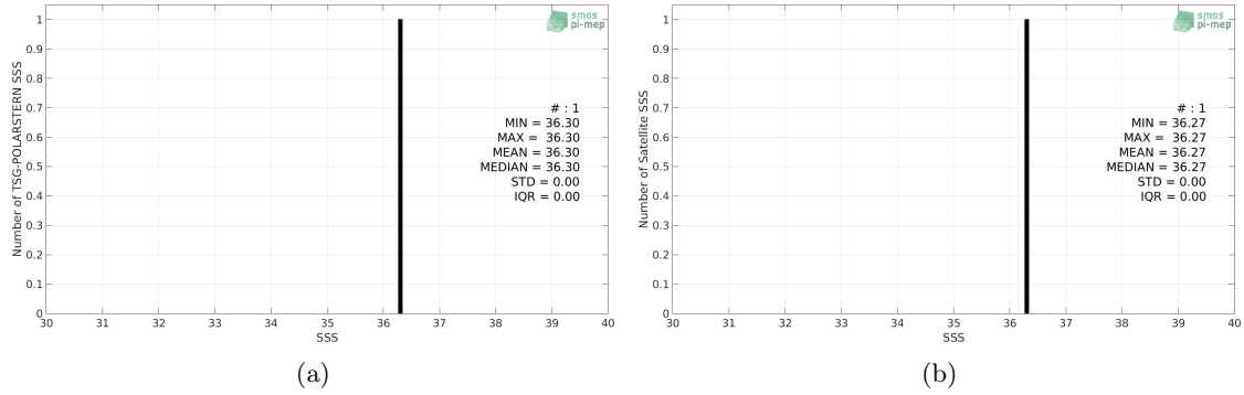
Figure 2: Histograms of SSS from TSG-POLARSTERN (a) and SMAP-L3-RSS-V4-MONTHLY (b) considering all match-up pairs per bins of 0.1 over the Congo river plume Pi-MEP region and for the full satellite product period.
