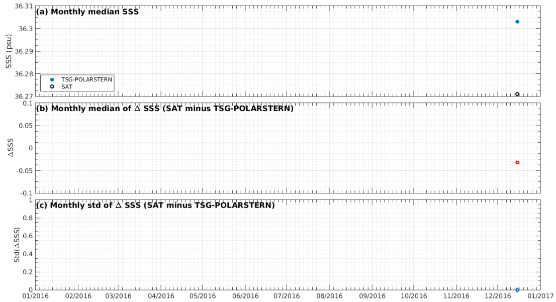
Figure 7: Time series of the monthly median SSS (top), median of \Delta SSS (Satellite - TSG-POLARSTERN) and Std of \Delta SSS (Satellite - TSG-POLARSTERN) over the Congo river plume Pi-MEP region considering all match-ups collected by the Pi-MEP.
