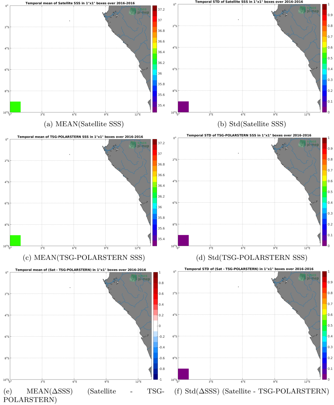
Figure 6: Temporal mean (left) and Std (right) of SSS from SMAP-L3-RSS-V4-MONTHLY (top), TSG-POLARSTERN (middle), and of \Delta SSS (Satellite - TSG-POLARSTERN). Only match-up pairs are used to generate these maps.
