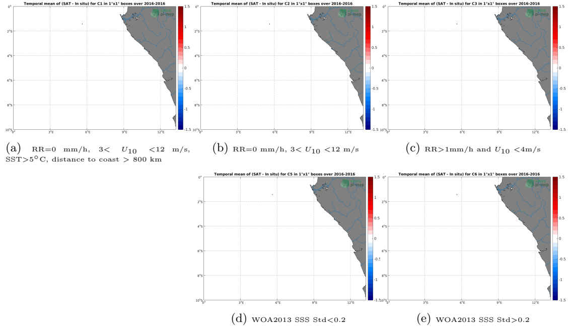
Figure 12: Temporal mean gridded over spatial boxes of size 1^\circ \times 1^\circ of \Delta SSS (SMAP-L3-RSS-V4-MONTHLY - TSG-POLARSTERN) for 5 different subdatasets corresponding to: RR=0 mm/h, 3 < U_{10} < 12 m/s, SST > 5^\circ C , distance to coast > 800 km (a), RR=0 mm/h, 3 < U_{10} < 12 m/s (b), RR > 1 mm/h and U_{10} < 4 m/s (c), WOA2013 SSS Std < 0.2 (d), WOA2013 SSS Std > 0.2 (e).
