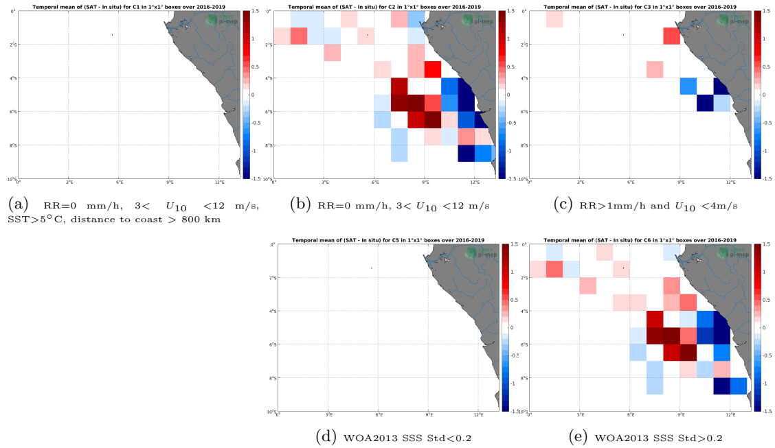
Figure 12: Temporal mean gridded over spatial boxes of size 1^\circ \times 1^\circ of \Delta\text{SSS} (SMAP SSS L3 v4 - Monthly (RSS) - TSG (LEGOS-DM)) for 5 different subdatasets corresponding to: \text{RR}=0 mm/h, 3 < U_{10} < 12 m/s, \text{SST} > 5^\circ\text{C} , distance to coast > 800 km (a), \text{RR}=0 mm/h, 3 < U_{10} < 12 m/s (b), \text{RR} > 1 mm/h and U_{10} < 4 m/s (c), WOA2013 SSS Std < 0.2 (d), WOA2013 SSS Std > 0.2 (e).
