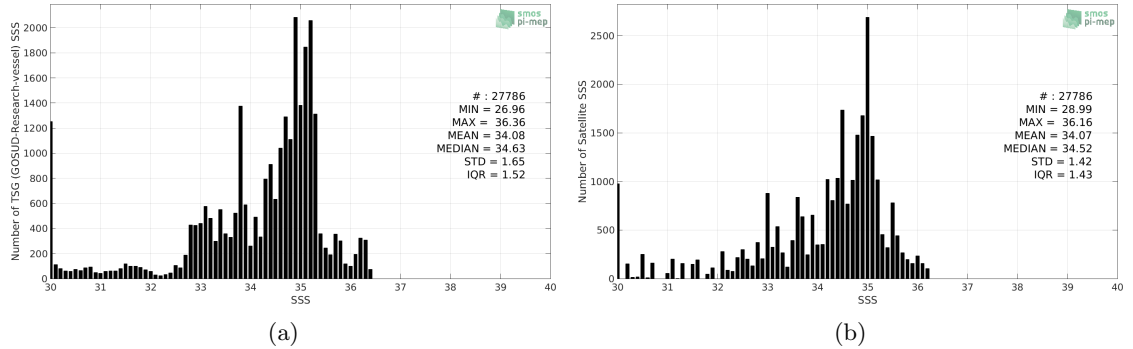
Figure 2: Histograms of SSS from TSG (GOSUD-Research-vessel) (a) and SMAP SSS L3 v4 - Monthly (RSS) (b) considering all match-up pairs per bins of 0.1 over the Congo river plume Pi-MEP region and for the full satellite product period.
