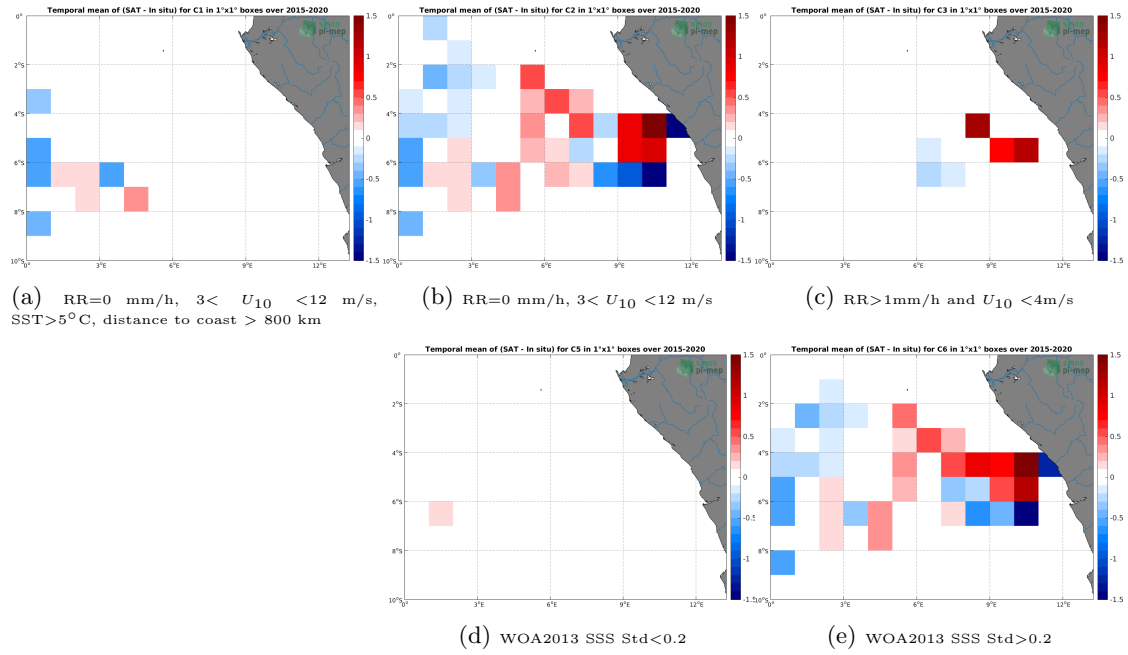
Figure 12: Temporal mean gridded over spatial boxes of size 1^\circ \times 1^\circ of \Delta SSS (SMAP SSS L3 v4 - Monthly (RSS) - TSG (GOSUD-Research-vessel)) for 5 different subdatasets corresponding to: RR=0 mm/h, 3 < U_{10} < 12 m/s, SST >5^\circ\text{C} , distance to coast > 800 km (a), RR=0 mm/h, 3 < U_{10} < 12 m/s (b), RR >1 mm/h and U_{10} < 4 m/s (c), WOA2013 SSS Std <0.2 (d), WOA2013 SSS Std >0.2 (e).
