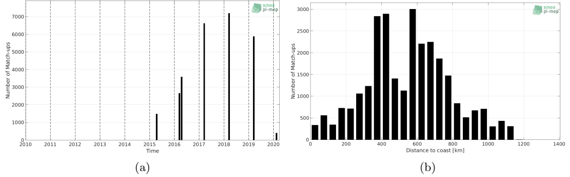
Figure 1: Number of match-ups between TSG (GOSUD-Research-vessel) and SMAP SSS L3 v4 - Monthly (RSS) SSS as a function of time (a) and as function of the distance to coast (b) over the Congo river plume Pi-MEP region and for the full satellite product period.
