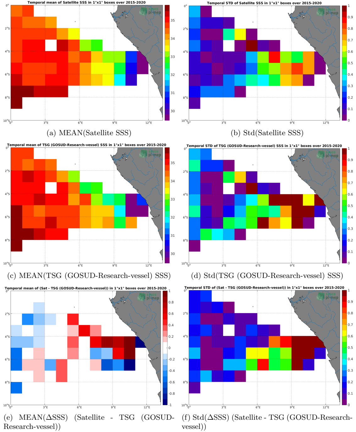
Figure 6: Temporal mean (left) and Std (right) of SSS from SMAP SSS L3 v4 - Monthly (RSS) (top), TSG (GOSUD-Research-vessel) (middle), and of \Delta SSS (Satellite - TSG (GOSUD-Research-vessel)). Only match-up pairs are used to generate these maps.
