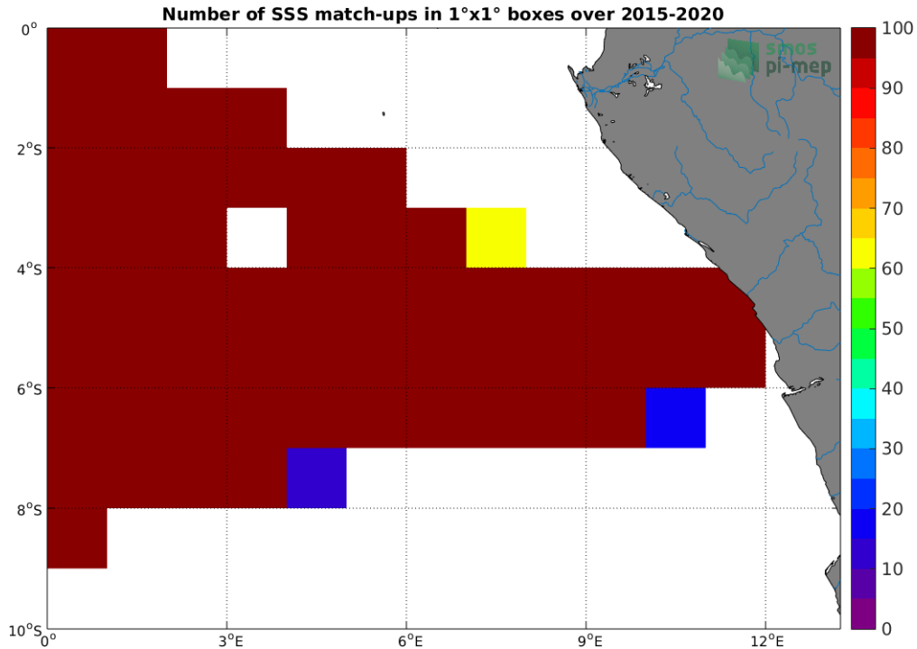
Figure 4: Number of SSS match-ups between TSG (GOSUD-Research-vessel) SSS and the SMAP SSS L3 v4 - Monthly (RSS) SSS product for the Congo river plume Pi-MEP region over 1^\circ \times 1^\circ boxes and for the full satellite product period.
