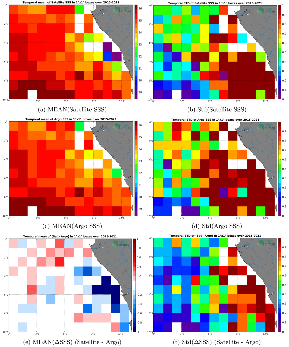
Figure 6: Temporal mean (left) and Std (right) of SSS from SMAP SSS L3 v4 - Monthly (RSS) (top), Argo (middle), and of \Delta SSS (Satellite - Argo). Only match-up pairs are used to generate these maps.
