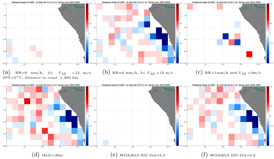
Figure 12: Temporal mean gridded over spatial boxes of size 1^\circ \times 1^\circ of \Delta SSS (SMAP-L3-RSS-V4-MONTHLY - Argo) for 6 different subdatasets corresponding to: RR=0 mm/h, 3 < U_{10} < 12 m/s, SST > 5^\circ\text{C} , distance to coast > 800 km (a), RR=0 mm/h, 3 < U_{10} < 12 m/s (b), RR > 1 mm/h and U_{10} < 4 m/s (c), MLD < 20 m (d), WOA2013 SSS Std < 0.2 (e), WOA2013 SSS Std > 0.2 (f).
