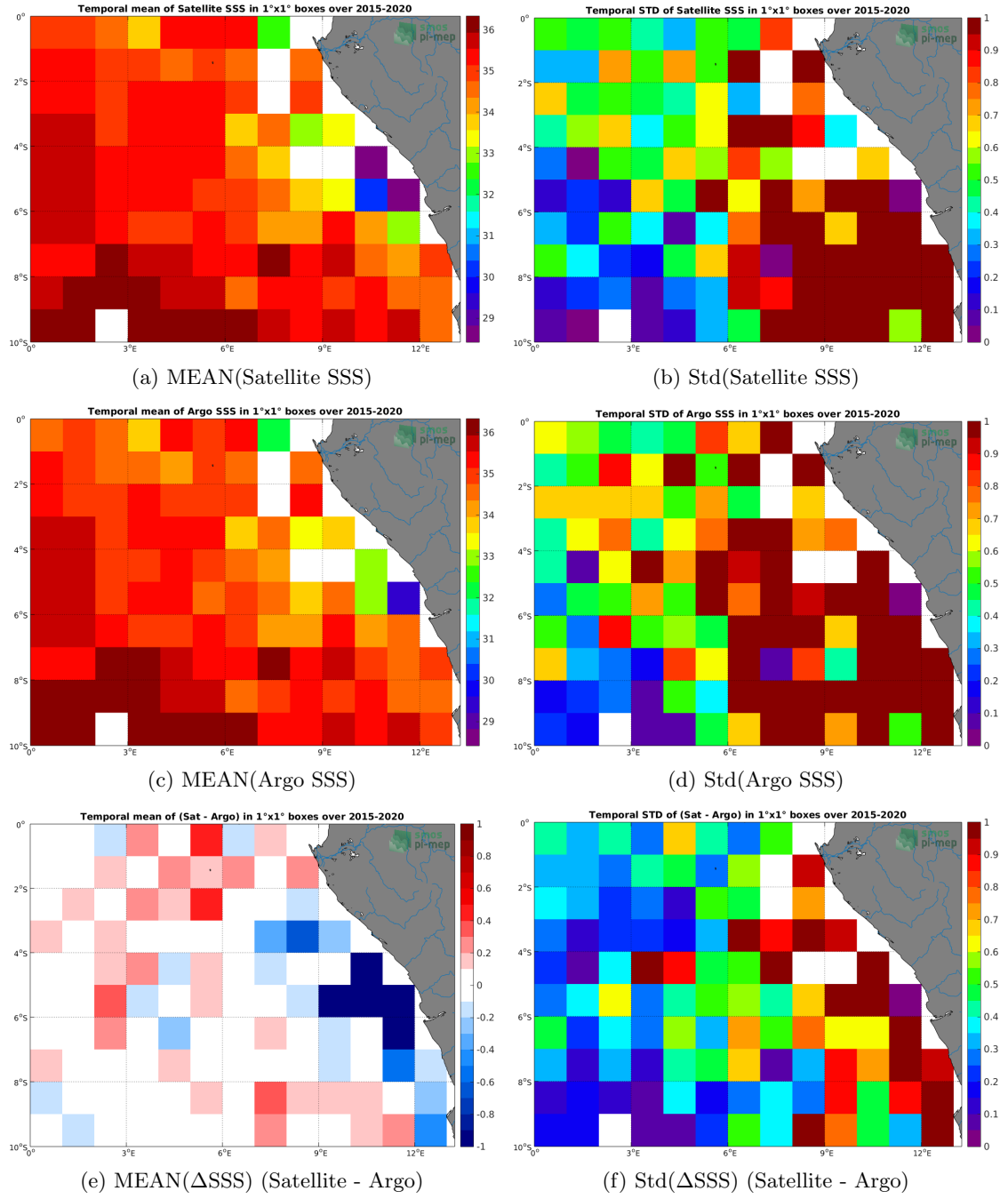
Figure 6: Temporal mean (left) and Std (right) of SSS from SMAP-L3-RSS-V4-MONTHLY (top), Argo (middle), and of \Delta SSS (Satellite - Argo). Only match-up pairs are used to generate these maps.
