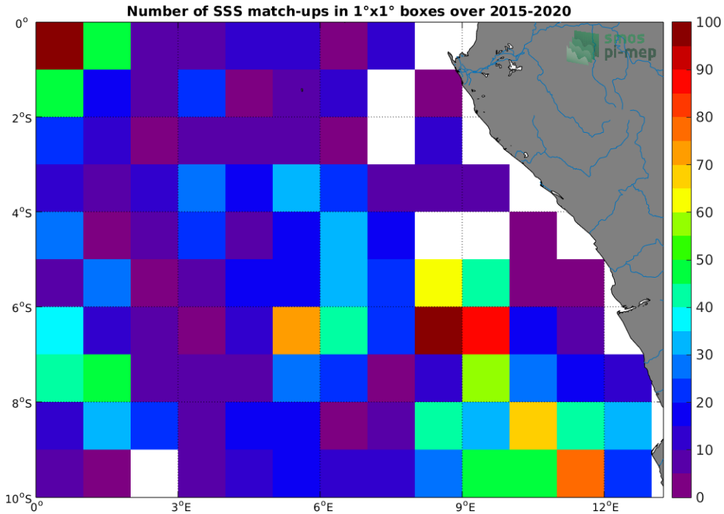
Figure 4: Number of SSS match-ups between Argo SSS and the SMAP-L3-RSS-V4-MONTHLY SSS product for the Congo river plume Pi-MEP region over 1°x1° boxes and for the full satellite product period.
