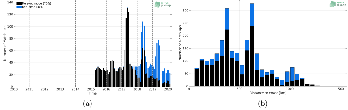
Figure 1: Number of match-ups between Argo and SMAP-L3-RSS-V4-MONTHLY SSS as a function of time (a) and as function of the distance to coast (b) over the Congo river plume Pi-MEP region and for the full satellite product period.
