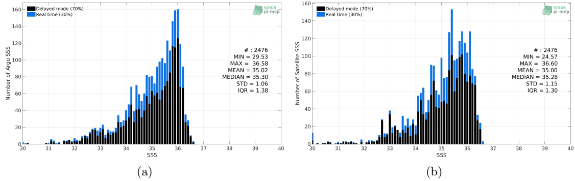
Figure 2: Histograms of SSS from Argo (a) and SMAP-L3-RSS-V4-MONTHLY (b) considering all match-up pairs per bins of 0.1 over the Congo river plume Pi-MEP region and for the full satellite product period.
