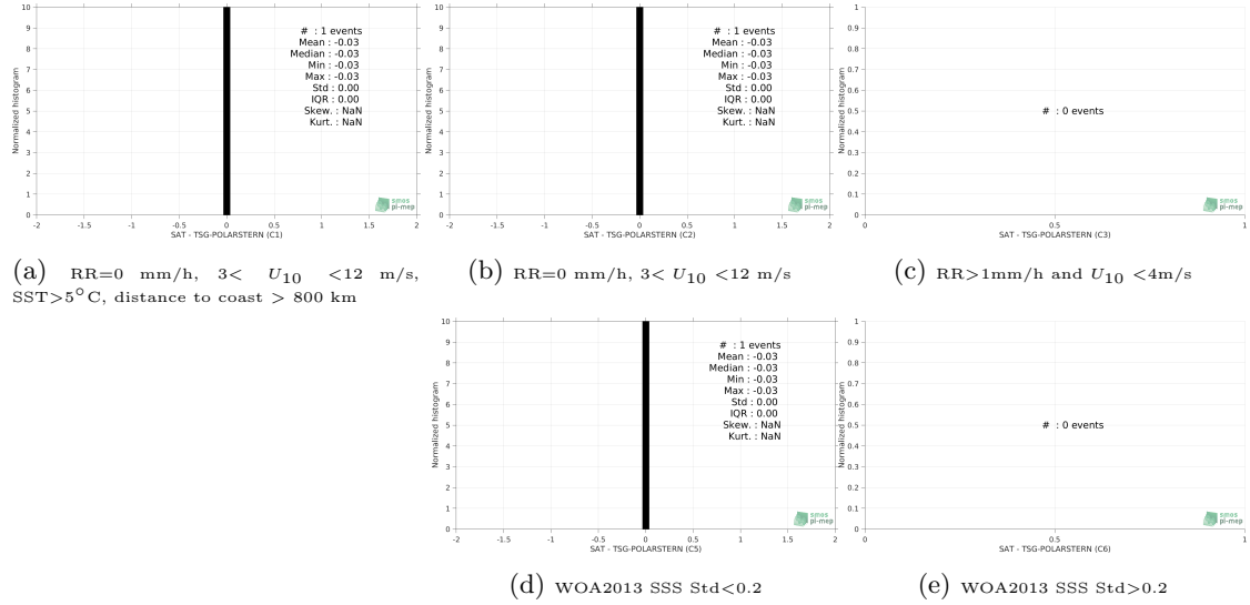
Figure 13: Normalized histogram of \Delta SSS (SMAP-L3-RSS-V3-8DAY-RUNNING-40KM - TSG-POLARSTERN) for 5 different subdatasets corresponding to: RR=0 mm/h, 3 < U_{10} < 12 m/s, SST >5^{\circ} C, distance to coast > 800 km (a), RR=0 mm/h, 3 < U_{10} < 12 m/s (b), RR >1 mm/h and U_{10} < 4 m/s (c), WOA2013 SSS Std <0.2 (d), WOA2013 SSS Std >0.2 (e).
