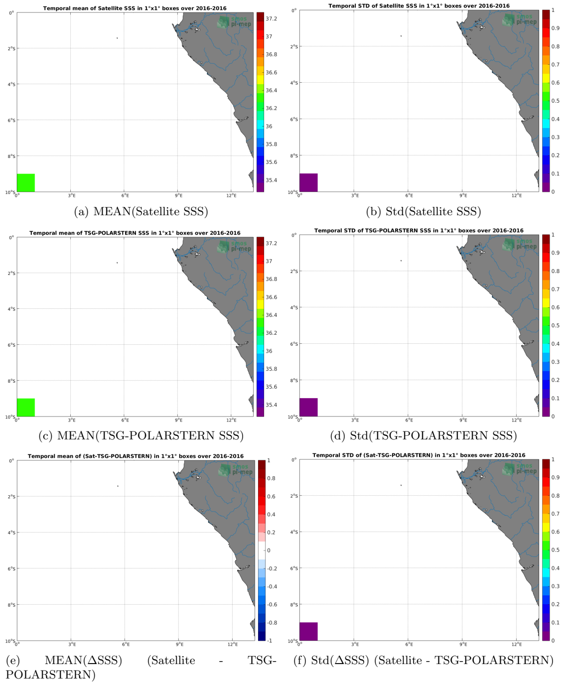
Figure 6: Temporal mean (left) and Std (right) of SSS from SMAP-L3-RSS-V3-8DAY-RUNNING-40KM (top), TSG-POLARSTERN (middle), and of \Delta SSS (Satellite - TSG-POLARSTERN). Only match-up pairs are used to generate these maps.
