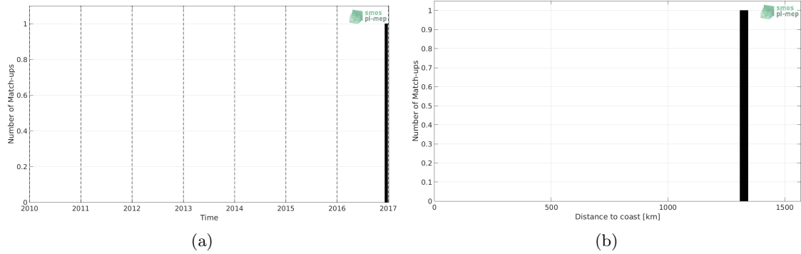
Figure 1: Number of match-ups between TSG-POLARSTERN and SMAP-L3-RSS-V3-8DAY-RUNNING-40KM SSS as a function of time (a) and as function of the distance to coast (b) over the Congo river plume Pi-MEP region and for the full satellite product period.
