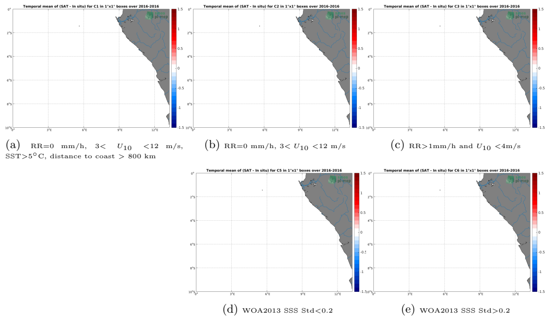
Figure 12: Temporal mean gridded over spatial boxes of size 1^\circ \times 1^\circ of \Delta SSS (SMAP-L3-RSS-V3-8DAY-RUNNING-40KM - TSG-POLARSTERN) for 5 different subdatasets corresponding to:RR=0 mm/h, 3 < U_{10} < 12 m/s, SST >5^\circ C, distance to coast > 800 km (a), RR=0 mm/h, 3 < U_{10} < 12 m/s (b), RR >1 mm/h and U_{10} < 4 m/s (c), WOA2013 SSS Std <0.2 (d), WOA2013 SSS Std >0.2 (e).
