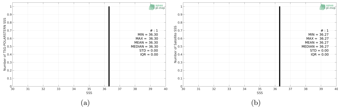
Figure 2: Histograms of SSS from TSG-POLARSTERN (a) and SMAP-L3-RSS-V3-8DAY-RUNNING-40KM (b) considering all match-up pairs per bins of 0.1 over the Congo river plume Pi-MEP region and for the full satellite product period.
