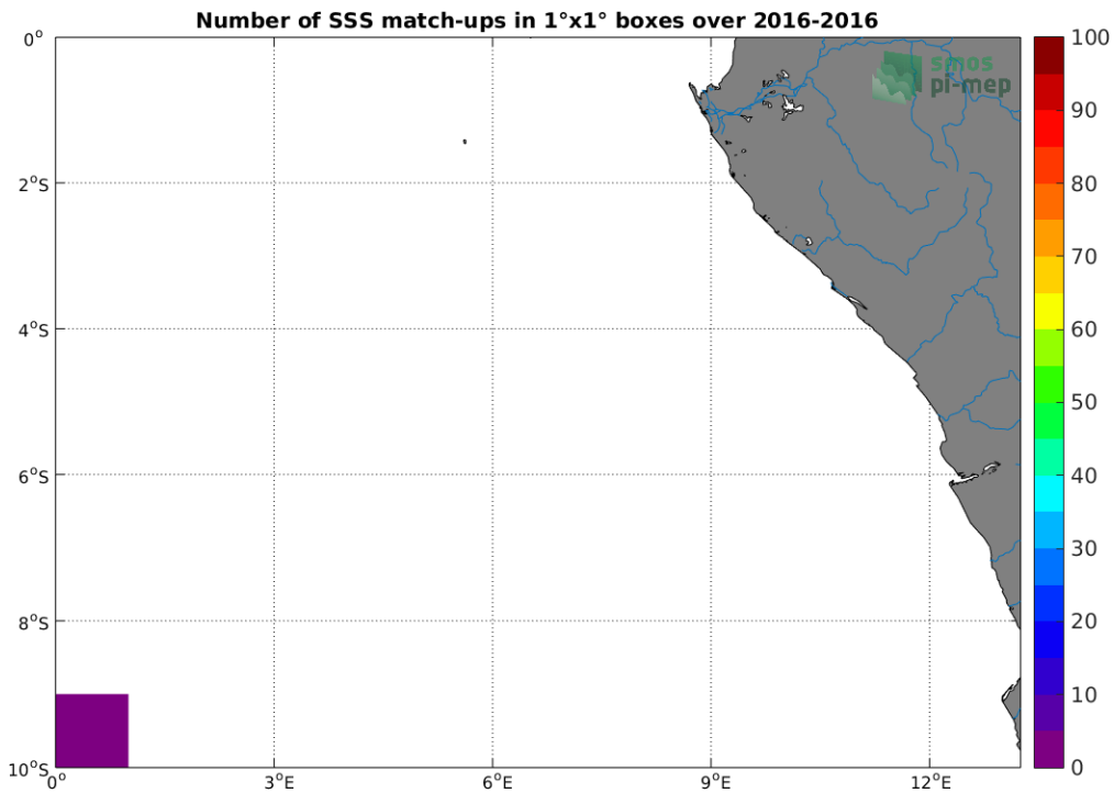
Figure 4: Number of SSS match-ups between TSG-POLARSTERN SSS and the SMAP-L3-RSS-V3-8DAY-RUNNING-40KM SSS product for the Congo river plume Pi-MEP region over 1^\circ \times 1^\circ boxes and for the full satellite product period.
