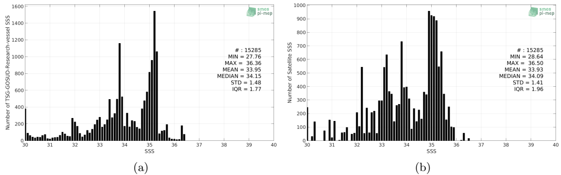
Figure 2: Histograms of SSS from TSG-GOSUD-Research-vessel (a) and SMAP-L3-RSS-V3-8DAY-RUNNING-40KM (b) considering all match-up pairs per bins of 0.1 over the Congo river plume Pi-MEP region and for the full satellite product period.
