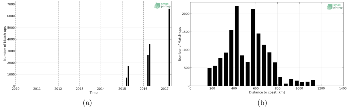
Figure 1: Number of match-ups between TSG-GOSUD-Research-vessel and SMAP-L3-RSS-V3-8DAY-RUNNING-40KM SSS as a function of time (a) and as function of the distance to coast (b) over the Congo river plume Pi-MEP region and for the full satellite product period.
