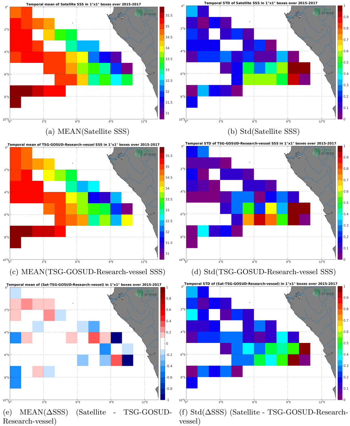
Figure 6: Temporal mean (left) and Std (right) of SSS from SMAP-L3-RSS-V3-8DAY-RUNNING-40KM (top), TSG-GOSUD-Research-vessel (middle), and of \Delta SSS (Satellite - TSG-GOSUD-Research-vessel). Only match-up pairs are used to generate these maps.
