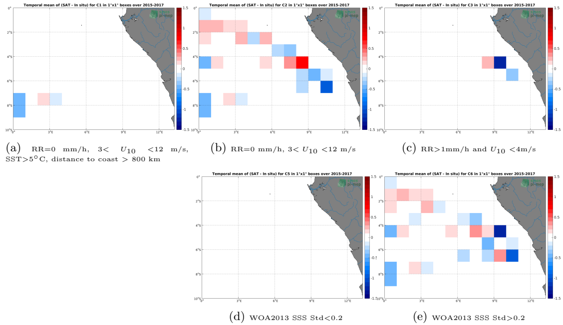
Figure 12: Temporal mean gridded over spatial boxes of size 1^\circ \times 1^\circ of \Delta SSS (SMAP-L3-RSS-V3-8DAY-RUNNING-40KM - TSG-GOSUD-Research-vessel) for 5 different subdatasets corresponding to:RR=0 mm/h, 3 < U_{10} < 12 m/s, SST >5^\circ\text{C} , distance to coast > 800 km (a), RR=0 mm/h, 3 < U_{10} < 12 m/s (b), RR >1 mm/h and U_{10} < 4 m/s (c), WOA2013 SSS Std <0.2 (d), WOA2013 SSS Std >0.2 (e).
