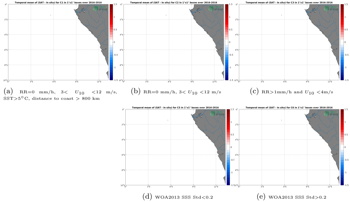
Figure 12: Temporal mean gridded over spatial boxes of size 1^\circ \times 1^\circ of \Delta SSS (SMAP-L3-RSS-V3-MONTHLY-70KM - TSG-POLARSTERN) for 5 different subdatasets corresponding to:RR=0 mm/h, 3 < U_{10} < 12 m/s, SST >5^\circ C, distance to coast > 800 km (a), RR=0 mm/h, 3 < U_{10} < 12 m/s (b), RR >1 mm/h and U_{10} < 4 m/s (c), WOA2013 SSS Std <0.2 (d), WOA2013 SSS Std >0.2 (e).
