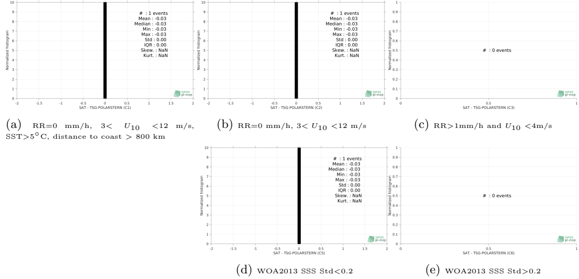
Figure 13: Normalized histogram of \Delta SSS (SMAP-L3-RSS-V3-MONTHLY-70KM - TSG-POLARSTERN) for 5 different subdatasets corresponding to: RR=0 mm/h, 3 < U_{10} < 12 m/s, SST > 5^\circ C , distance to coast > 800 km (a), RR=0 mm/h, 3 < U_{10} < 12 m/s (b), RR > 1 mm/h and U_{10} < 4 m/s (c), WOA2013 SSS Std < 0.2 (d), WOA2013 SSS Std > 0.2 (e).
