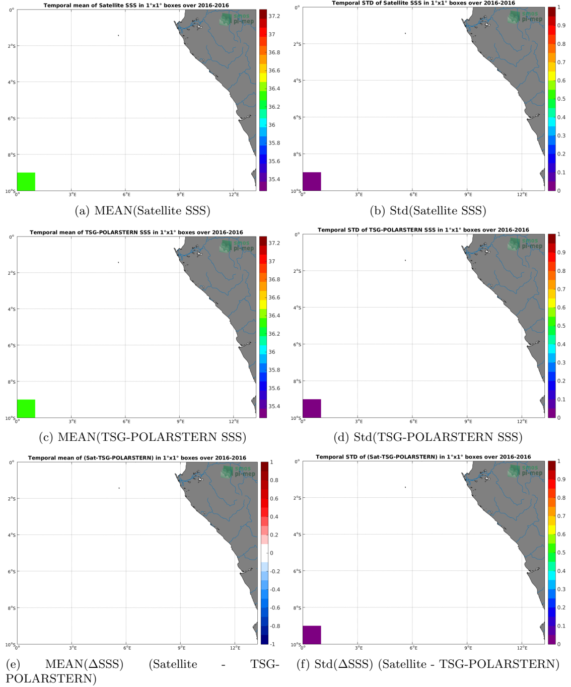
Figure 6: Temporal mean (left) and Std (right) of SSS from SMAP-L3-RSS-V3-MONTHLY-70KM (top), TSG-POLARSTERN (middle), and of \Delta SSS (Satellite - TSG-POLARSTERN). Only match-up pairs are used to generate these maps.
