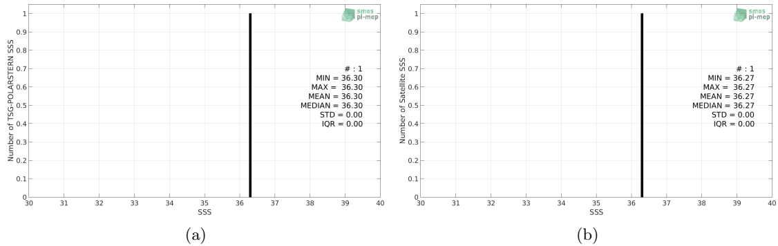
Figure 2: Histograms of SSS from TSG-POLARSTERN (a) and SMAP-L3-RSS-V3-MONTHLY-70KM (b) considering all match-up pairs per bins of 0.1 over the Congo river plume Pi-MEP region and for the full satellite product period.
