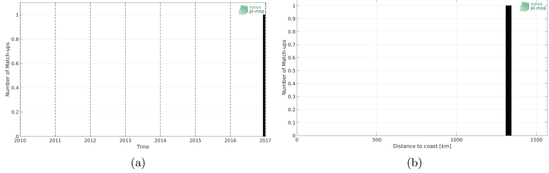
Figure 1: Number of match-ups between TSG-POLARSTERN and SMAP-L3-RSS-V3-MONTHLY-70KM SSS as a function of time (a) and as function of the distance to coast (b) over the Congo river plume Pi-MEP region and for the full satellite product period.
