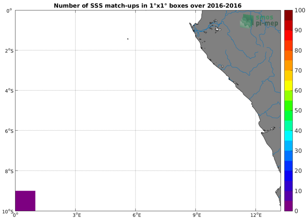
Figure 4: Number of SSS match-ups between TSG-POLARSTERN SSS and the SMAP-L3-RSS-V3-MONTHLY-70KM SSS product for the Congo river plume Pi-MEP region over 1^\circ \times 1^\circ boxes and for the full satellite product period.
