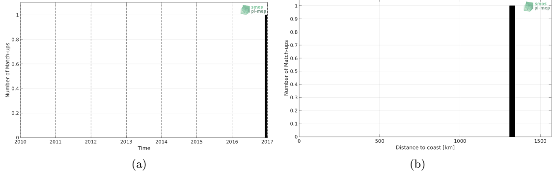
Figure 1: Number of match-ups between TSG-POLARSTERN and SMAP-L3-RSS-V3-MONTHLY-0.25DEG-40KM SSS as a function of time (a) and as function of the distance to coast (b) over the Congo river plume Pi-MEP region and for the full satellite product period.
