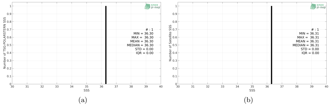
Figure 2: Histograms of SSS from TSG-POLARSTERN (a) and SMAP-L3-RSS-V3-MONTHLY-0.25DEG-40KM (b) considering all match-up pairs per bins of 0.1 over the Congo river plume Pi-MEP region and for the full satellite product period.
