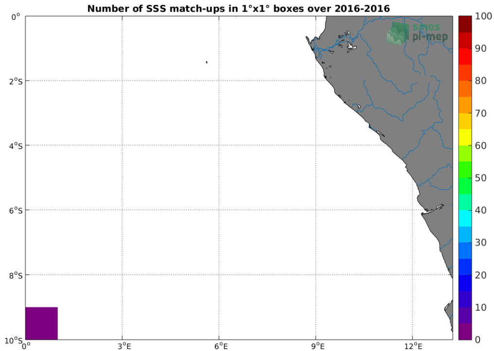
Figure 4: Number of SSS match-ups between TSG-POLARSTERN SSS and the SMAP-L3-RSS-V3-MONTHLY-0.25DEG-40KM SSS product for the Congo river plume Pi-MEP region over 1^\circ \times 1^\circ boxes and for the full satellite product period.
