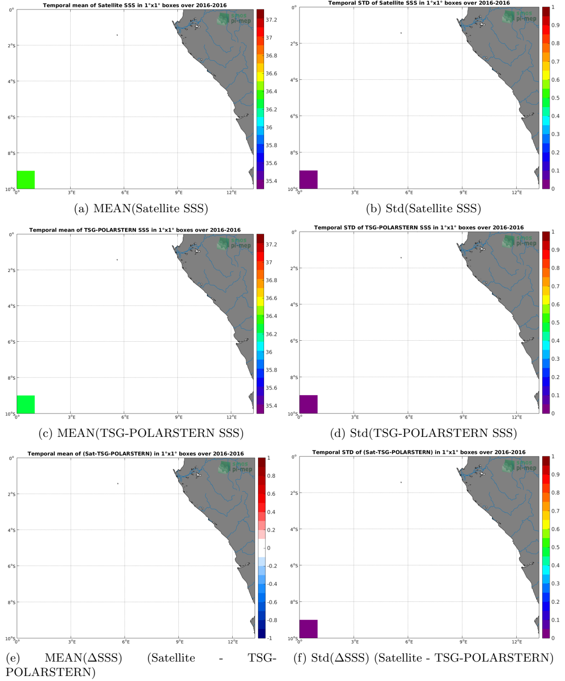
Figure 6: Temporal mean (left) and Std (right) of SSS from SMAP-L3-RSS-V3-MONTHLY-0.25DEG-40KM (top), TSG-POLARSTERN (middle), and of \Delta SSS (Satellite - TSG-POLARSTERN). Only match-up pairs are used to generate these maps.
