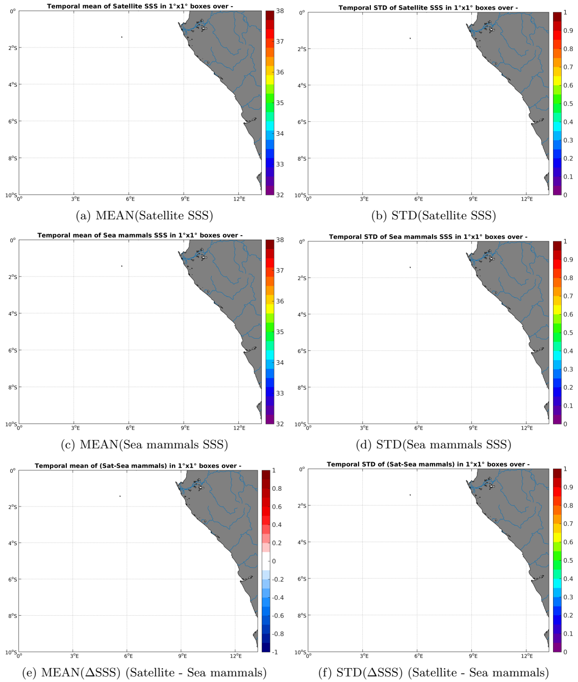
Figure 6: Temporal mean (left) and STD (right) of SSS from SMAP-L3-RSS-V2-8DAY-RUNNING-40KM (top), Sea mammals (middle), and of \Delta SSS (Satellite - Sea mammals). Only match-up pairs are used to generate these maps.
